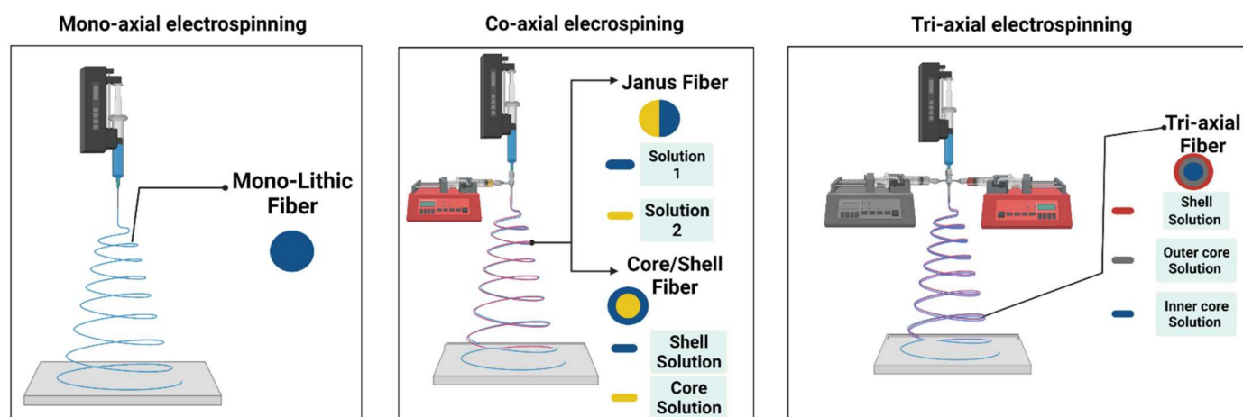
Figure 1. Techniques for nanofiber production.
