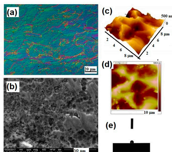
Figure 2. Surface properties of Ti mesh for cranioplasty evidenced by different microscopic techniques: (a) light microscopy image in phase contrast, longitudinal section, 500×, Kroll reagent; (b) Scanning Electron Microscopy 2000×; (c,d) 3D and 2D Atomic Force Microscopy images; (e) contact angle investigation on the surface of the titanium mesh.
