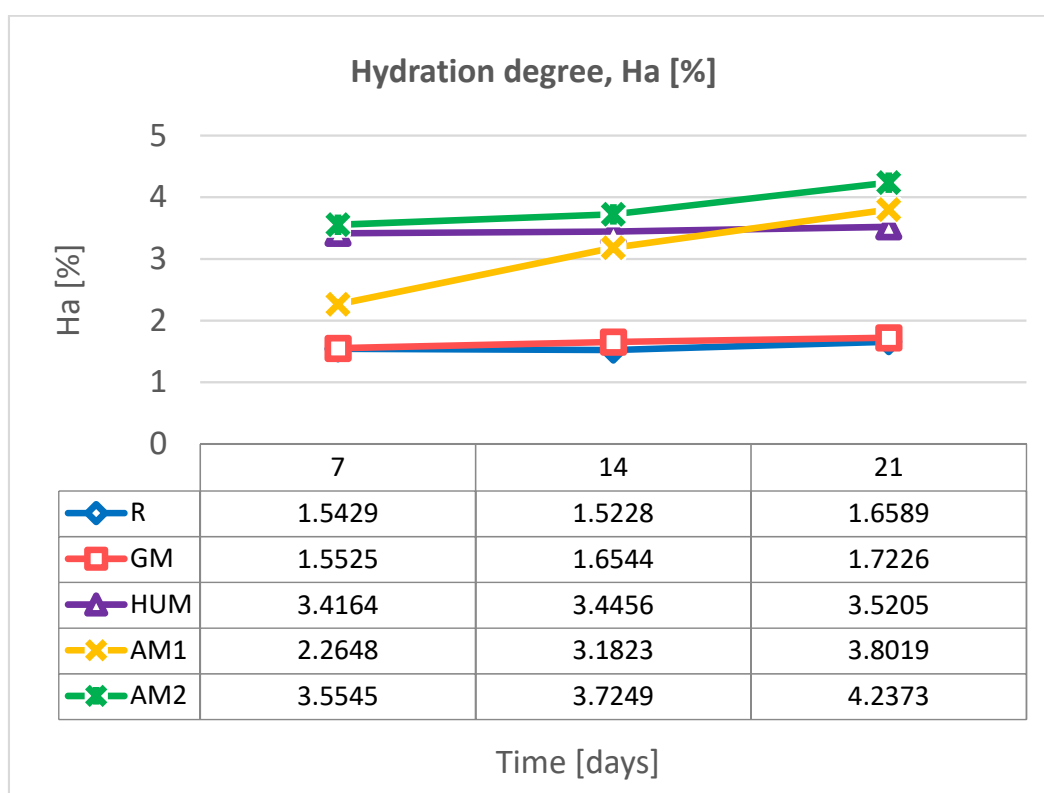
Figure 4. Variation of hydration degree over a period of 21 days in distilled water, at 37 °C, for experimental bone cements samples.
