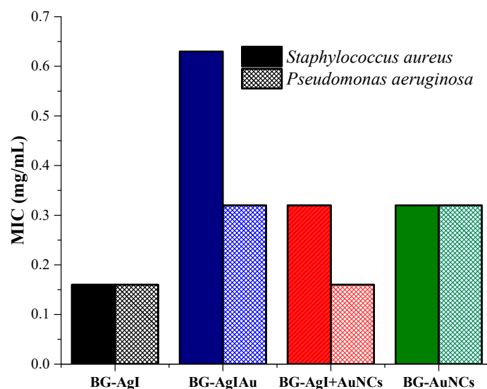
Figure 10. Minimal inhibitory concentration (MIC) of S. aureus and P. aeruginosa using BG composites. Gentamycin was used as a positive control obtaining MIC of 0.0024 \text{ mg} \cdot \text{mL}^{-1} for both bacteria.
