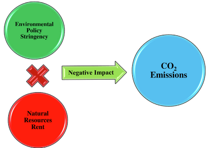
Fig. 11. Impact of interaction term of EPS and NRR on CO 2 emissions.
