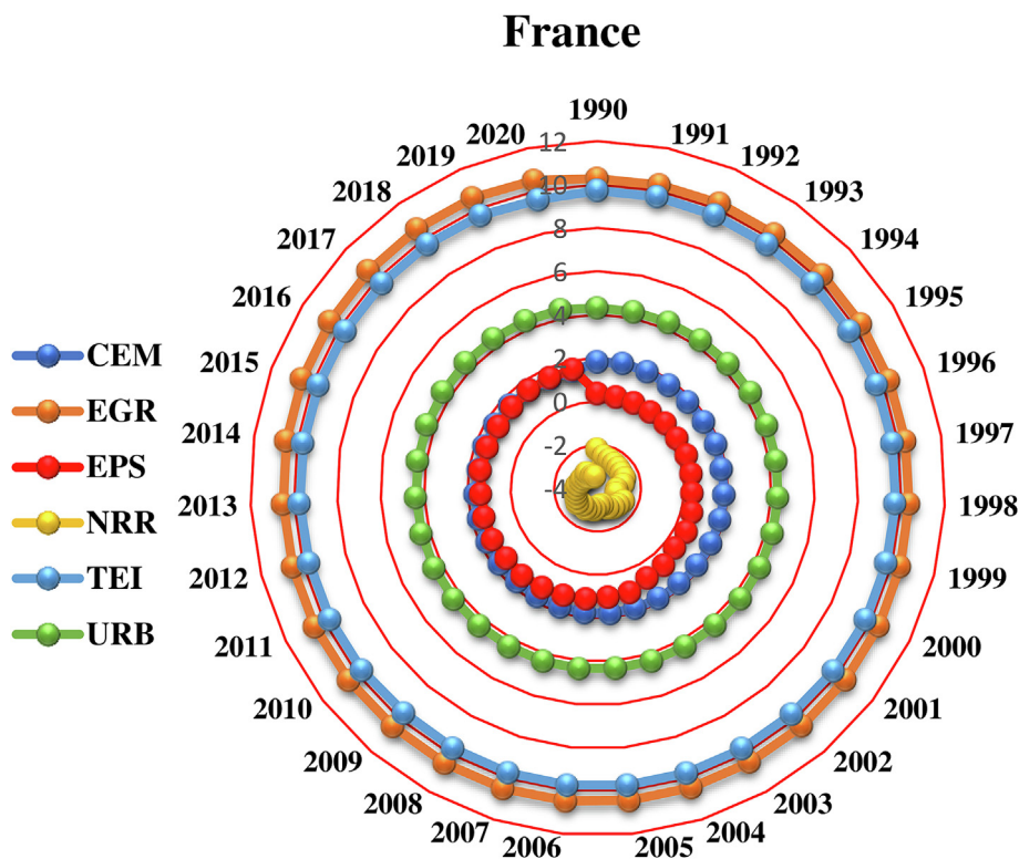
Fig. 4. Data trend of France.
