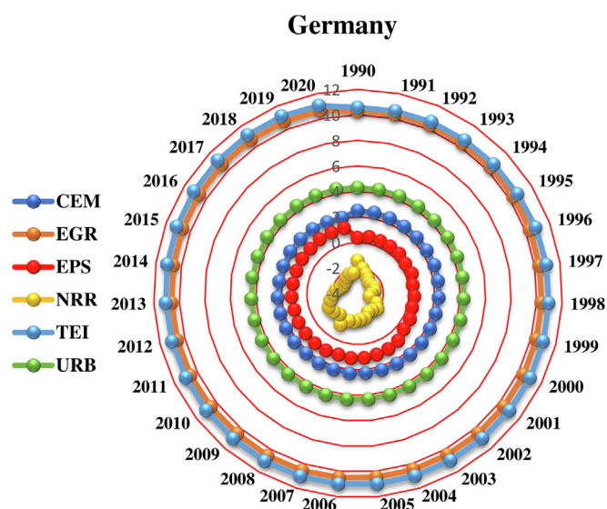
Fig. 5. Data trend of Germany.
