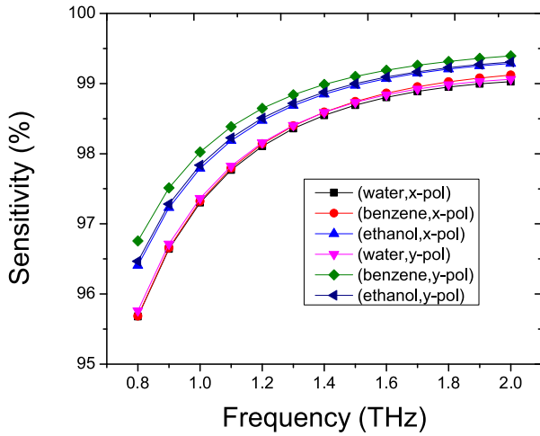
(b) S = 20 \mu\text{m}
