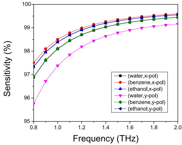
(a) S = 10 \mu\text{m}
