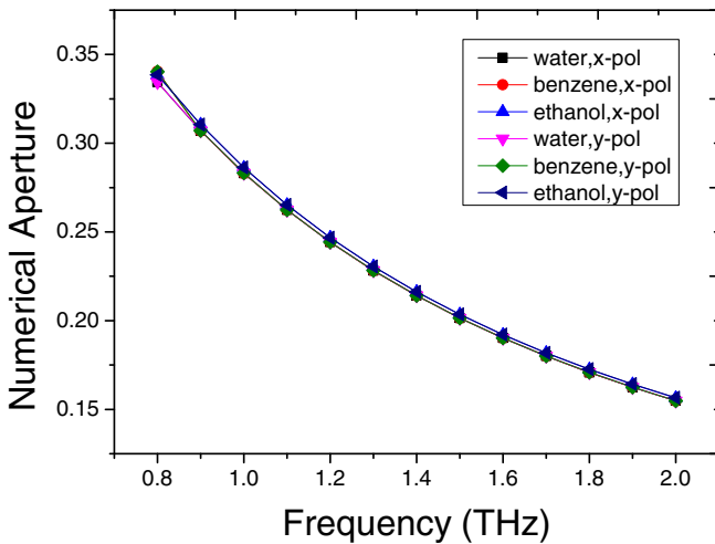
Fig. 13. Numerical aperture for Water, Benzene and Ethanol as a function of frequency.
