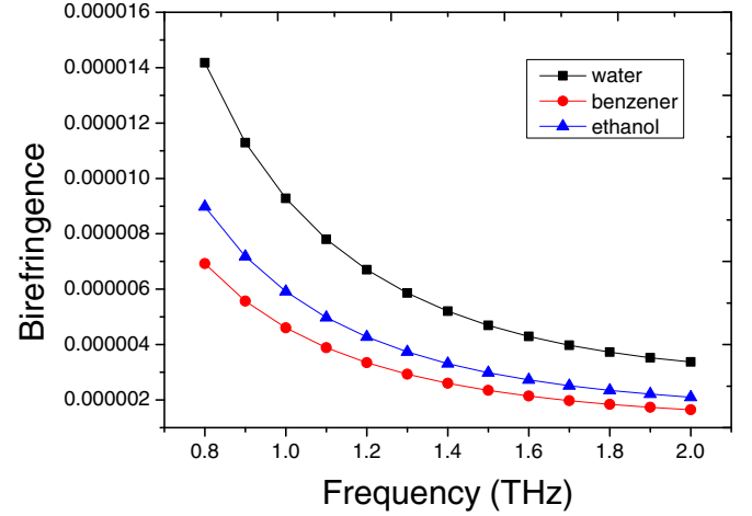
Fig. 9. The relation between birefringence and frequency for Ethanol, Water, and Benzene.
