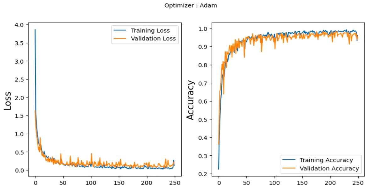
Fig. 4. Accuracy diagram for image size [64x64] and patch 12.
