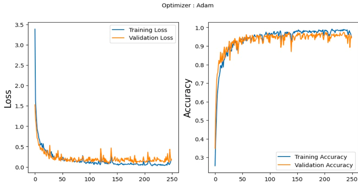
Fig. 5. Accuracy diagram for image size [56×56] and patch 7.
