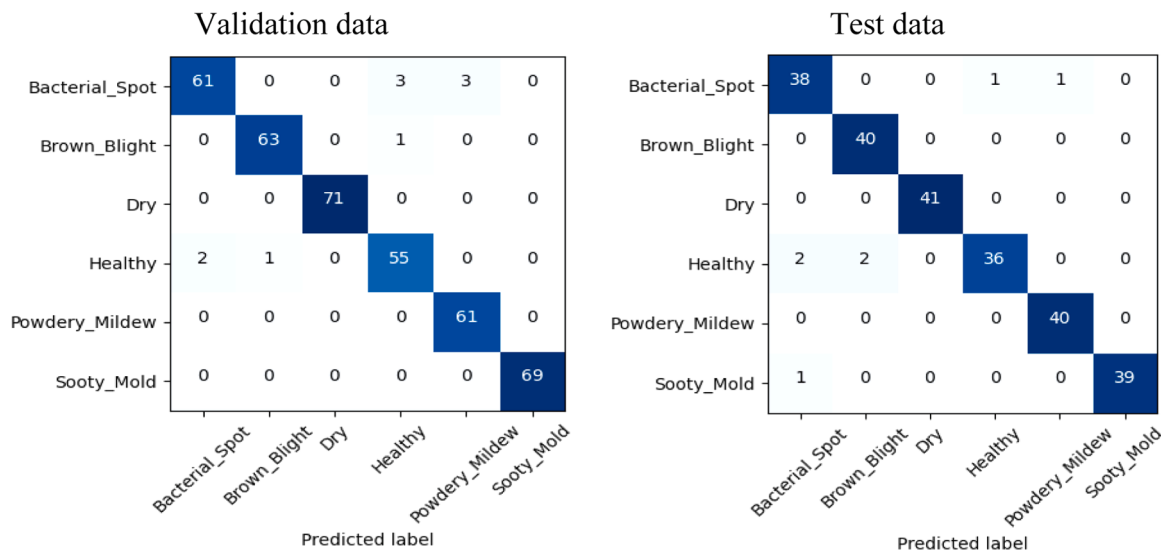
Fig. 3. Confusion matrices for image size [56x56] and patch 7.
