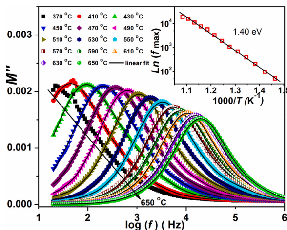
Fig. 6. Modulus plots at various temperatures of NSBT samples. Gaussian fitting solid lines are shown with solid lines, Relaxation frequency vs temperature curve of NSBT compound is shown in the inset.
