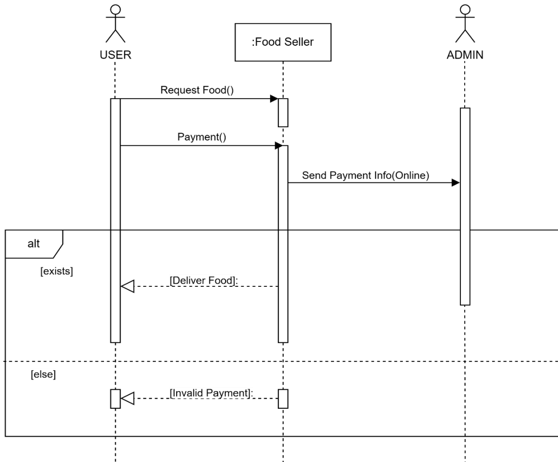
Figure 3.5 Sequence Diagram
