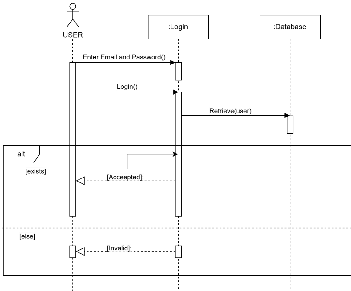
Figure 3.4 Sequence Diagram
