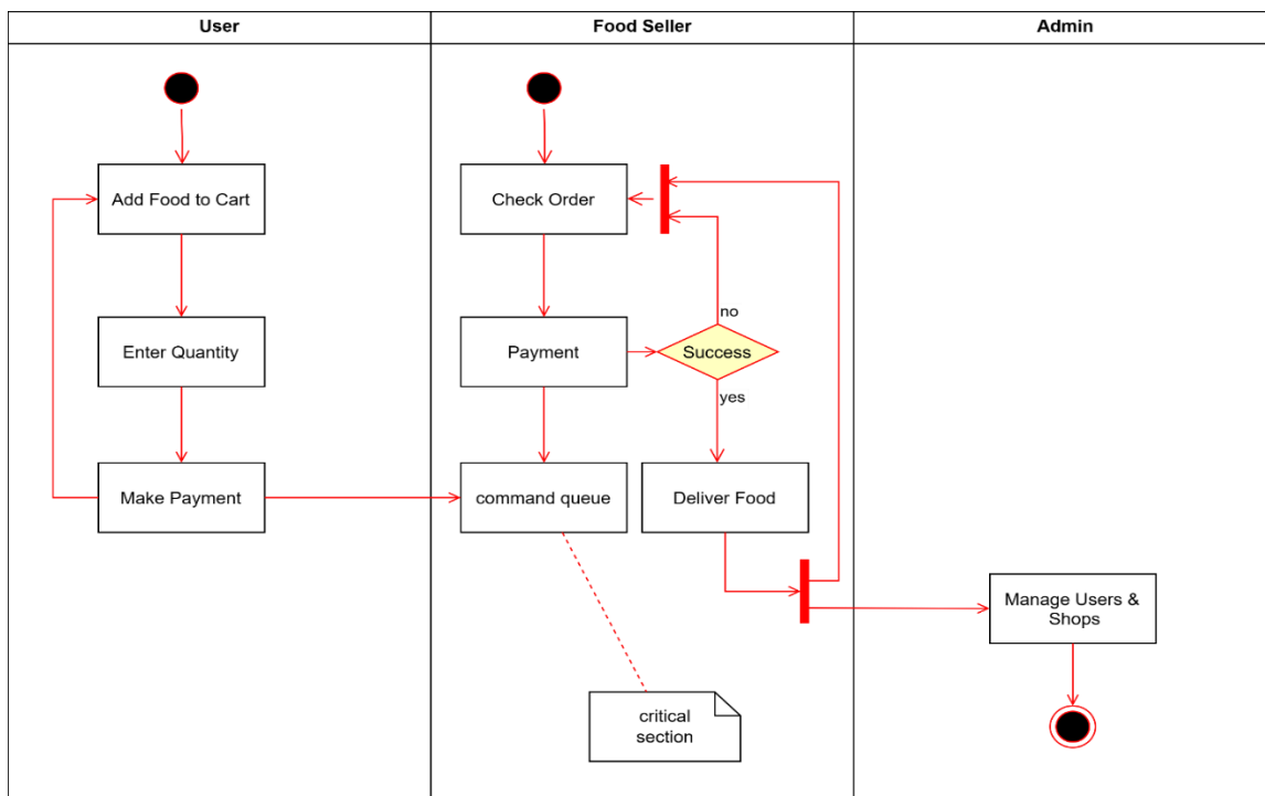
Figure 3.3 Activity Diagram
