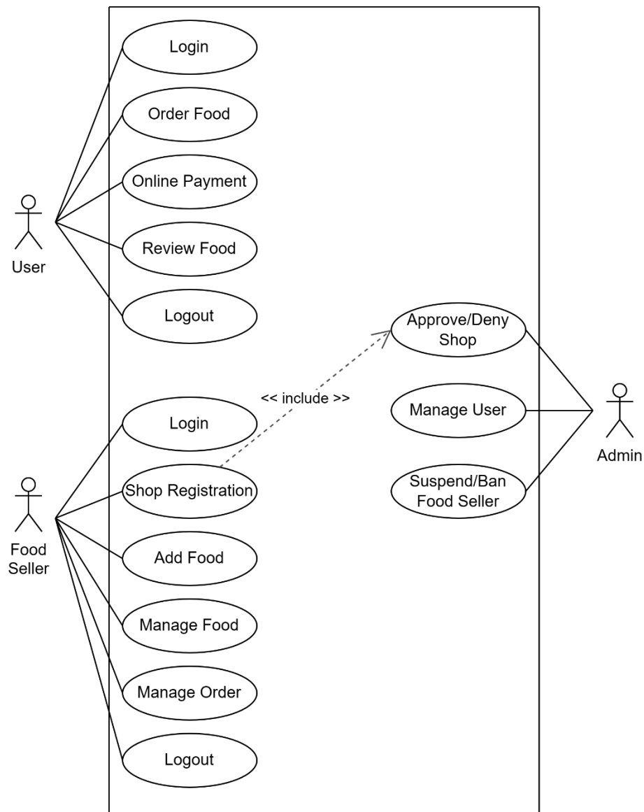
Figure 3.2: Use case diagram.
