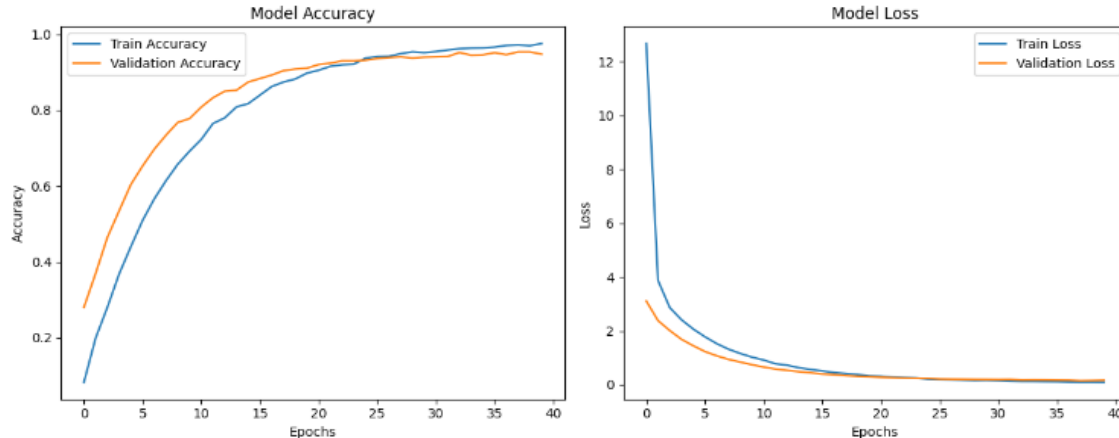
Figure 4.3.2: Training & Validation Accuracy and Loss of VGG16 over the epochs
