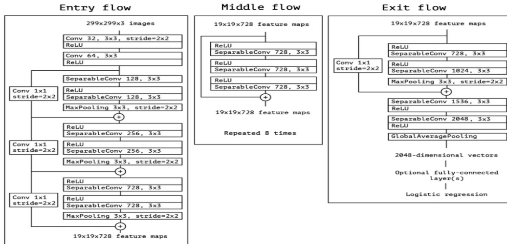
Figure 3.2.5: Xception Architecture [34]
