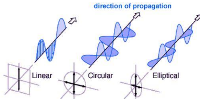
Figure 3.2: Antenna Polarization
