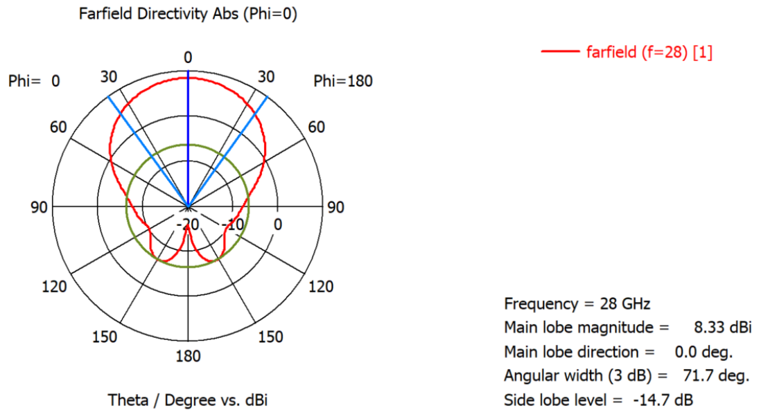
Figure 4.8: Radiation Pattern at 28GHz
