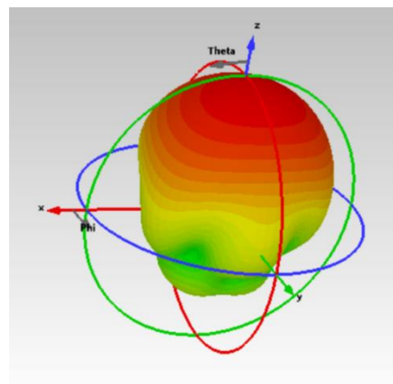
Figure 3.6: Far-field of a MPA
