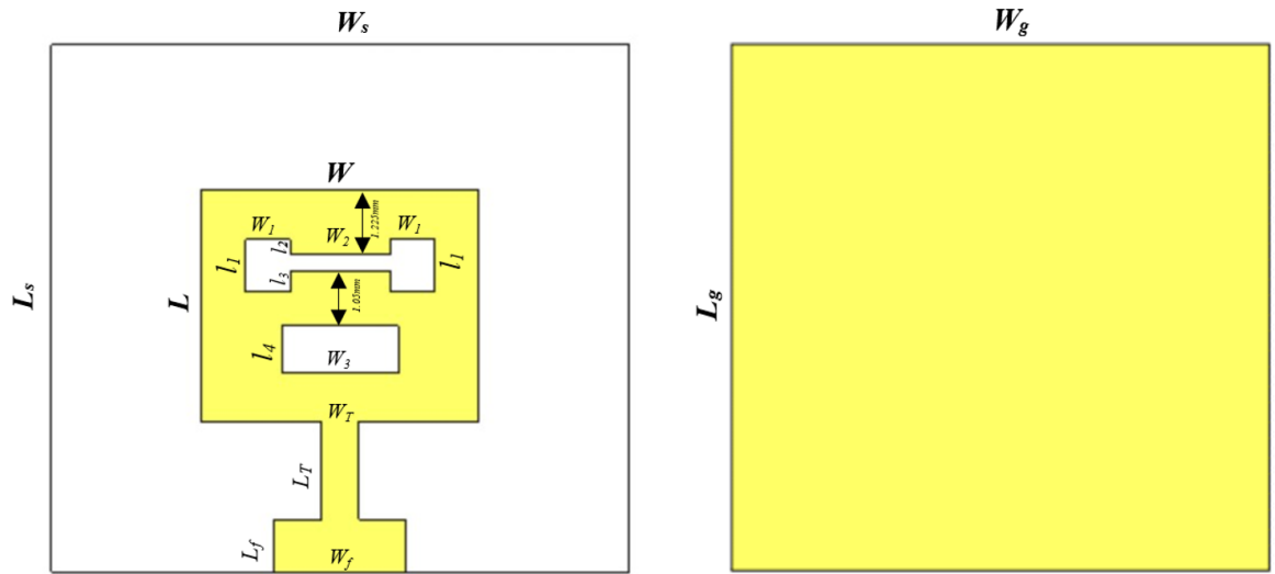
Figure 3.8: Top and bottom view of the proposed antenna
