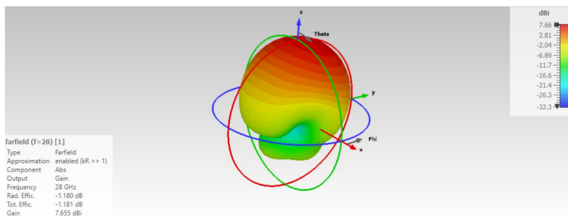
Figure 4.6: Antenna Gain at 28GHz
