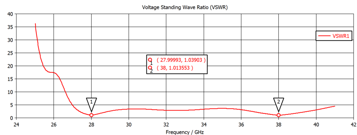
Figure 4.3: VSWR Graph
