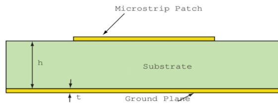
Figure 3.9: Side view of the proposed antenna
