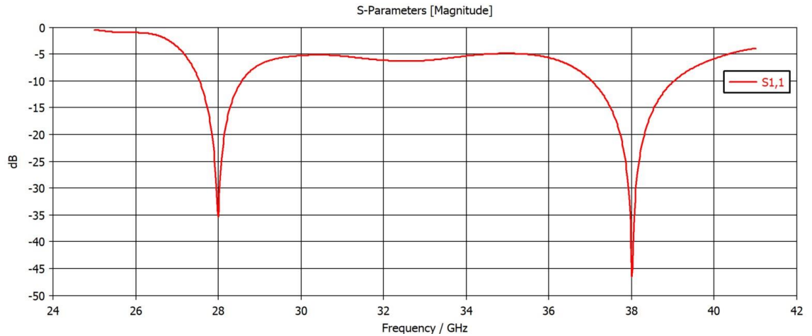
Figure 4.1: S_{11} Parameter for the proposed dual band antenna
