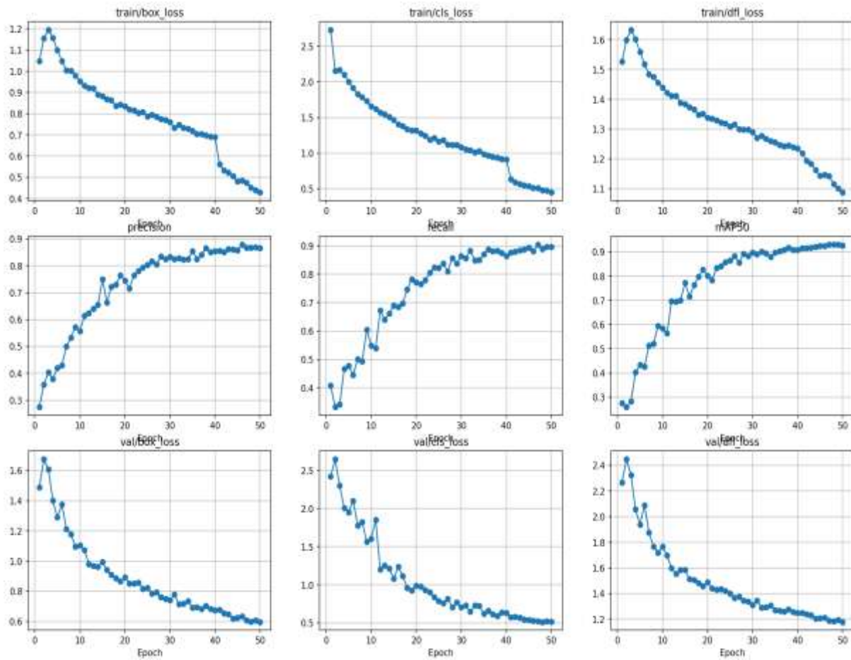
Figure 4.3: Plots of loss Curve for YOLOv11
