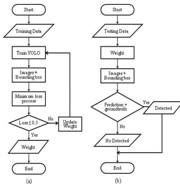
Figure 3.16: Data Flow Diagram for YOLO
