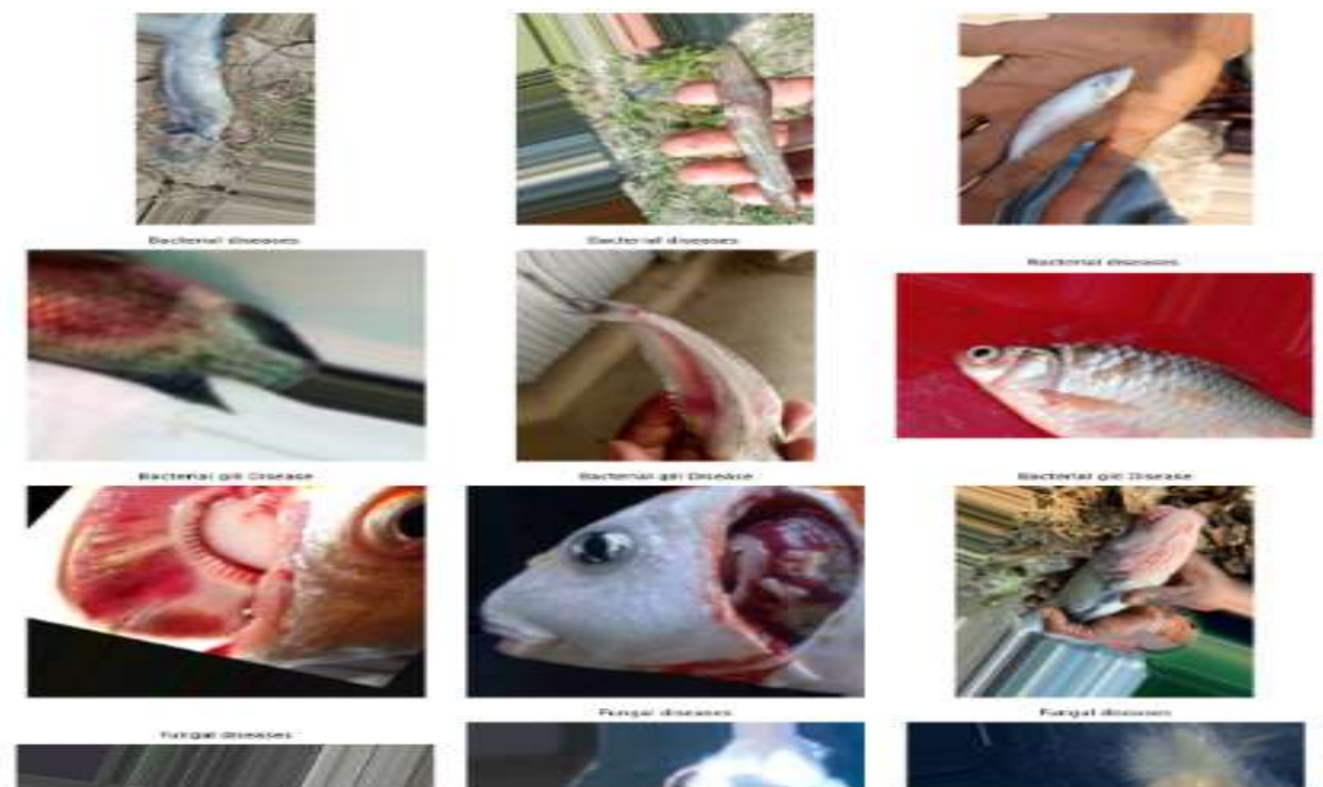
Figure 3.1: Raw Dataset
