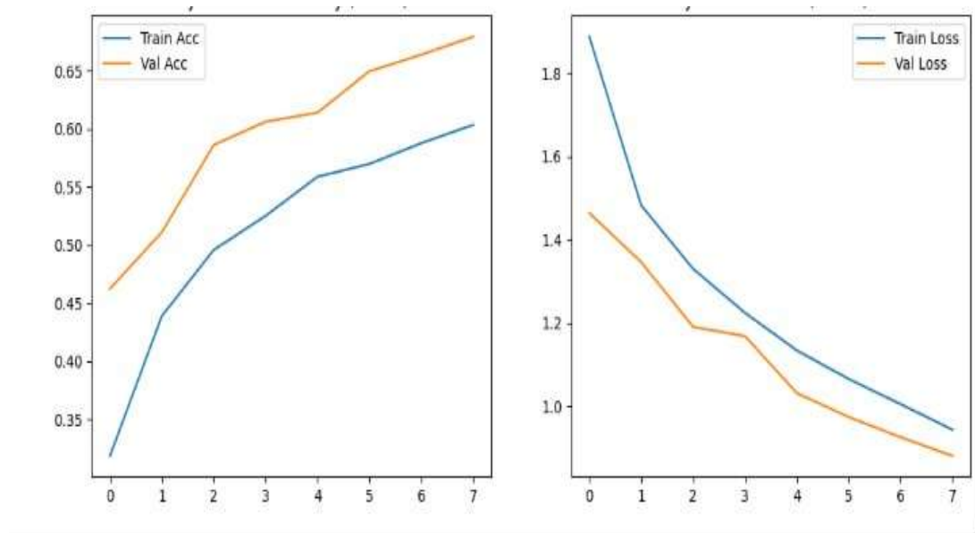
Figure 4.5: Plots of Accuracy and loss for Hybrid CNN
