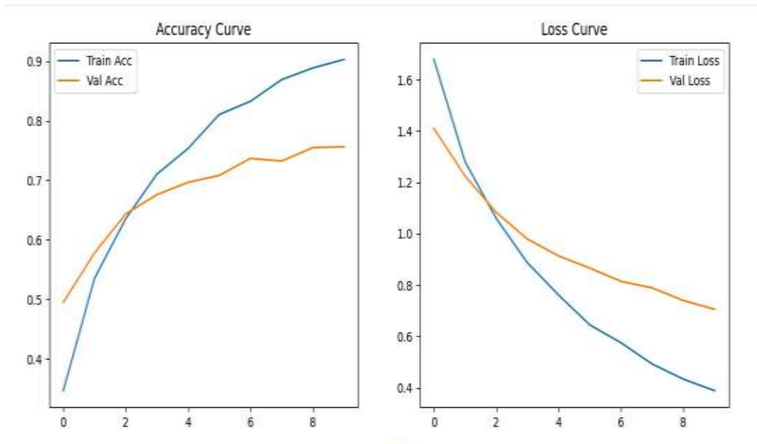
Figure 4.4: Plots of Accuracy and loss for VGG16
