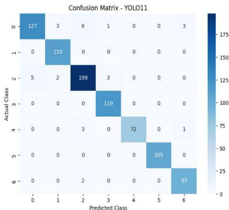
Figure 4.6: Confusion matrix for YOLOv11
