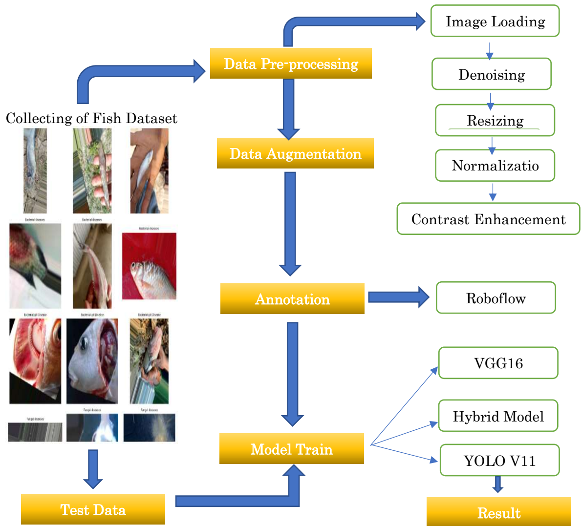
Figure 3.13: Proposed Model Diagram
