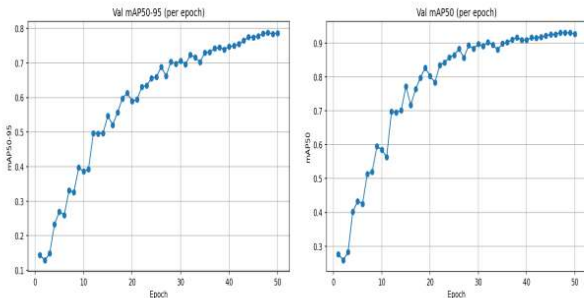
Figure 4.2: Plots of mAP50 and mAP50-95 Curve for YOLOv11
