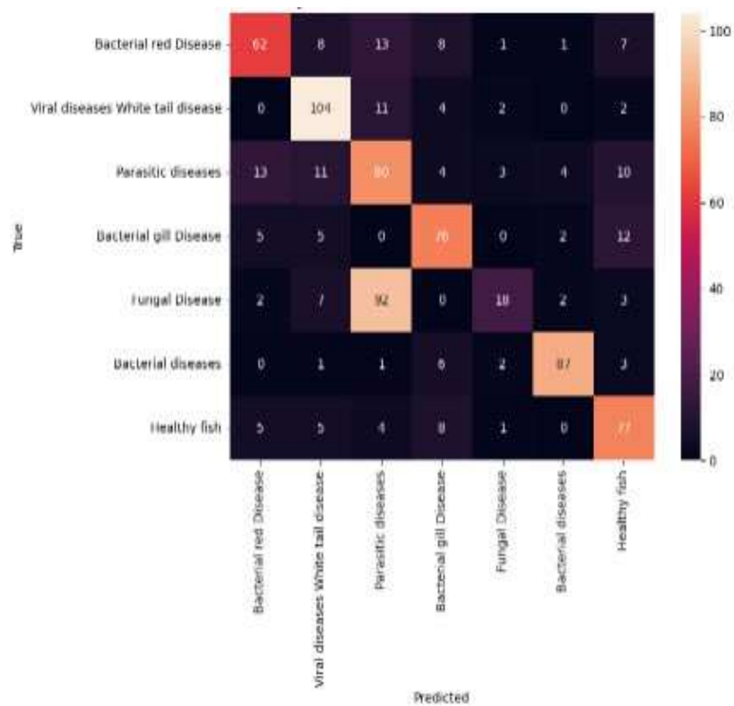
Figure 4.8: Confusion Matrix for Hybrid CNN
