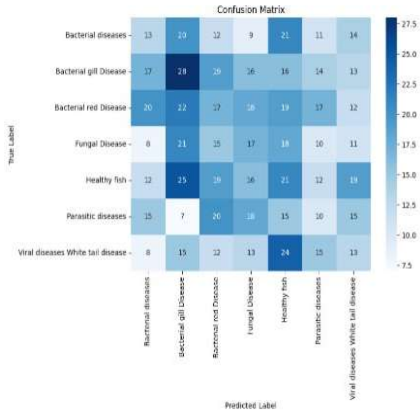
Figure 4.7: Confusion matrix for VGG16
