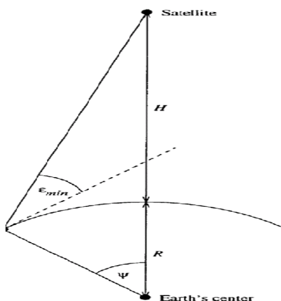
FIGURE A5-1 Geometric satellite coverage scheme
