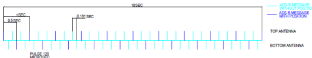
FIGURE A6-7 Time representation of automatic dependent surveillance - broadcast pulse frames
