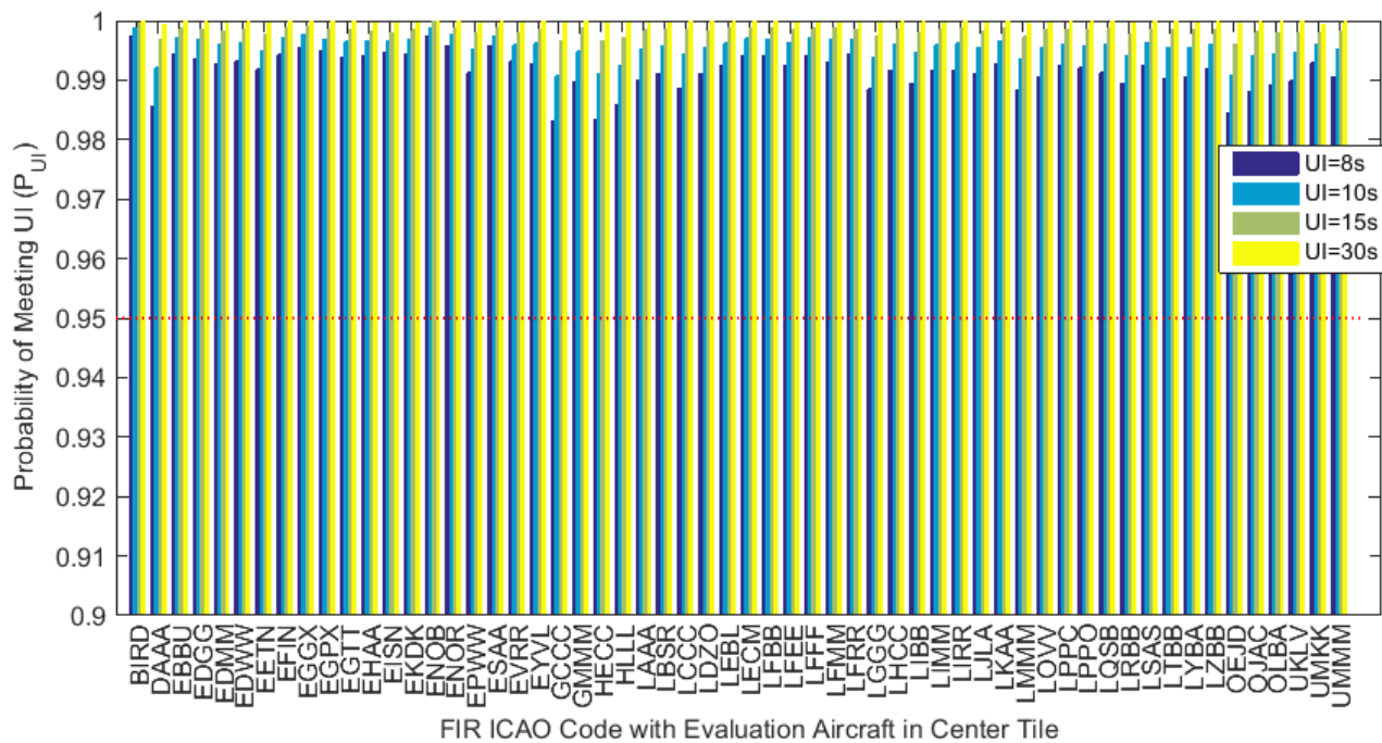
Automatic dependent surveillance – broadcast update interval results for 125 W equipped aircraft
