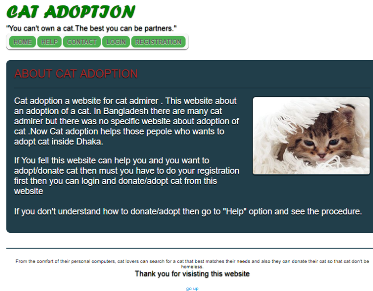
Figure6.1 Home Page
