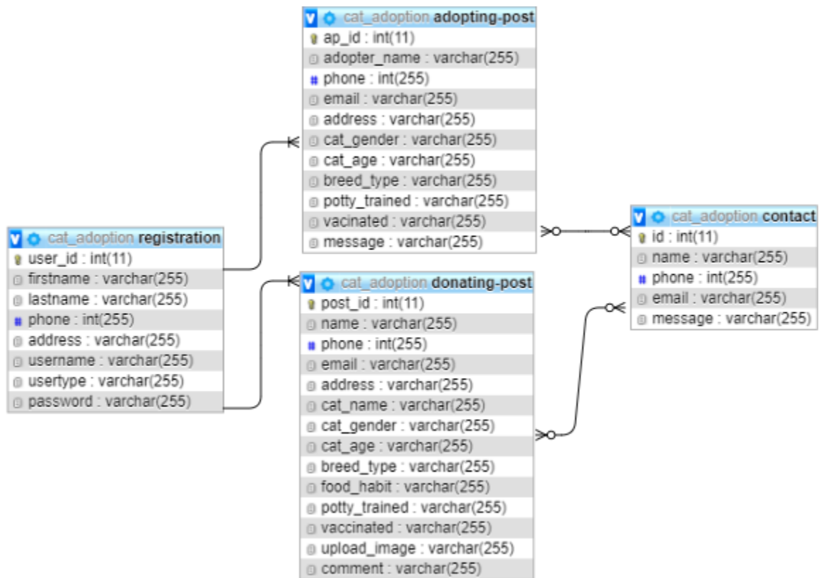
Figure4.4 Database Diagram
