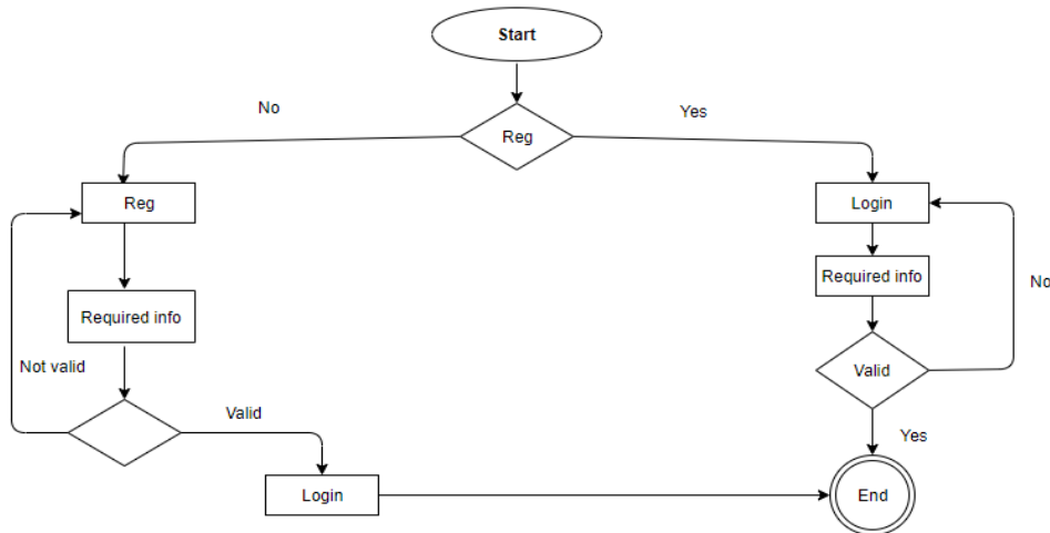
Figure 3.3.1Registration Activity
