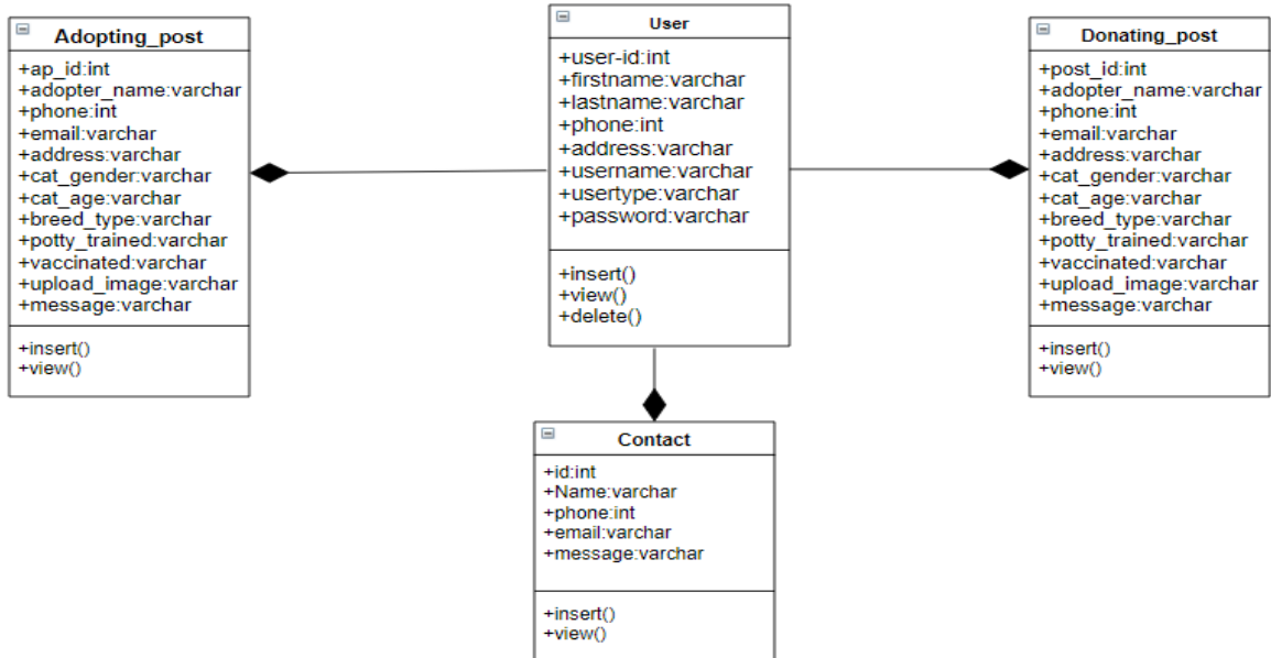
Figure4.3Class diagram
