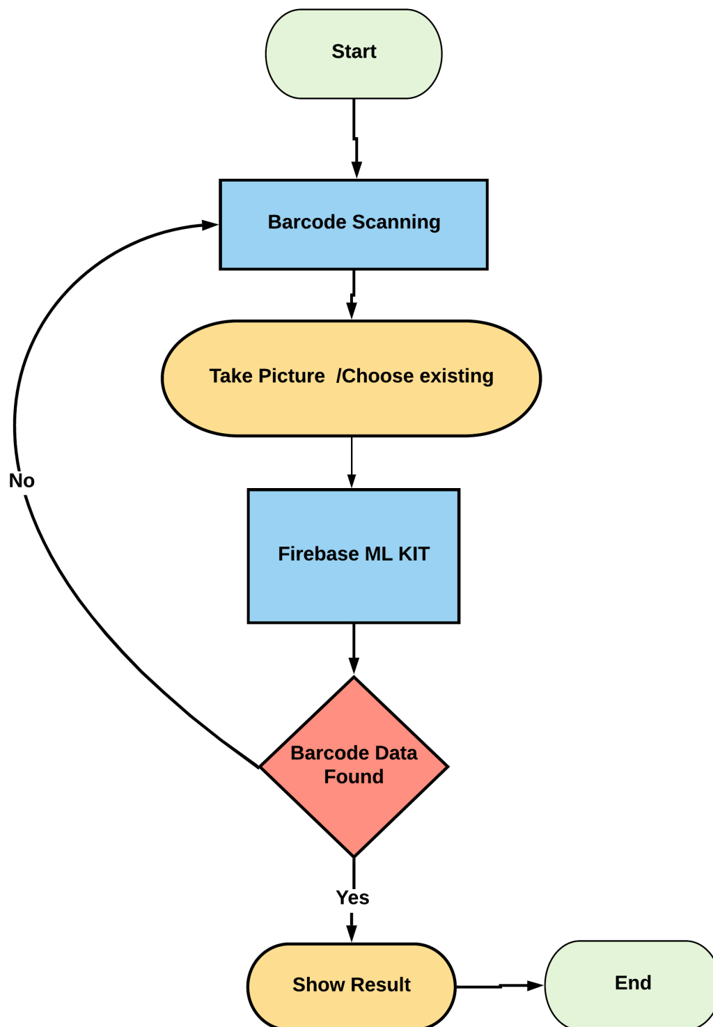
Figure 3.4.4: Barcode Detection Case Diagram.
