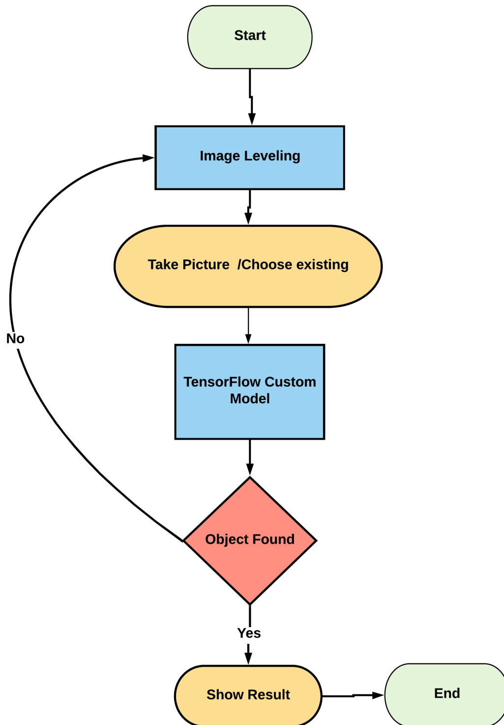
Figure 3.4.6: Image Use Case Diagram
