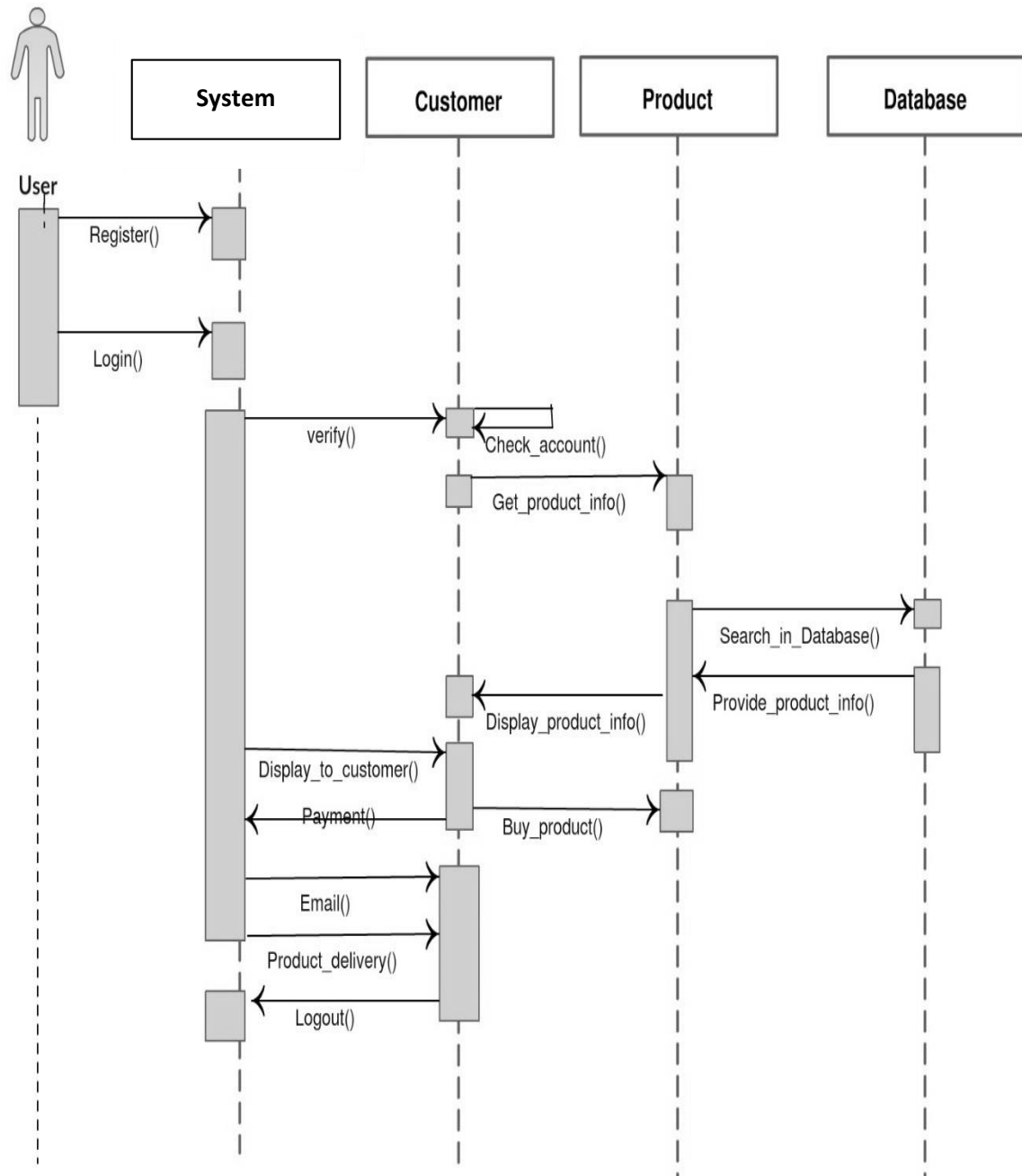
Figure 4.5: Sequence Diagram of Easybazar
