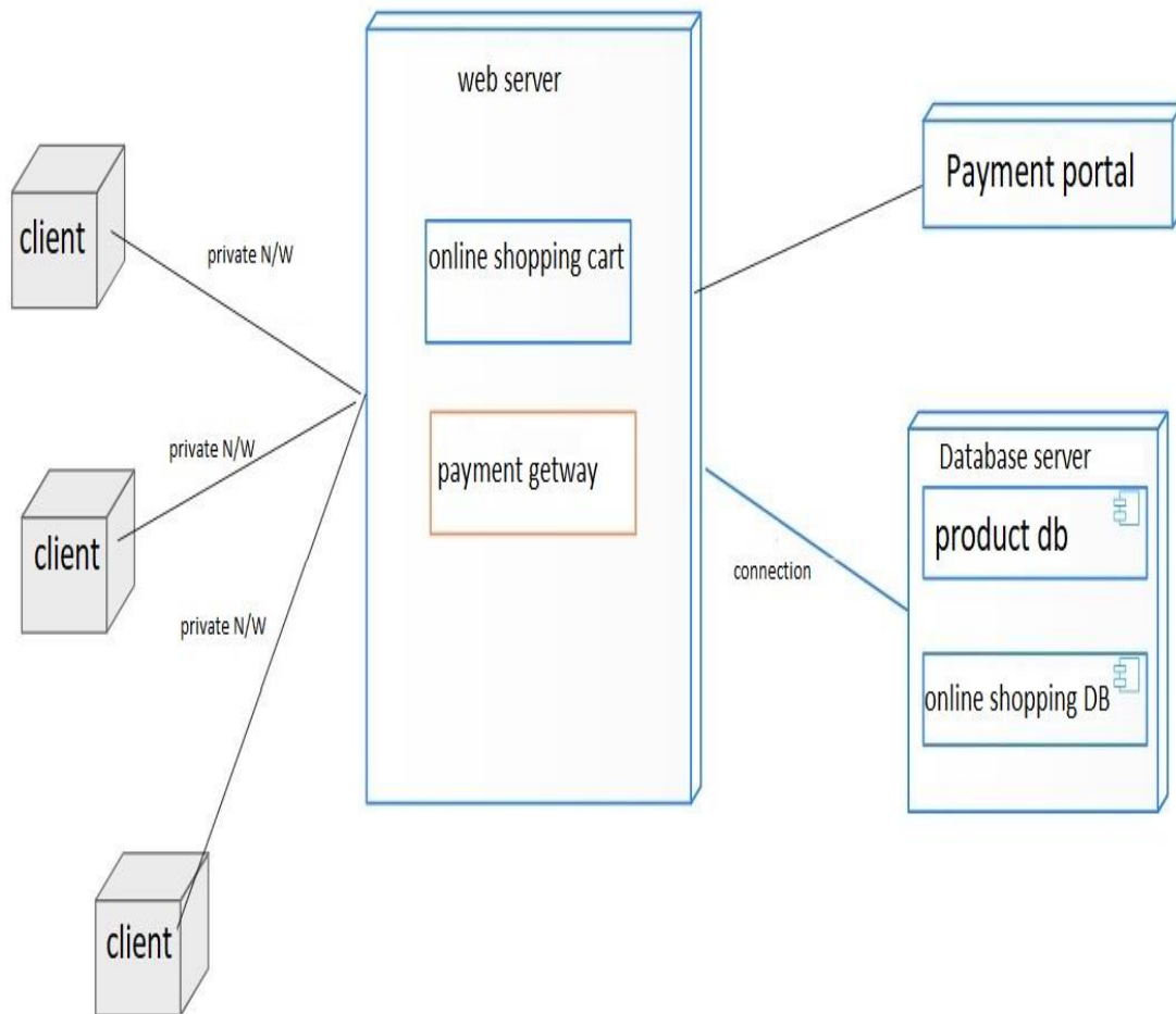
Figure 4.7: Deployment Diagram of Easybazar
