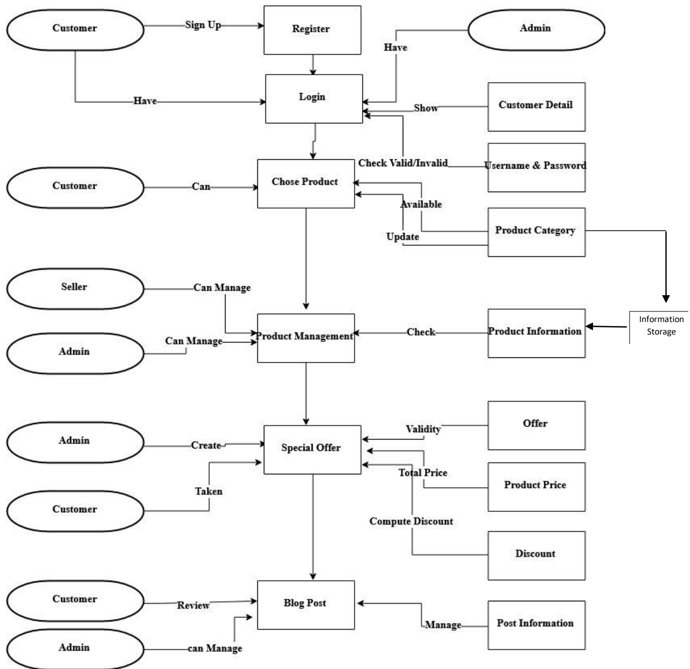
Figure 4.3: DFD 1 Level Diagram of Easybazar
