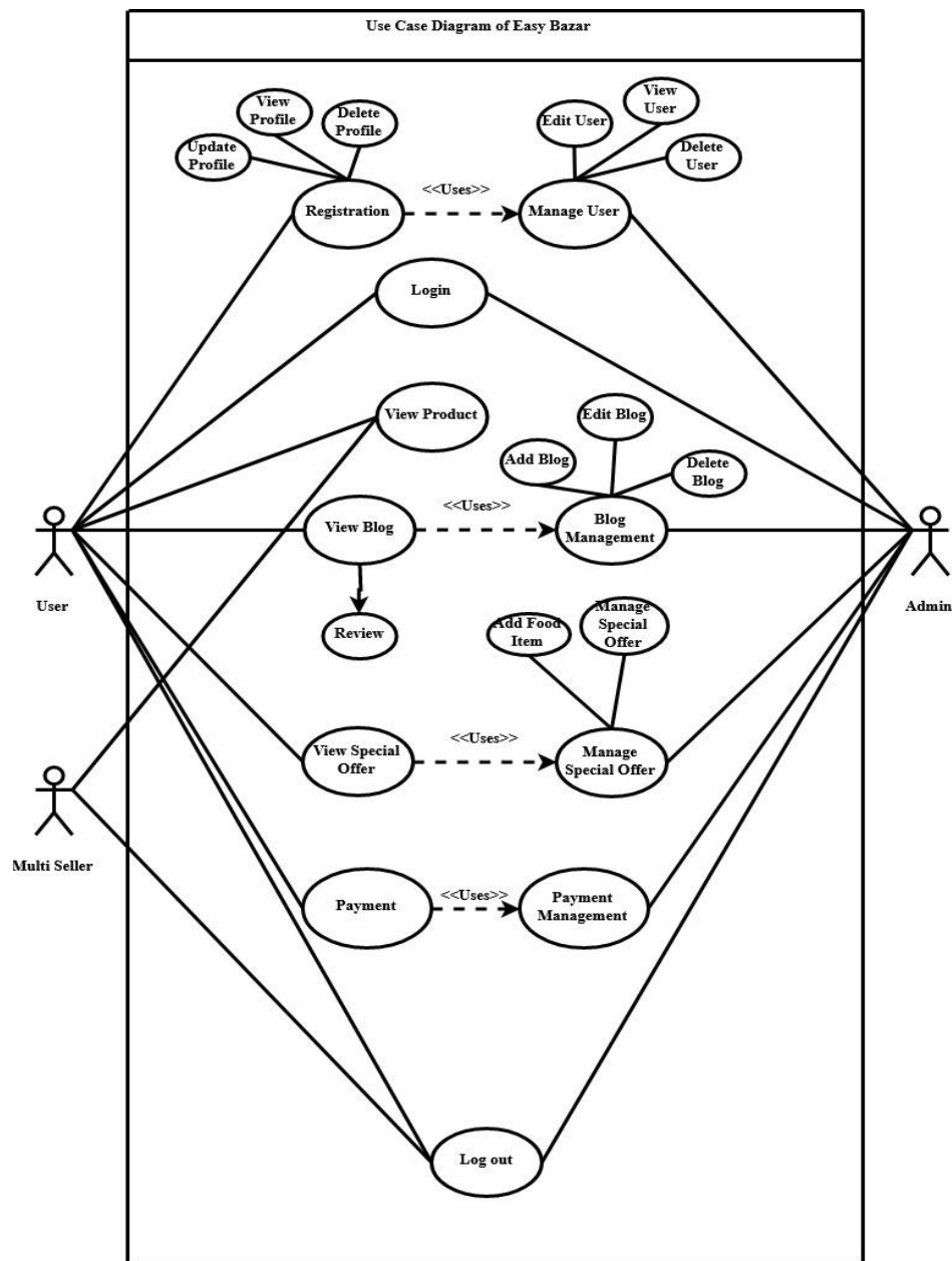
Figure 4.1: Use Case Diagram of Easybazar
