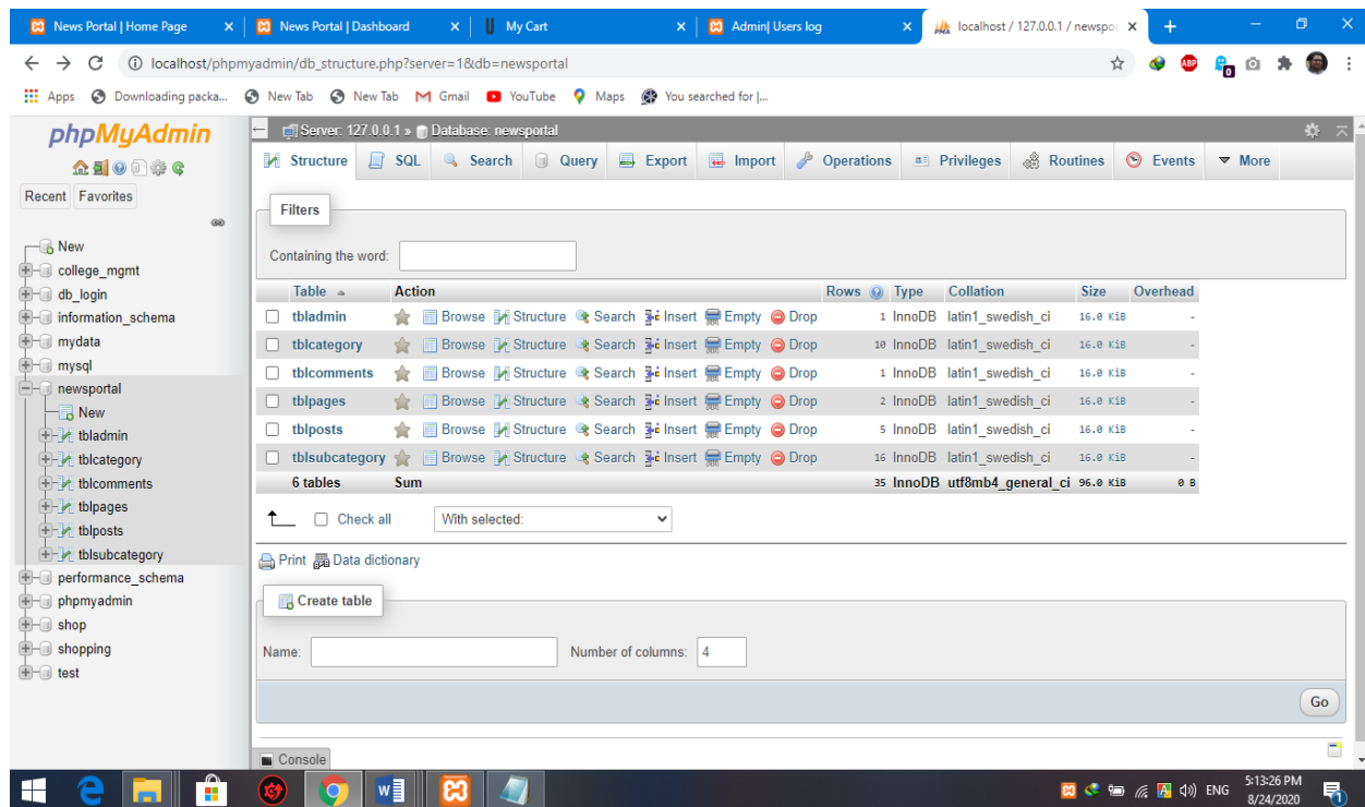
Figure 3. 3.9:Database Tables
