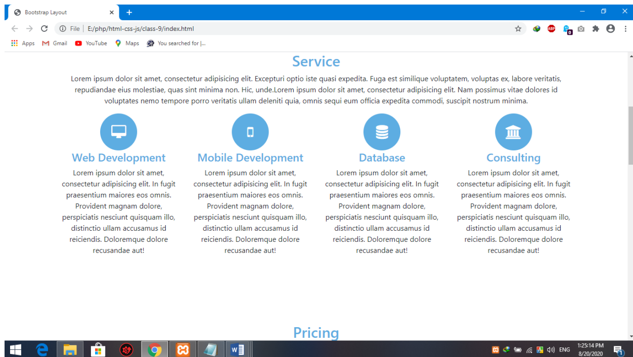
Figure 3.3.2: First/Front Page
