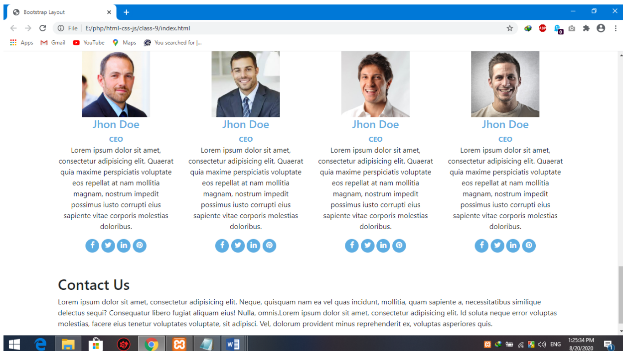
Figure 3.3.4: First/Front Page
