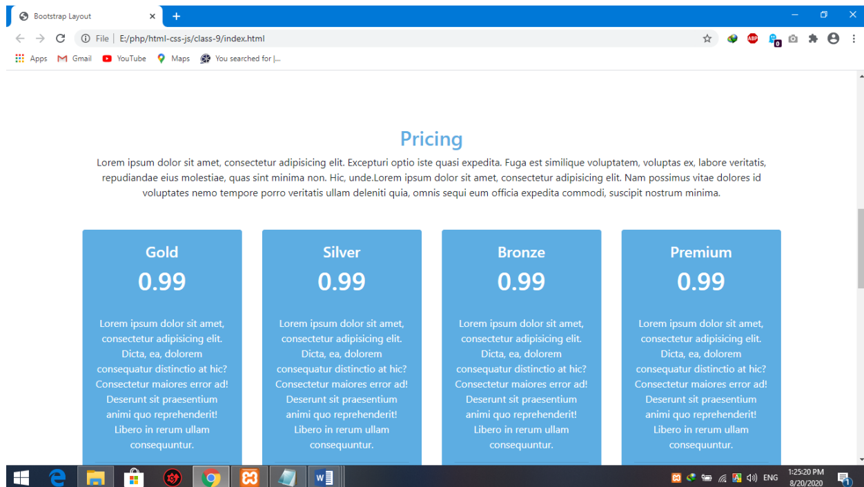
Figure 3.3.3: First/Front Page
