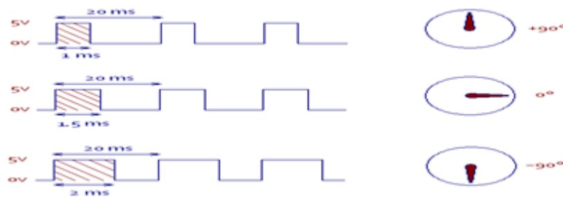
Figure: 2.11: Variable pulse width control servo position.
