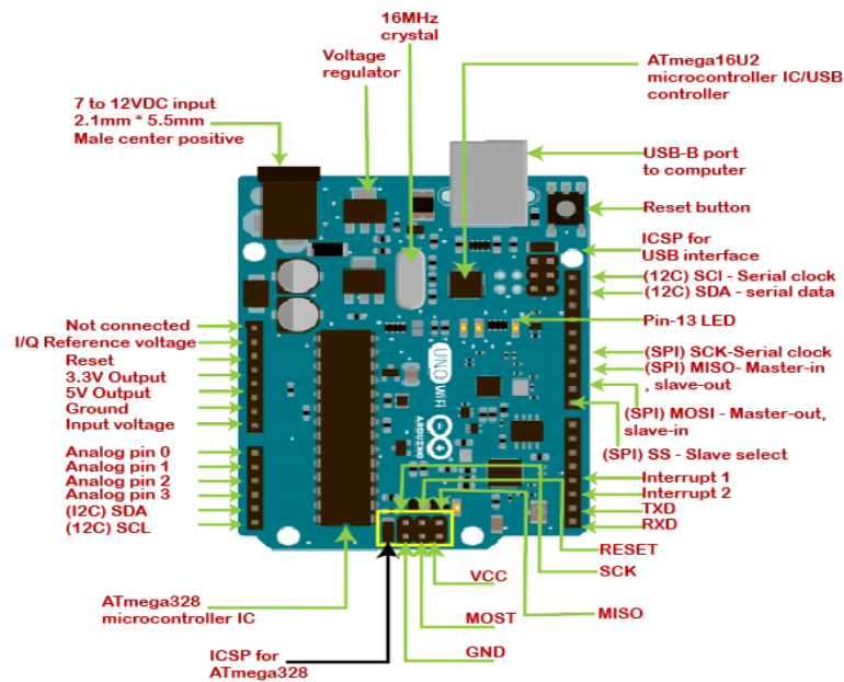
Figure:3.3 Arduino Uno Pinout.
