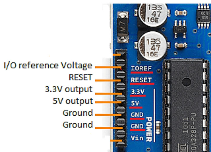
Figure:3.4.4: Others pins.
