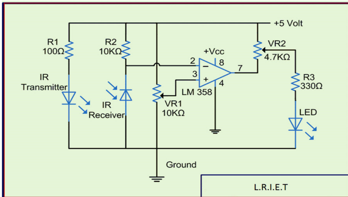
Figure: 2.15.1: IR Sensors Circuit.
