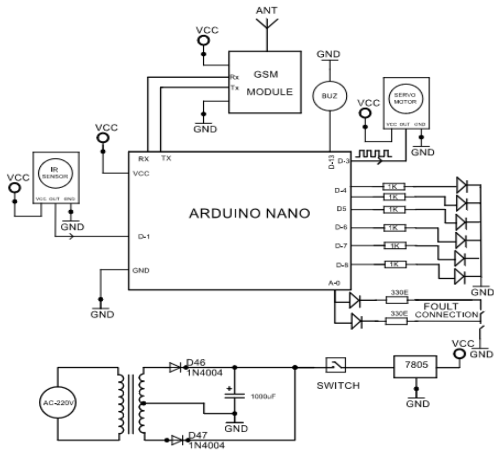
Figure: 2.2 : Schematic Diagram.
