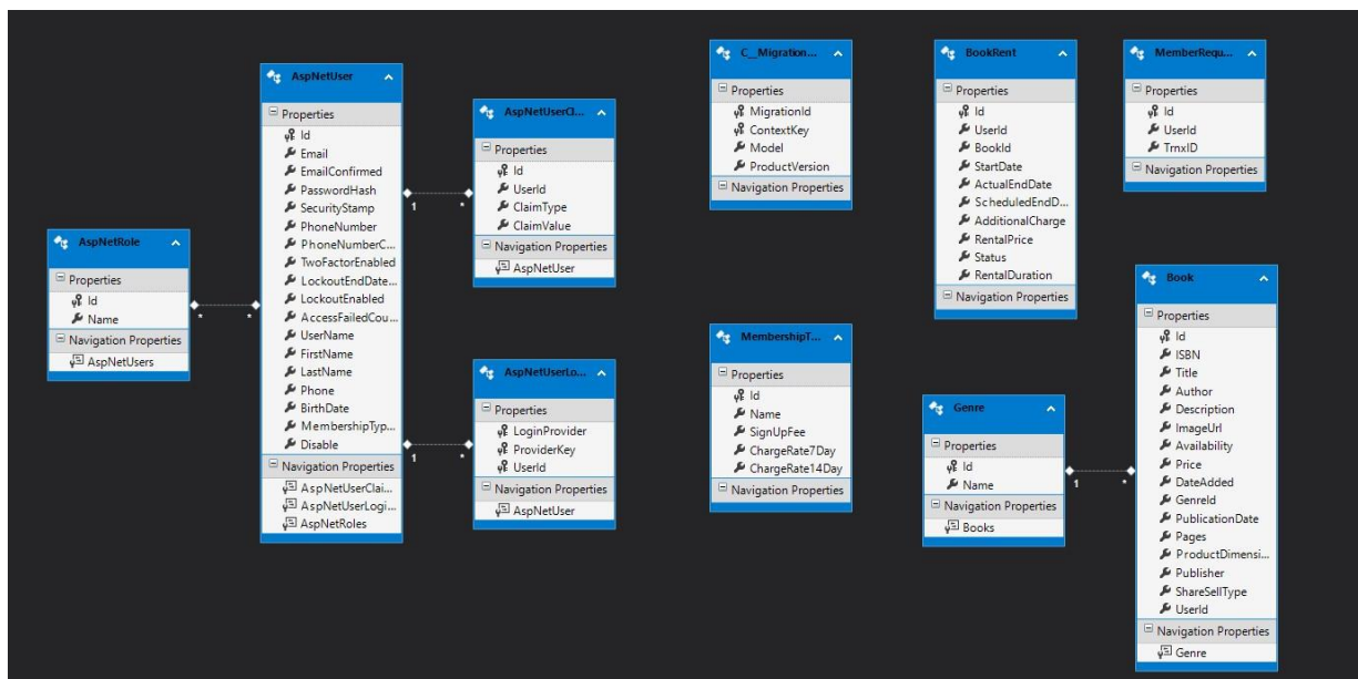
Figure 5.1.1: Implementation of database
