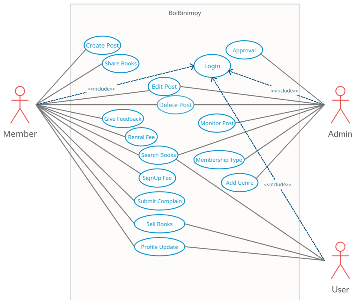
Figure 3.3.1: Use Case Modeling and Description
