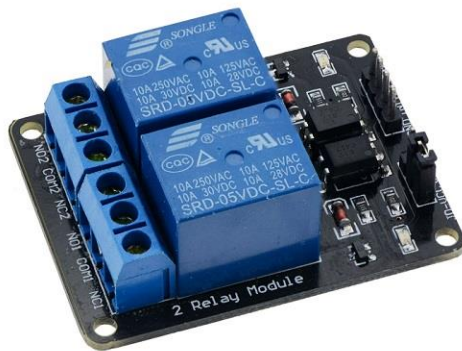
Figure 3.3.7: 2 Channel 5V relay Module. [17]
