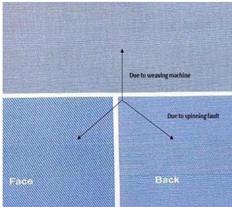
Figure 20: weft bar.
