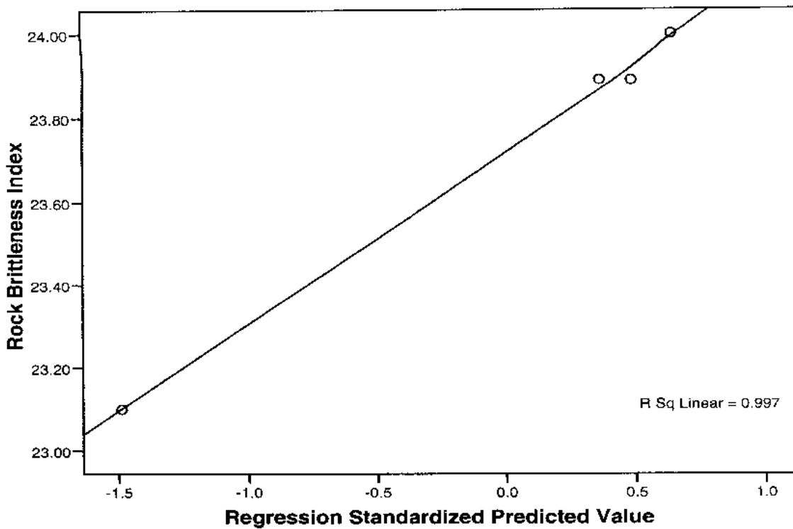
Figure 4 : A graph of rock brittleness index against regression standardized predicted value
