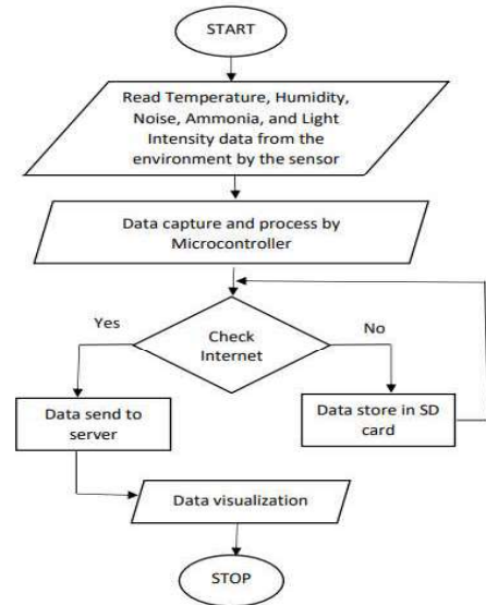
Figure 2.1: Flowchart of IoT Device
