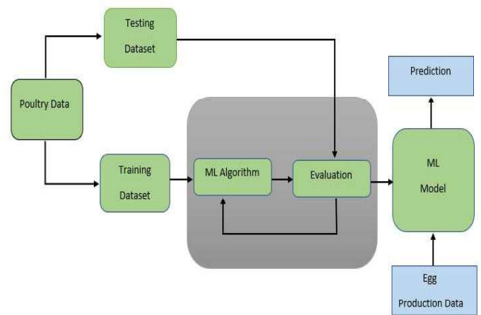
Figure 6: ML Model
