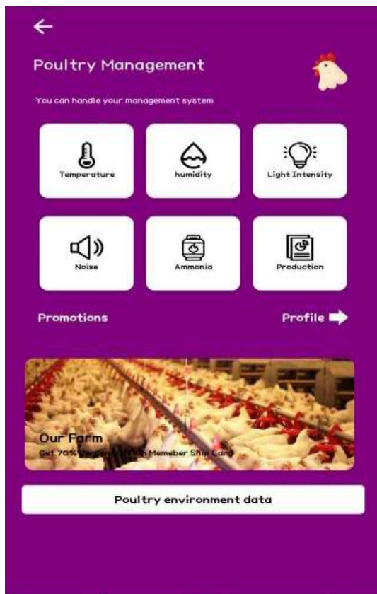
Figure 5: Android Apps
