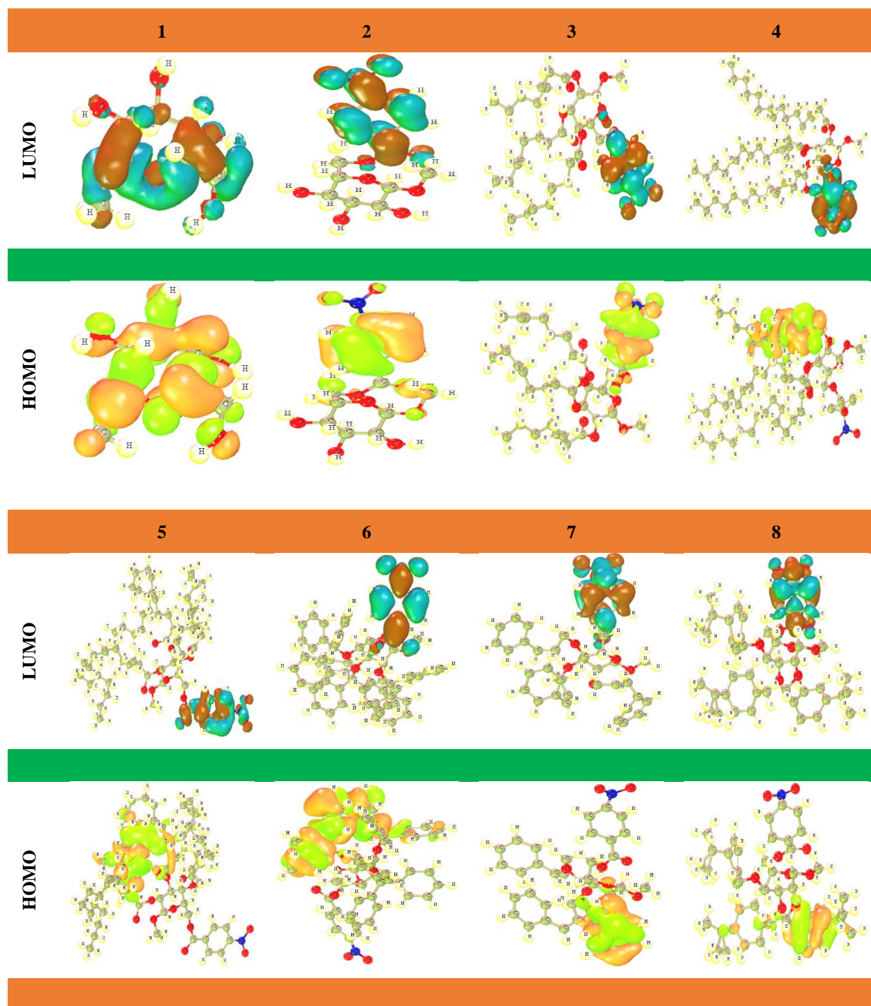
Figure S3. HOMO and LUMO diagram.
