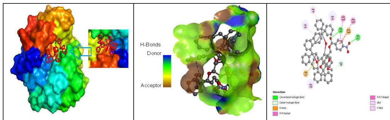
Figure 8. Molecular docking poses of R. miehei (4WTP).
