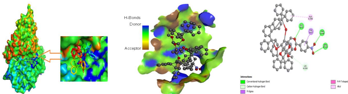
Figure 6. Molecular docking poses of P. aeruginosa .
