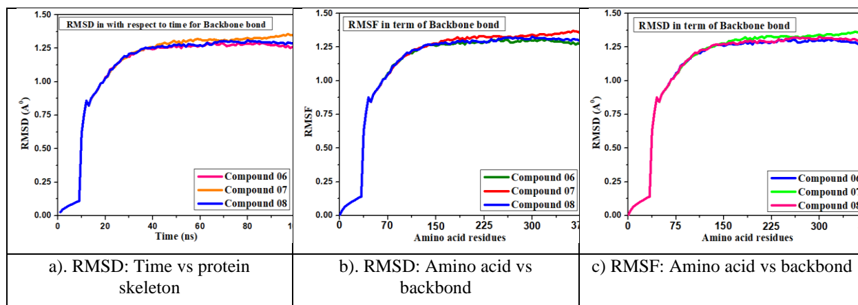
Figure S6. Various pictures of RMSD and RMSF for protein C. Auris .
