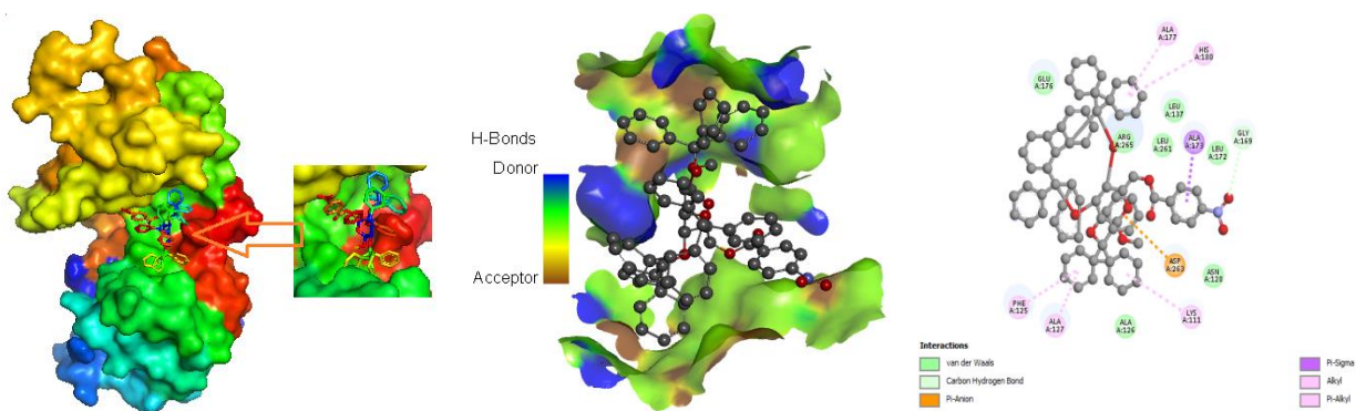
Figure 7. Molecular docking poses of E. coli (1DIH).
