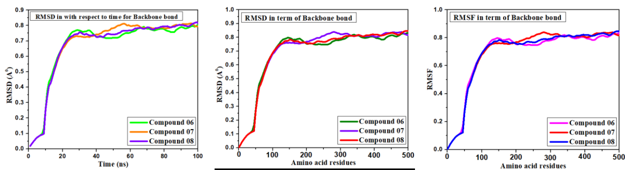
a). RMSD: Time vs protein skeleton b). RMSD: Amino acid vs backbone c) RMSF: Amino acid vs backbone
