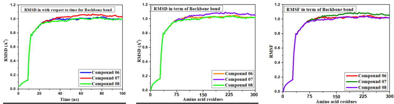
a). RMSD: Time vs protein skeleton b). RMSD: Amino acid vs backbone c) RMSF: Amino acid vs backbone
