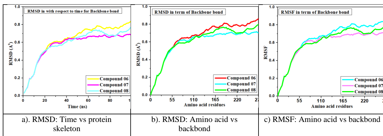
Figure S5. Various pictures of RMSD and RMSF for protein R. miehei .
