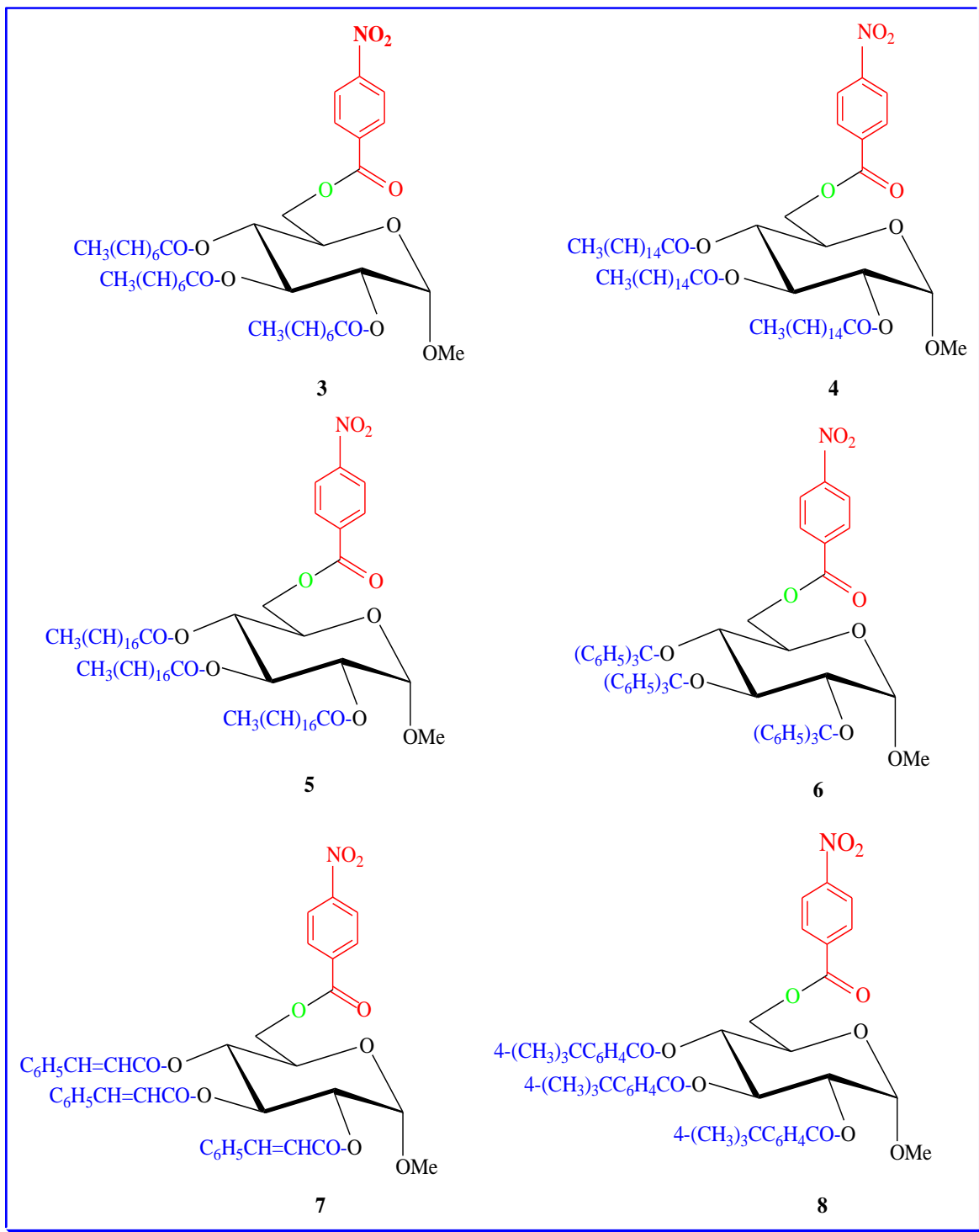
Figure 1. Chemical structures of glucopyranoside derivatives.
