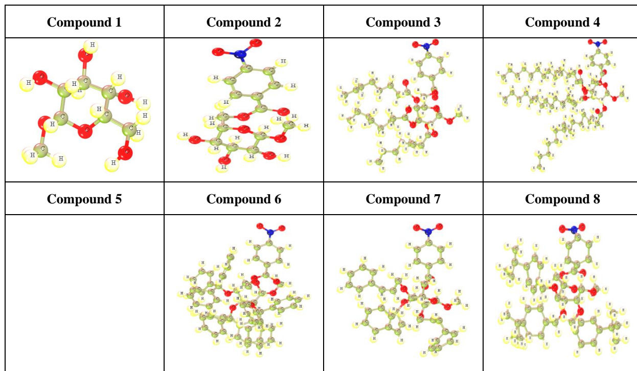
Figure S2. Optimized structure methyl \alpha -D-glucopyranoside derivatives.
