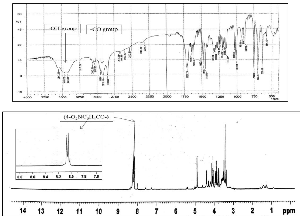
Figure S1. FTIR and 1 H-NMR spectra of the compound 2.
