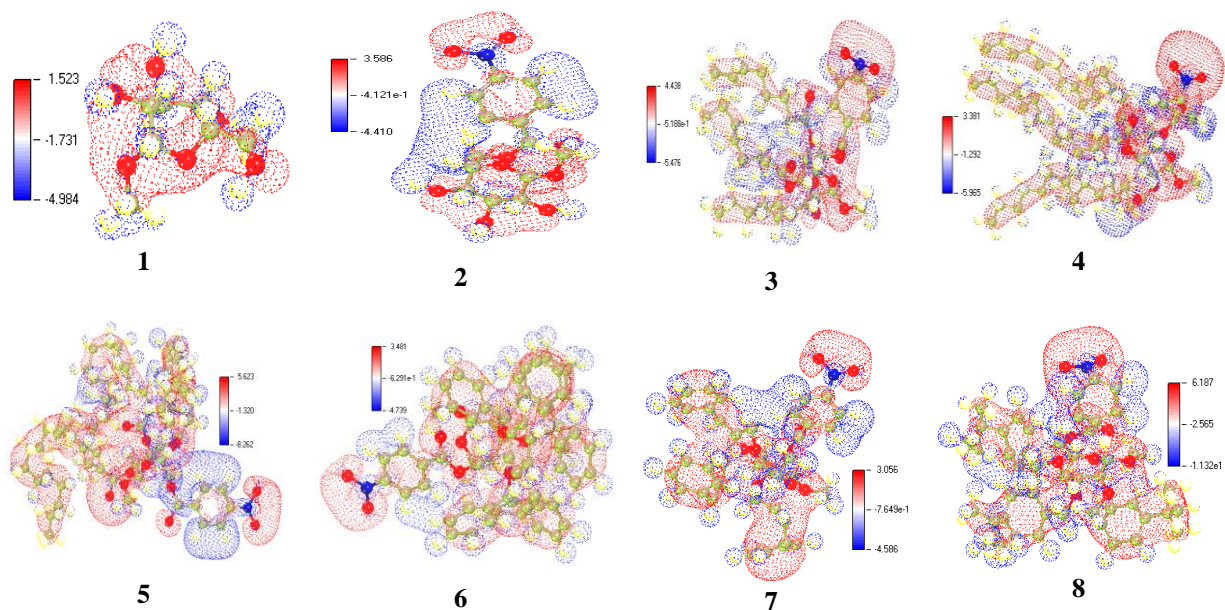
Figure 5. Molecular electrostatic potential (MEP) mappings.
