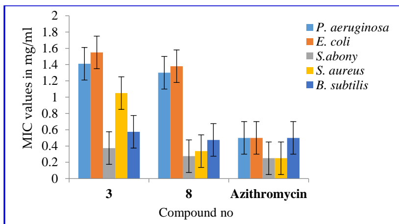
Figure 2. MIC values of the 3 and 8 compounds against tested organisms.
