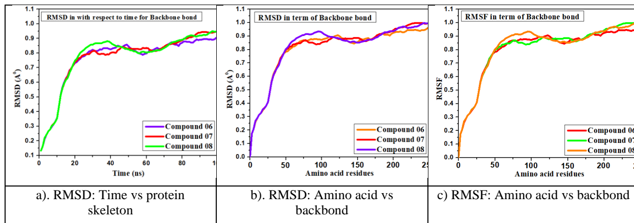
Figure S4. Various pictures of RMSD and RMSF for protein E. coli .
