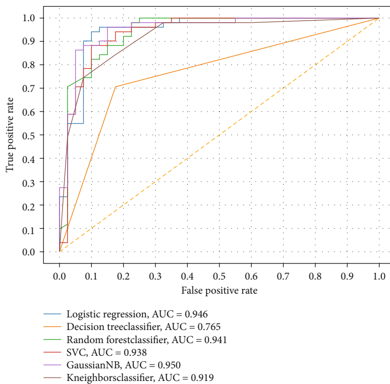
FIGURE 11: AUROC for SF2.
