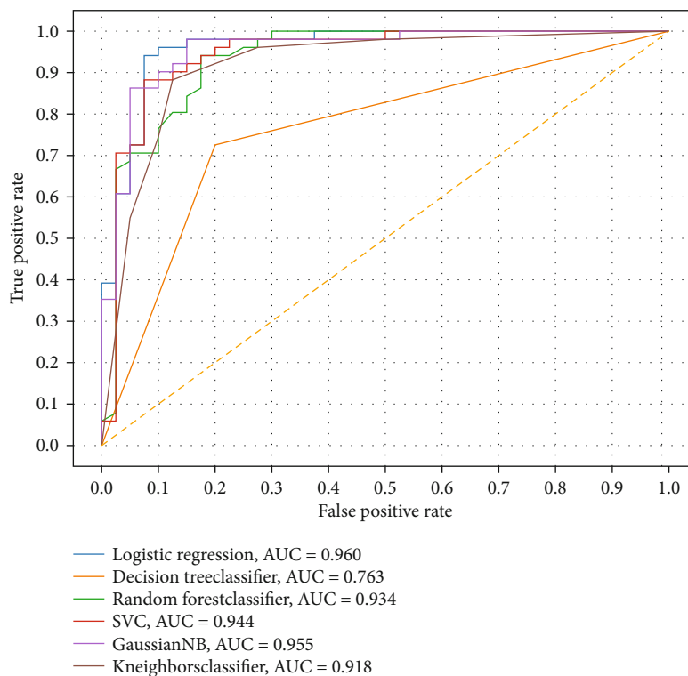
FIGURE 10: AUROC for SF1.
