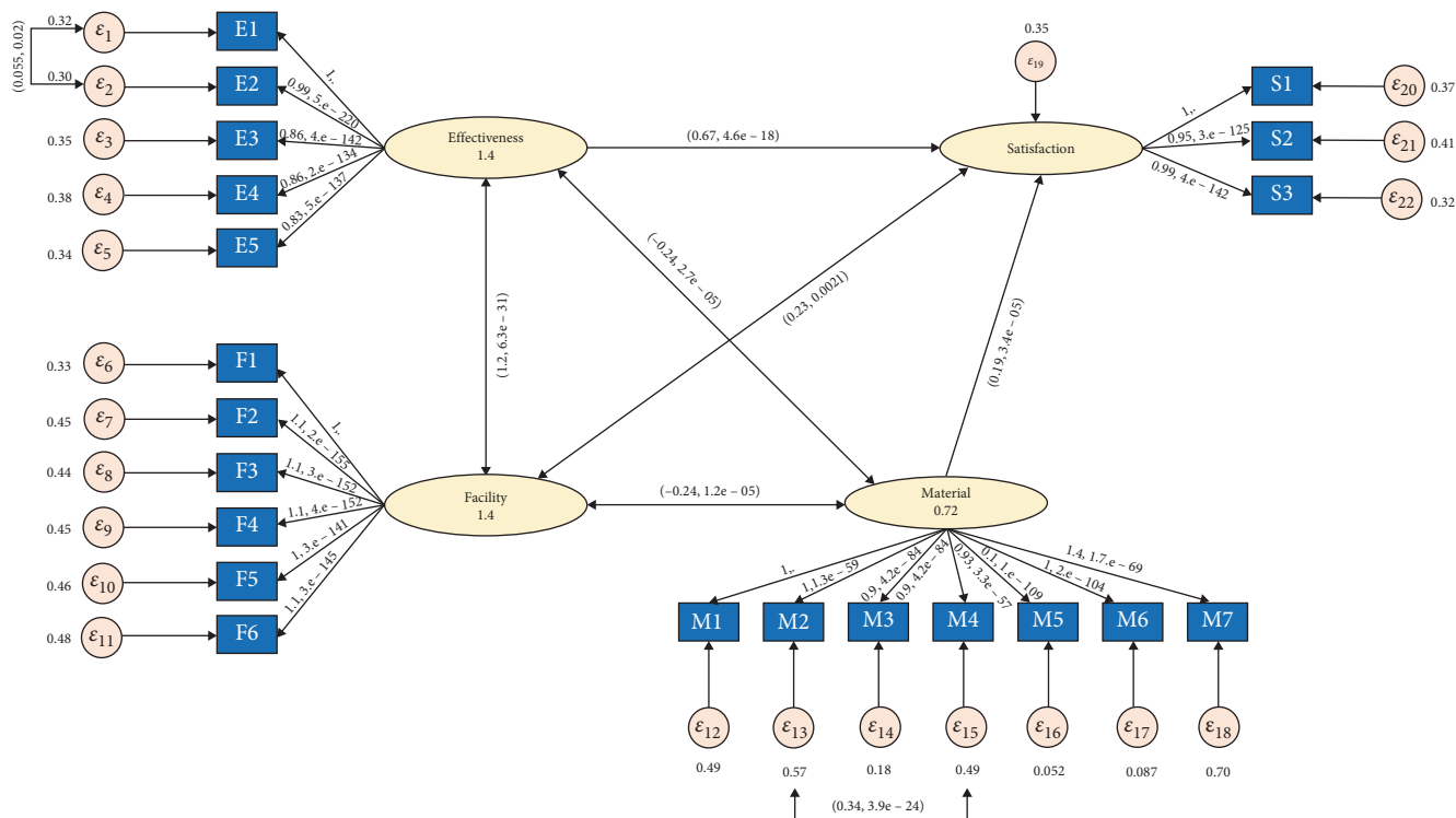
FIGURE 1: Path diagram among study variables.
