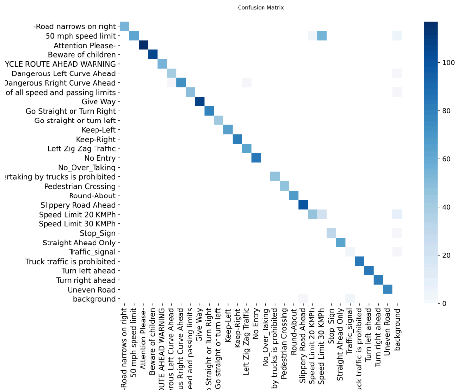
Figure 11: Confusion Matrix
