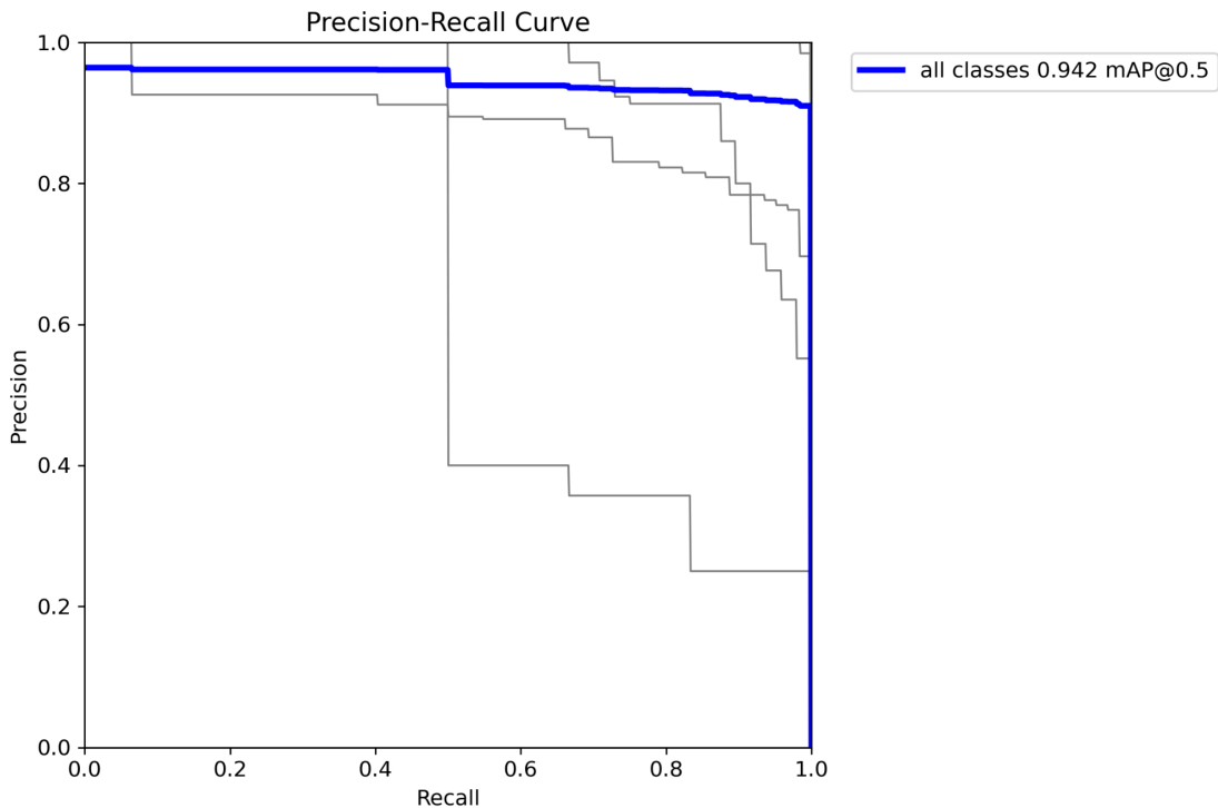
Figure 10: Precision-Recall Curve
