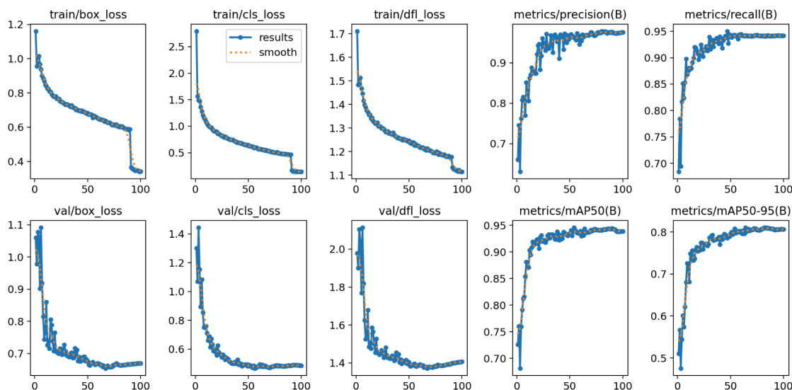
Figure 9: Training and Validation Metrics over 100 Epochs
