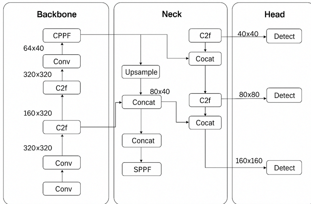
Figure 3: Architecture of the YOLOv8I Model
