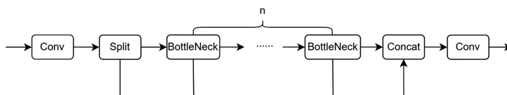
Figure 2: C2f network architecture.
