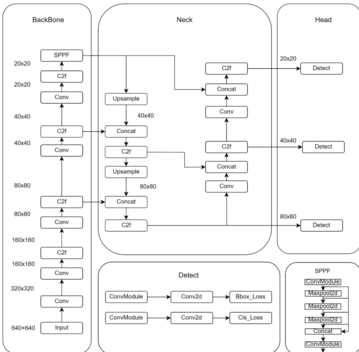
Figure 1: YOLOv8 network architecture.
