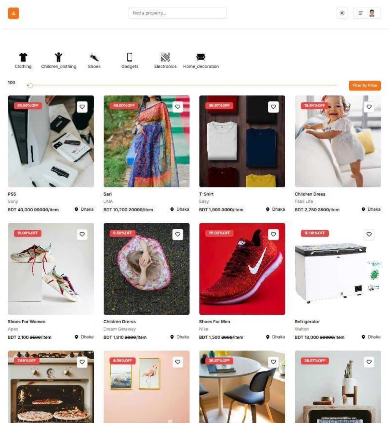
Figure 5.4: Home Page
