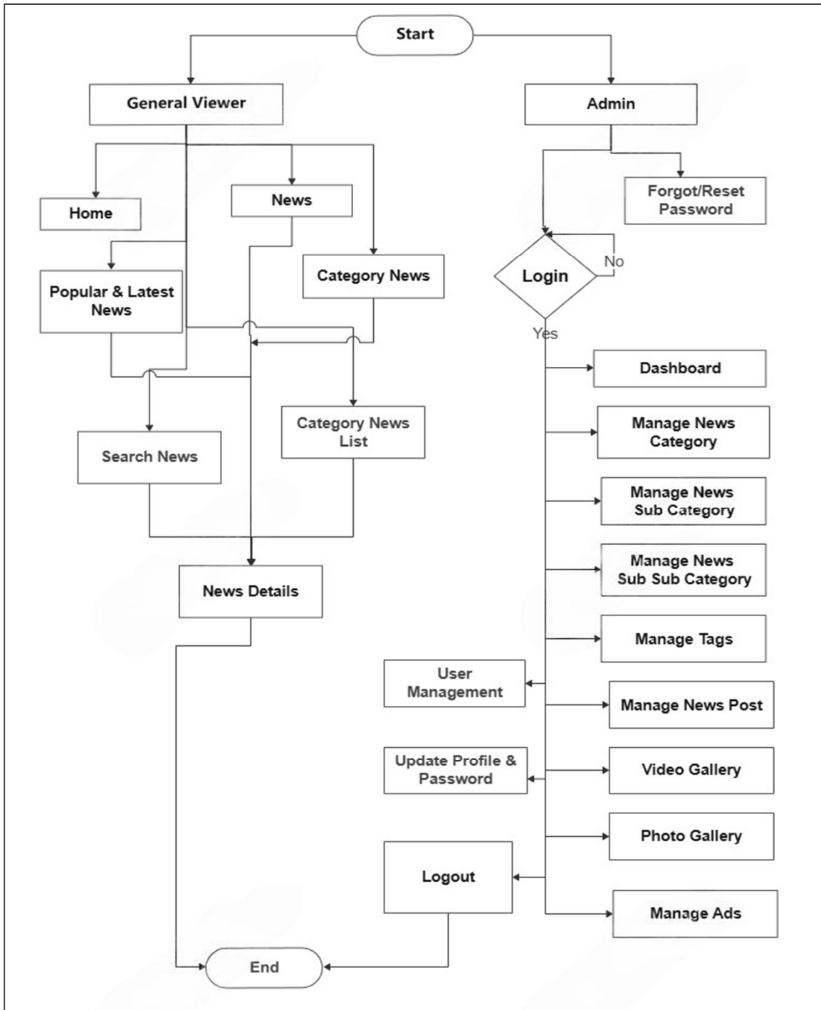
Fig 3.2: System flow chart
