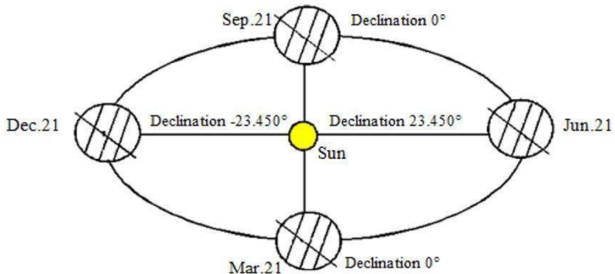
Figure 2.4: Declination AngleHour Angle
