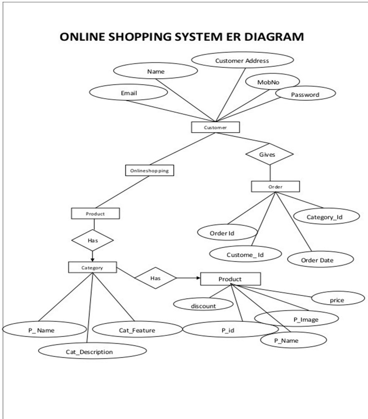
Figure 3.3.3.1: ER Diagram of the Project
