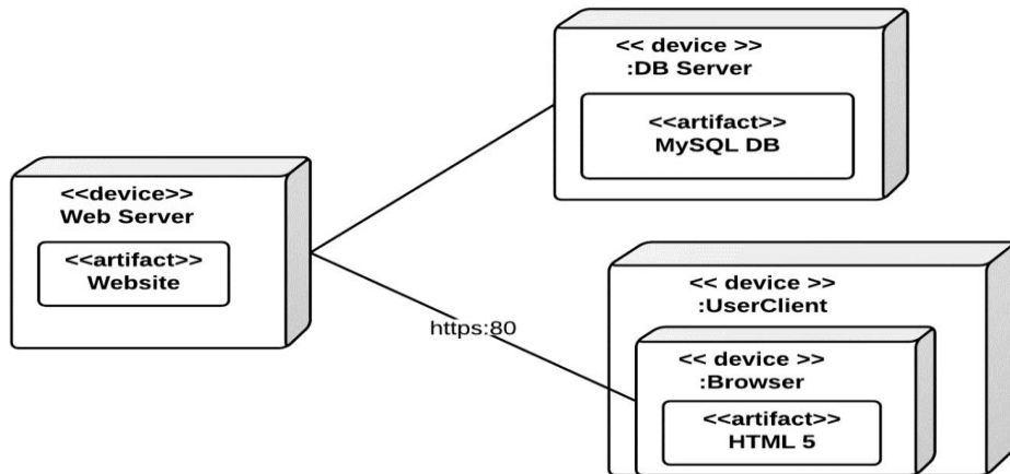
Figure 3.11: Component Diagram
