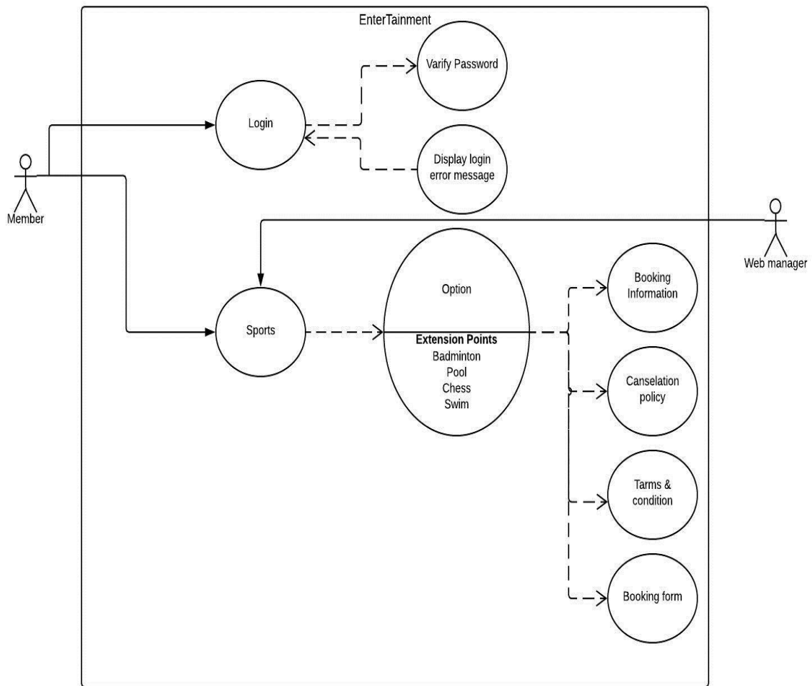
Figure 3.8.3: Use Case Diagram of Member login in System
