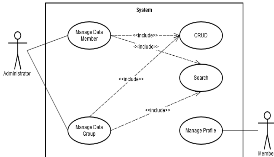
Figure3.8.1: Use Case Diagram of Administrator
