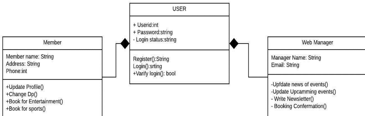
Figure 3.12: Class Diagram
