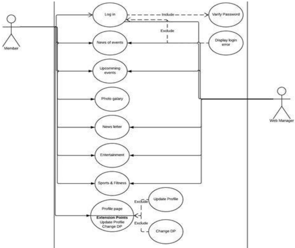
Figure 3.8.2: Use Case Diagram of Member
