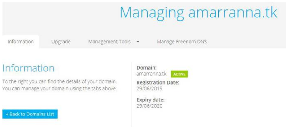
Figure 3.1: Domain Registrations
