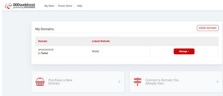
Figure 3.2: Web Hosting
