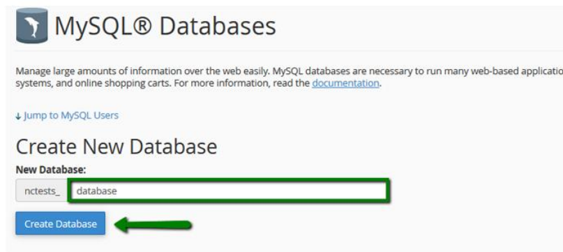
Figure 3.4: Database Create
