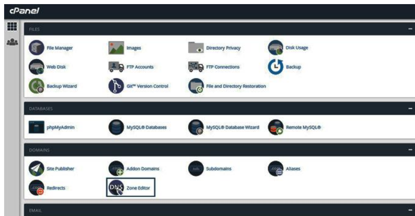
Figure 3.3: c-Panel Login
