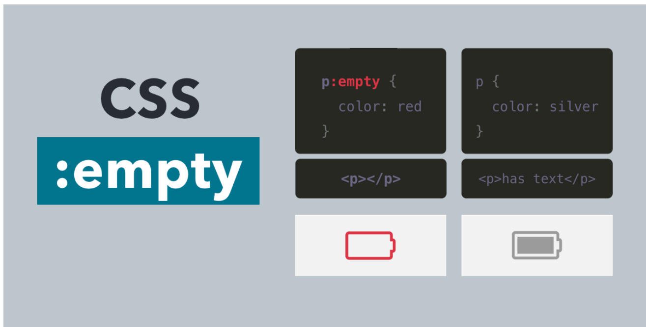
Figure 4.2: CSS
