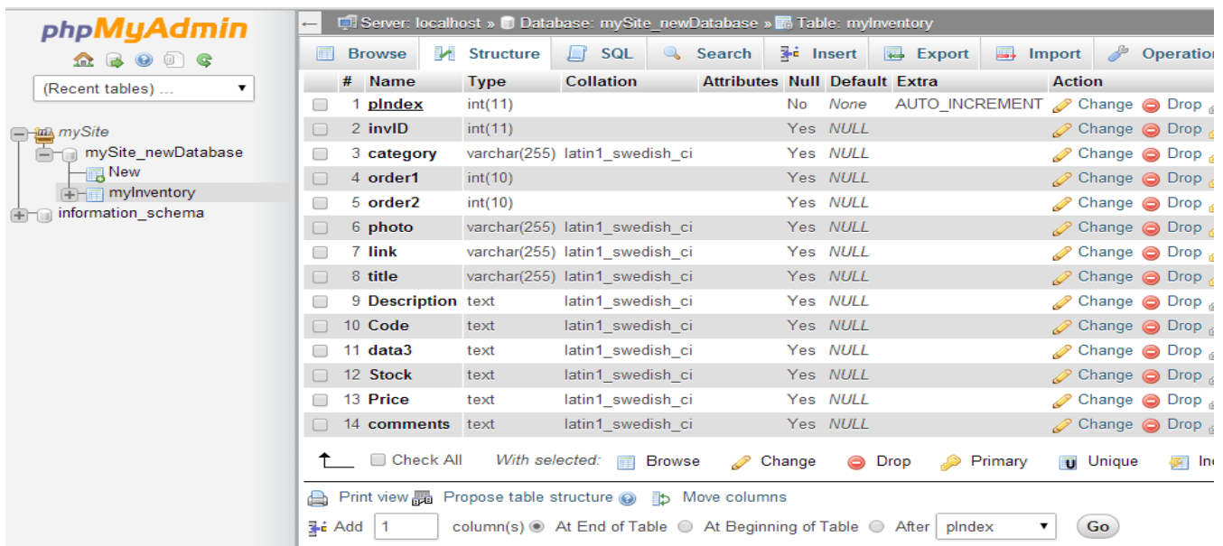
Figure 3.2: Database
