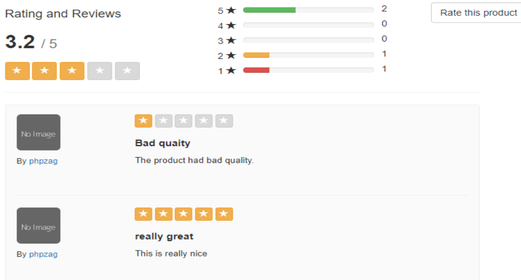
Figure 3.3: Rating & Review
