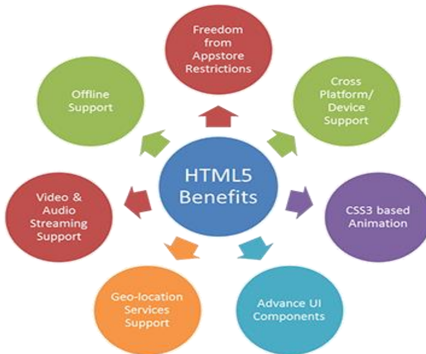
Figure 4.1: Html 5
