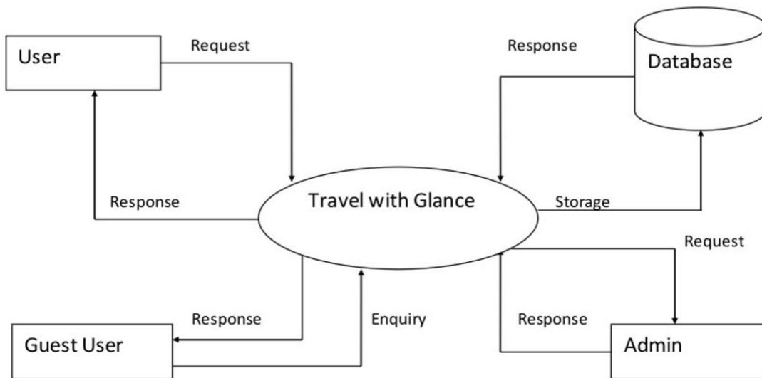
Figure 3.5: Tours & travels management system design
