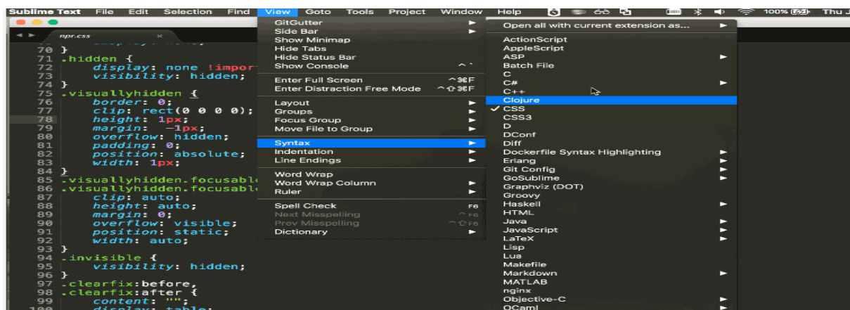
Figure 4.2: CSS3
