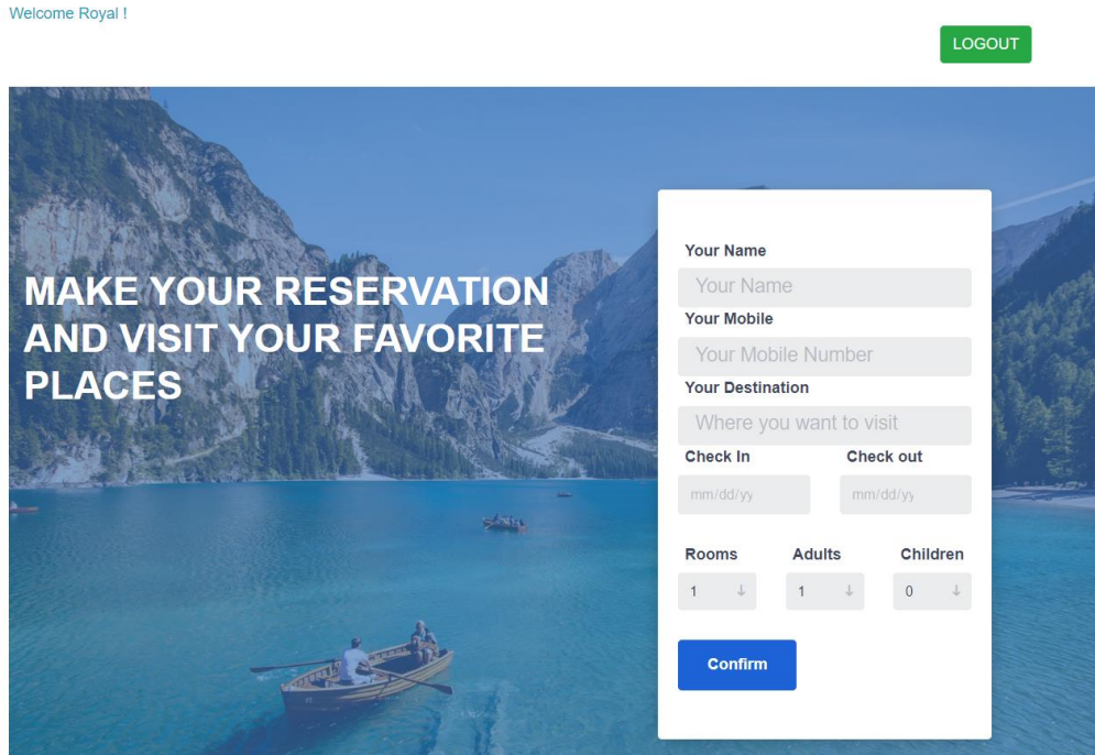
Fig3.13 Customer dashboard
