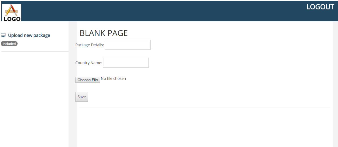
Fig3.14 Admin Pannel
