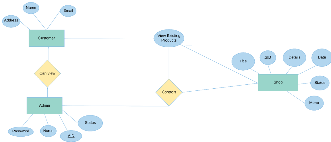
Figure 3.2: ER-Diagram
