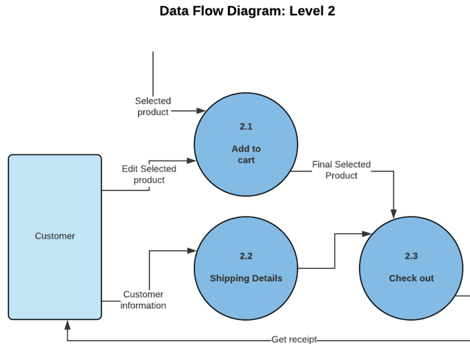
Figure 3.5: DFD-Level 2
