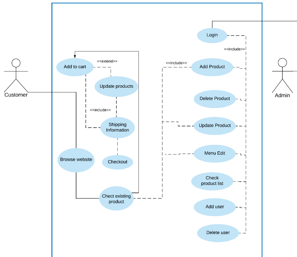
Figure 3.1: Use-case Diagram
