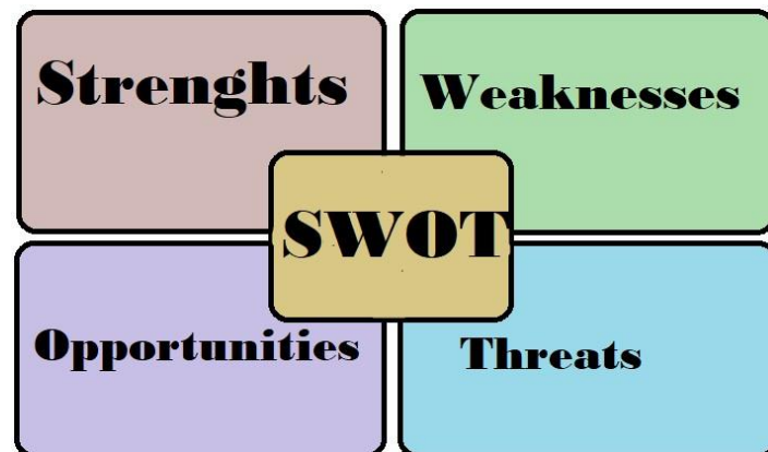
Figure 2.6.1: SWOT Analysis
