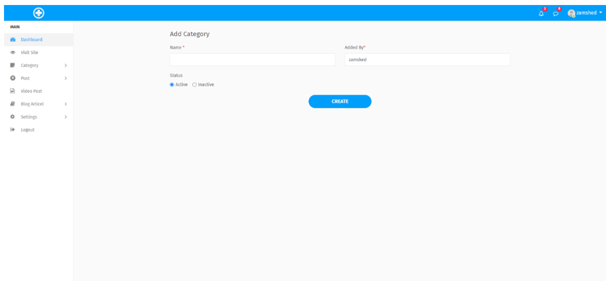
Figure 3.12: Add Category
