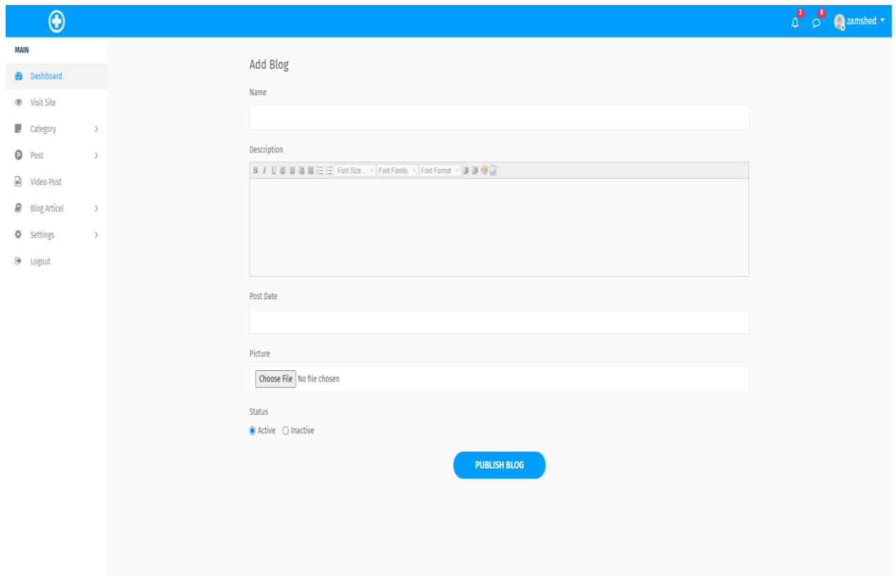
Figure 3.11: Add Blog
