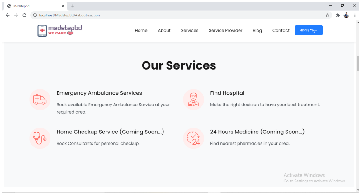
Fig 4.1.3: Service Section
