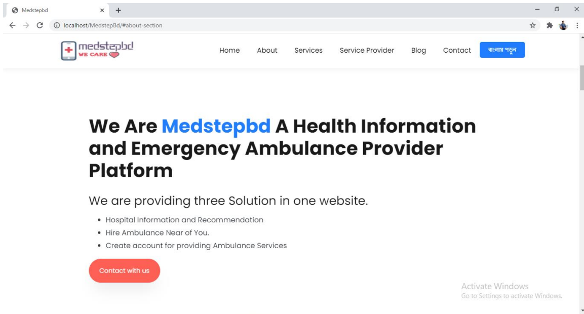
Fig 4.1.2: About Section
