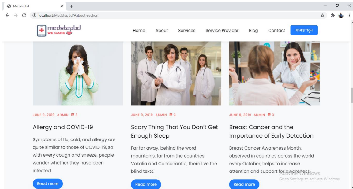
Fig 4.1.4: Blog Section
