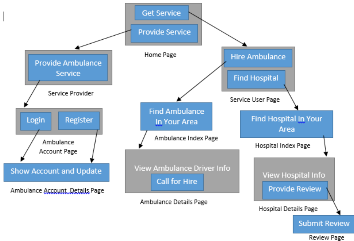
Fig 4.3: Interaction Design
