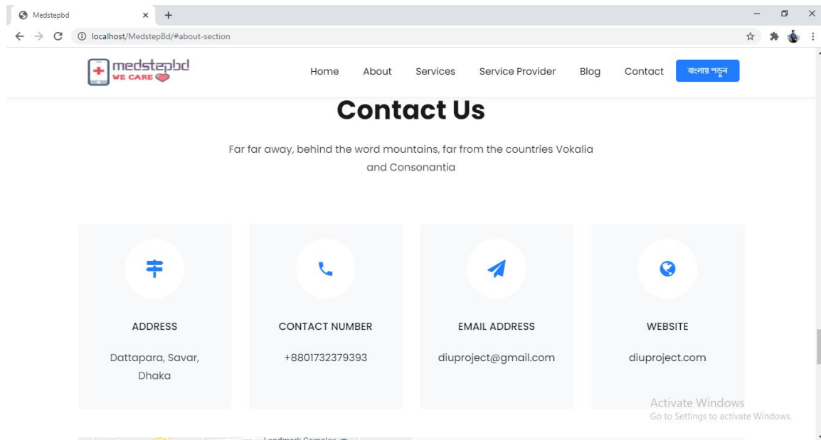
Fig 4.1.5: Contact Section
