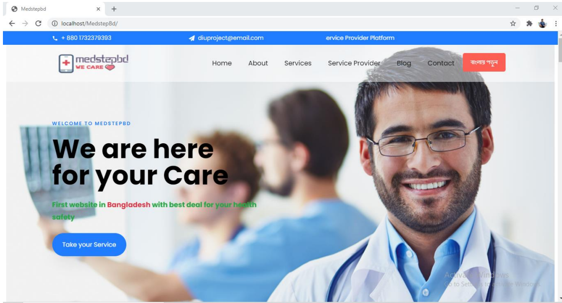
Fig 4.1.1: Homepage
