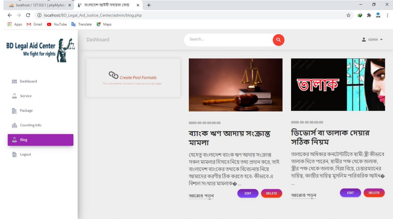
Figure 5.2.4.4: Blog Update
