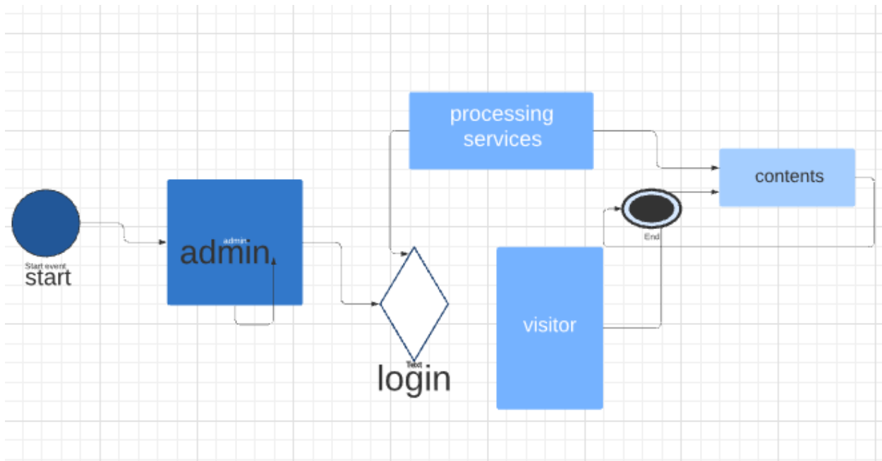
Figure 3.1: BPMN
