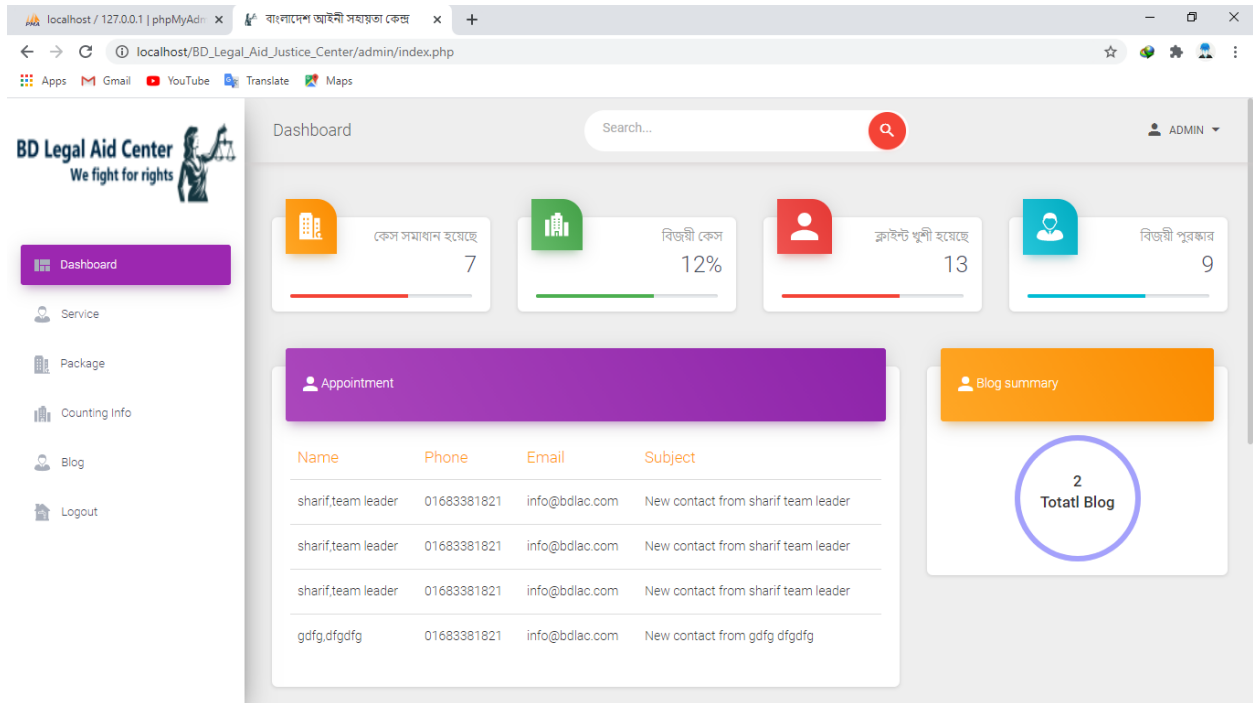
Figure 5.2.3: Admin Dashboard
