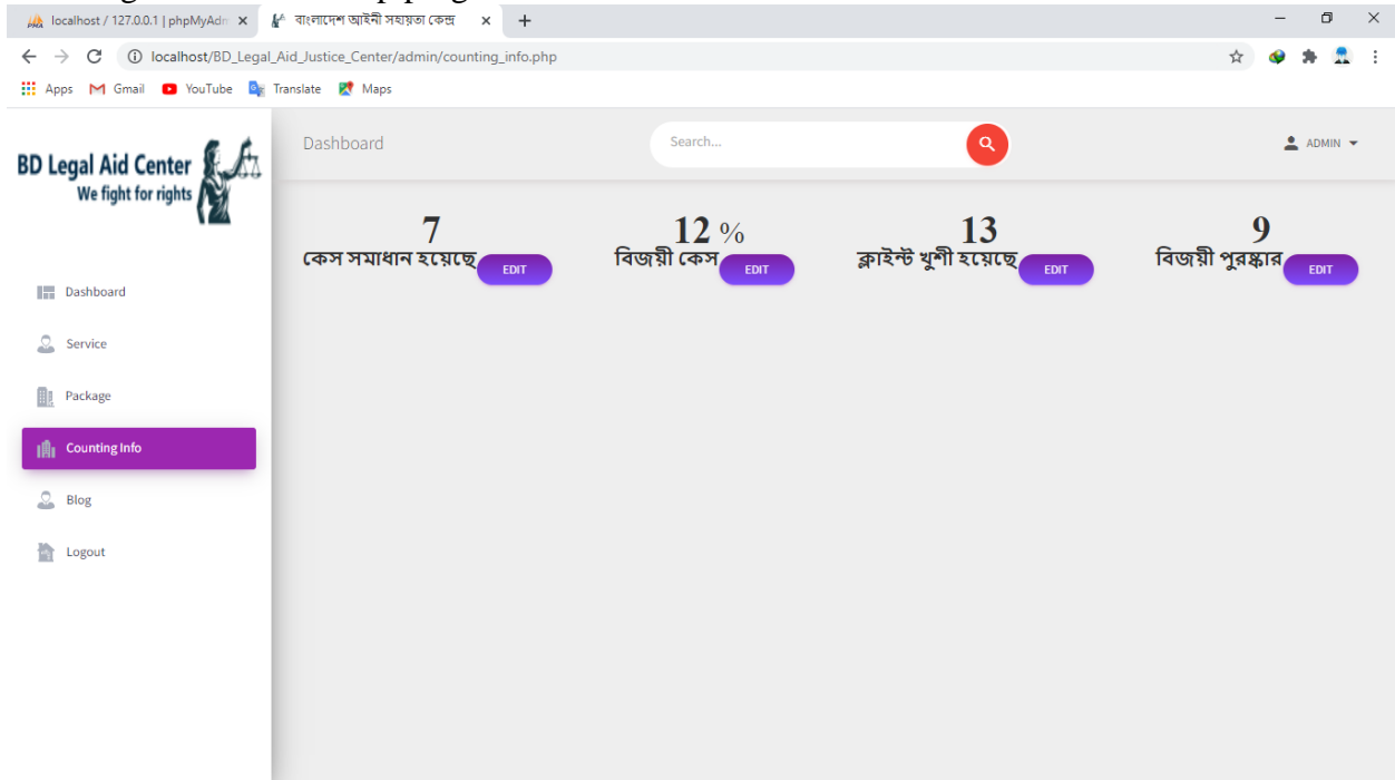
Figure 5.2.4.3: Counting Info
