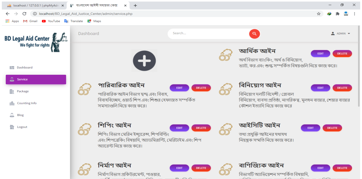
Figure 5.2.4.1: Admin Services
