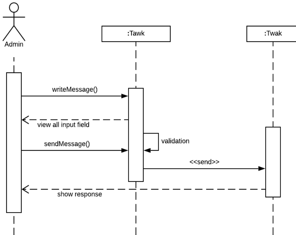
Figure 3.6.21: Sequence diagram for live chat
