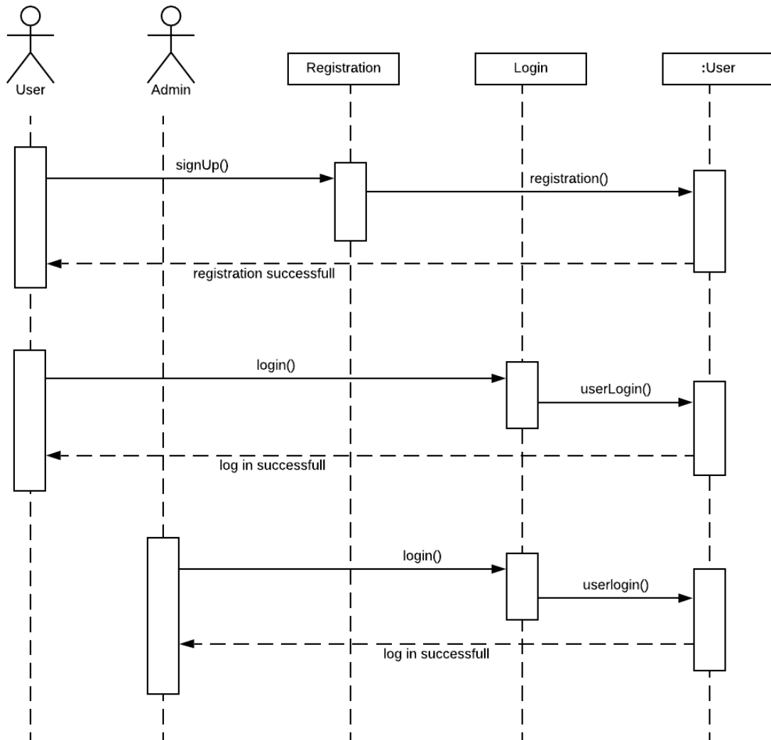
Figure 3.6.1: Sequence diagram for log in and registration
