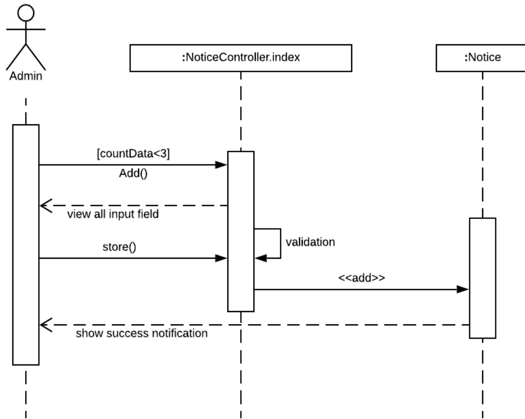
Figure 3.6.12: Sequence diagram for add notice
