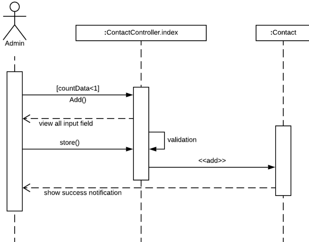
Figure 3.6.13: Sequence diagram for add contact us
