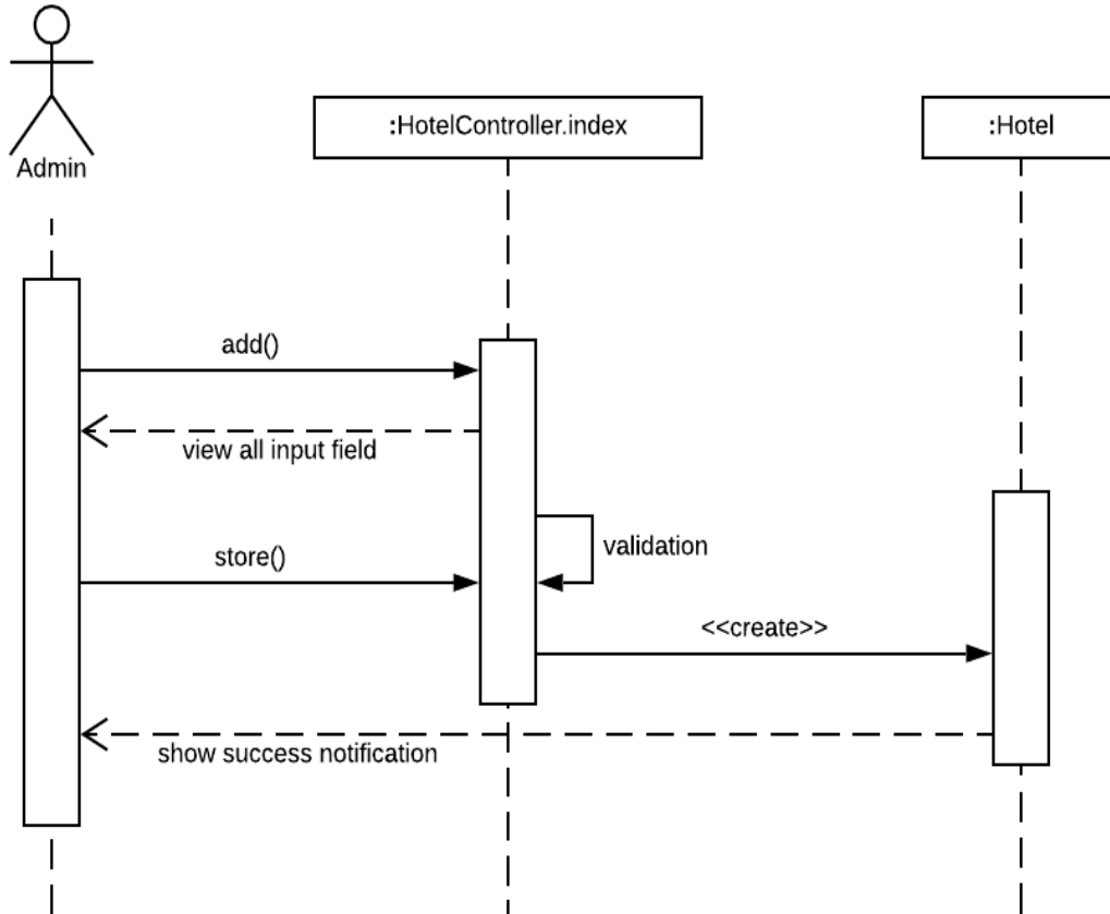
Figure 3.6.17: Sequence diagram for add hotel
