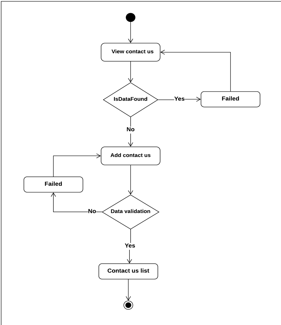
Figure 3.5.15: Add contact us activity diagram
