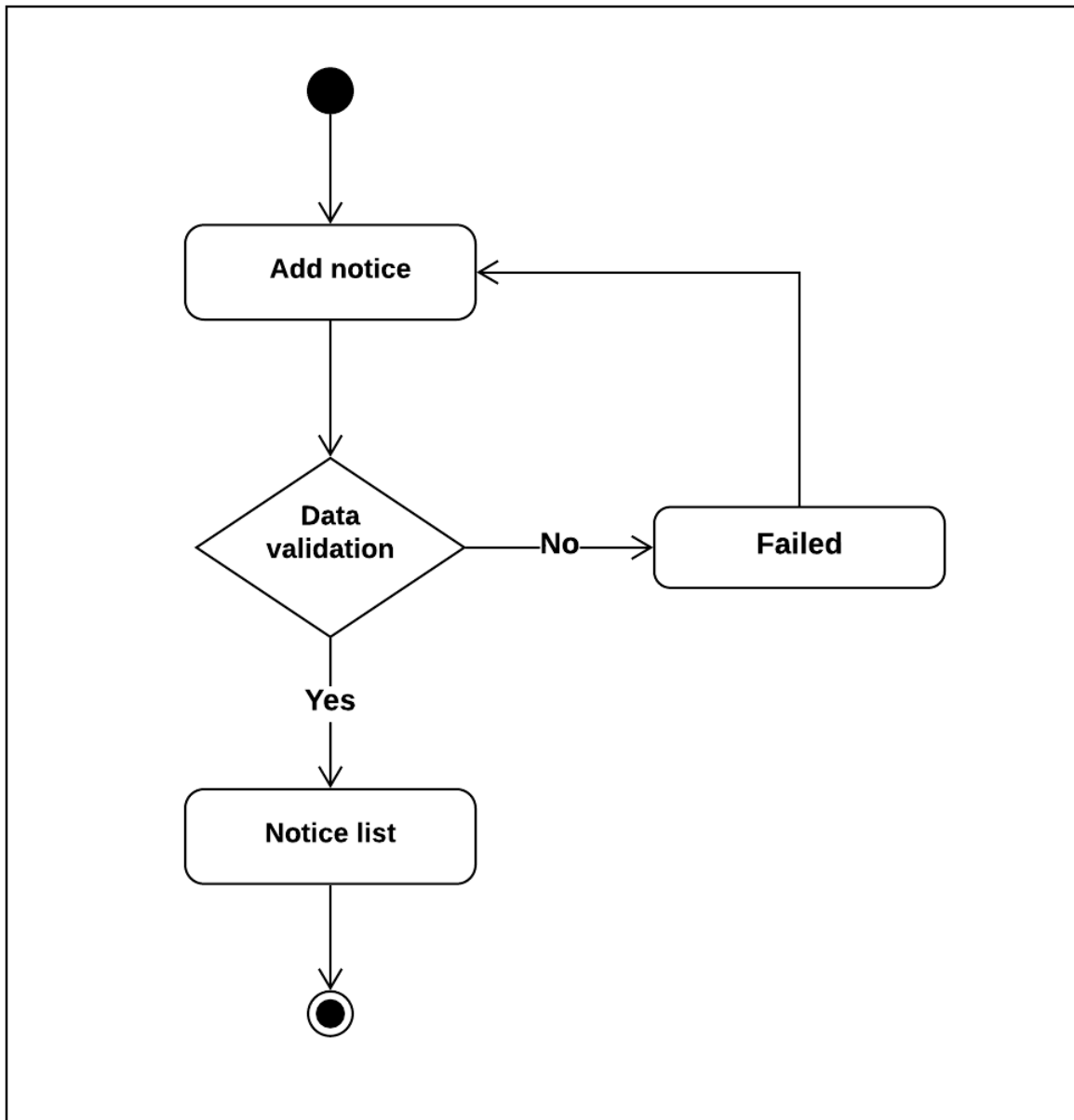
Figure 3.5.14: Add notice activity diagram
