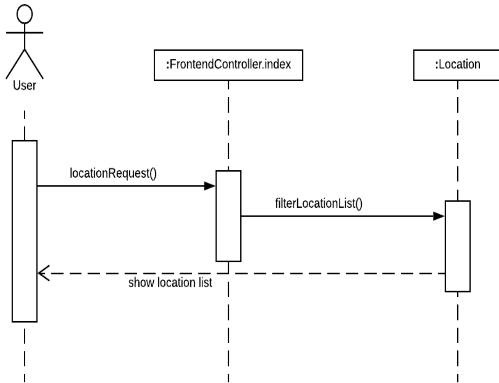
Figure 3.6.2: Sequence diagram for find location
