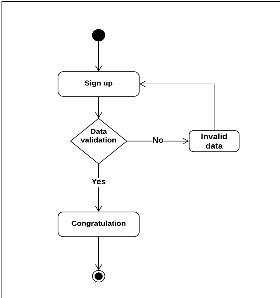
Figure 3.5.1: User sign up activity diagram
