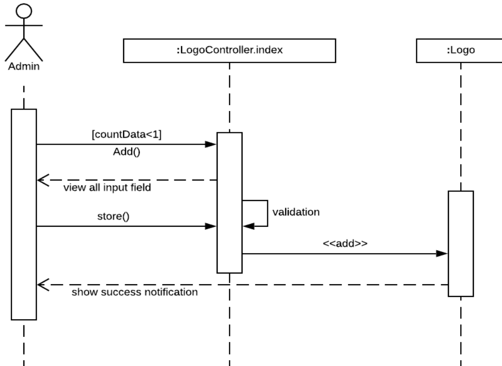
Figure 3.6.10: Sequence diagram for add logo
