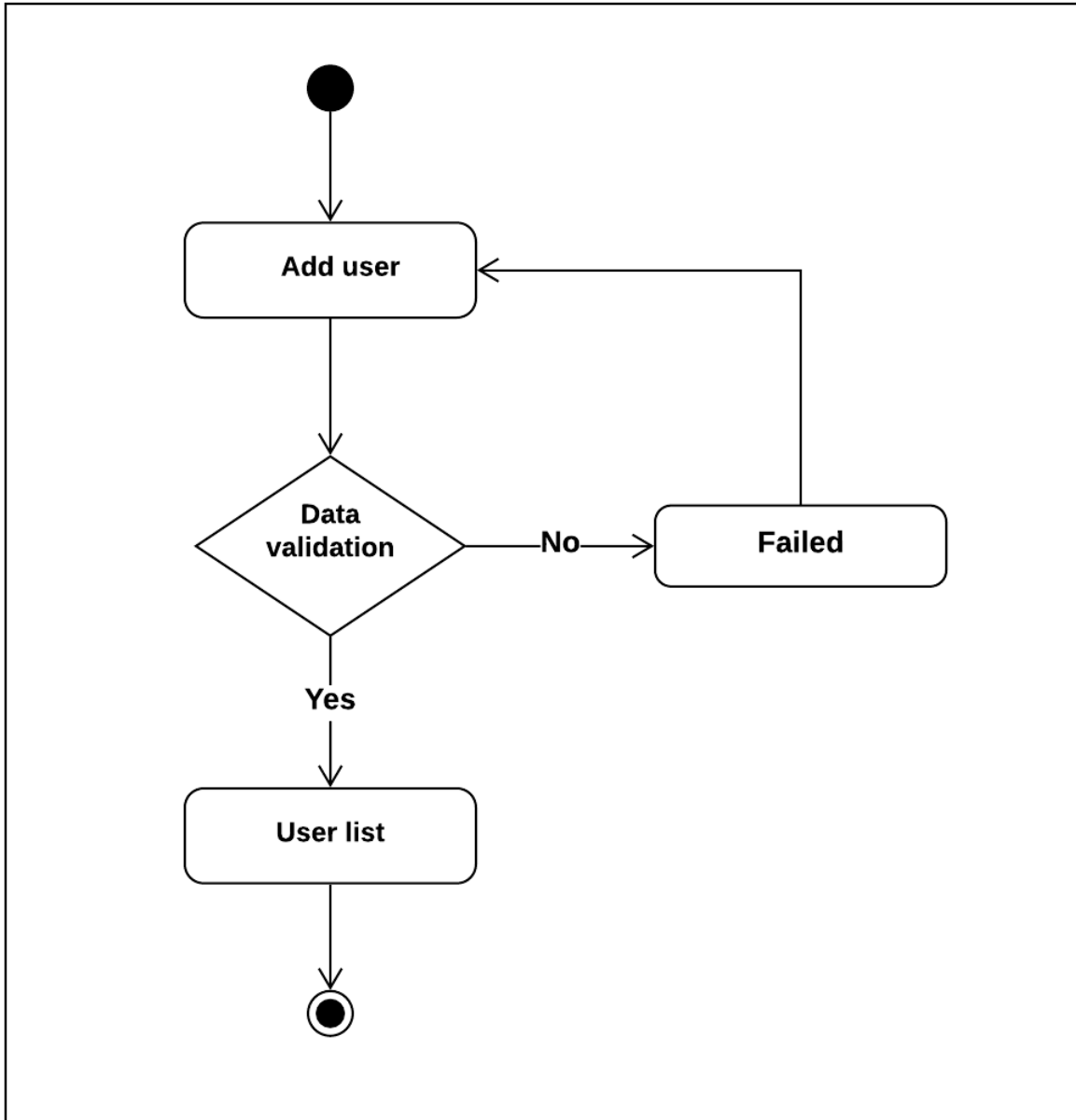
Figure 3.5.10: Add user activity diagram
