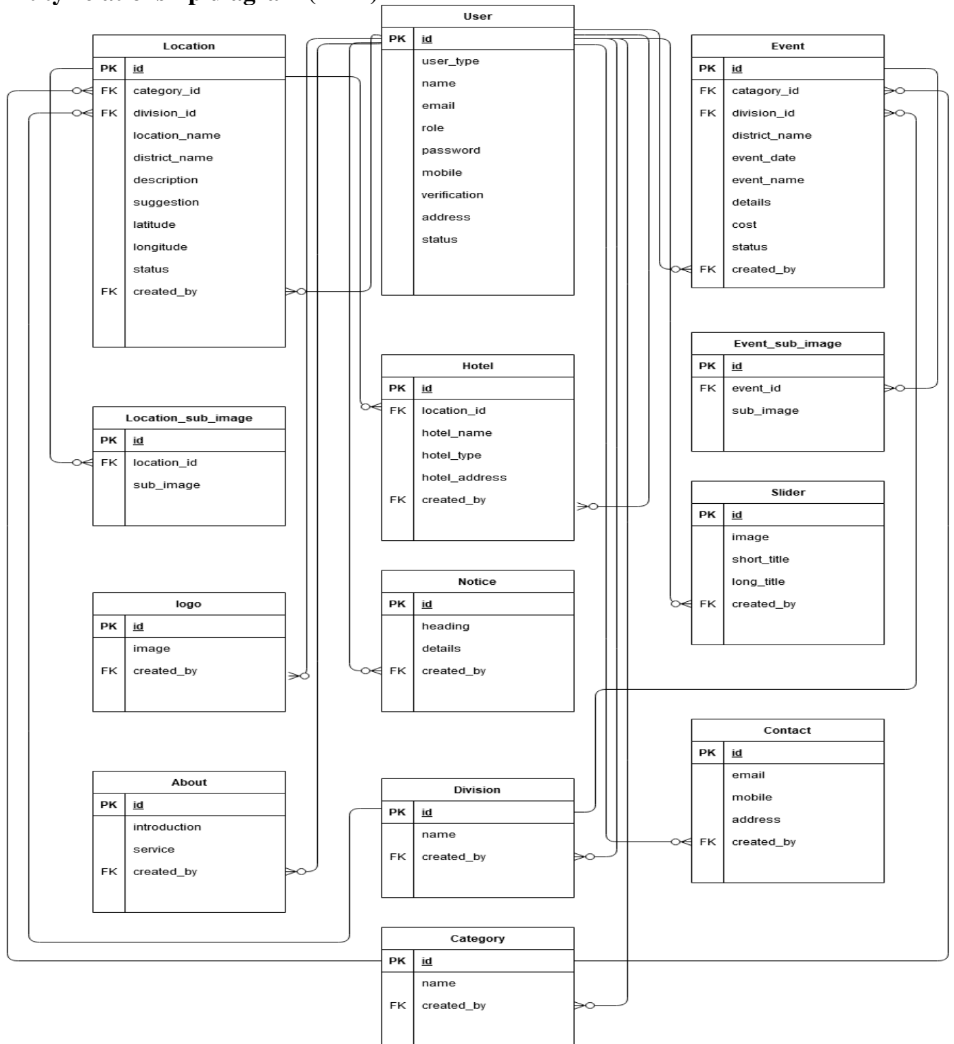
Figure 4.9: Entity relationship diagram
