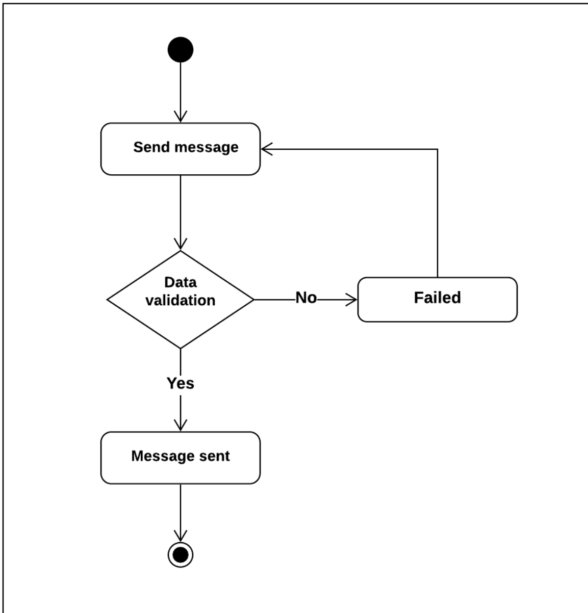
Figure 3.5.8: Live chat activity diagram
