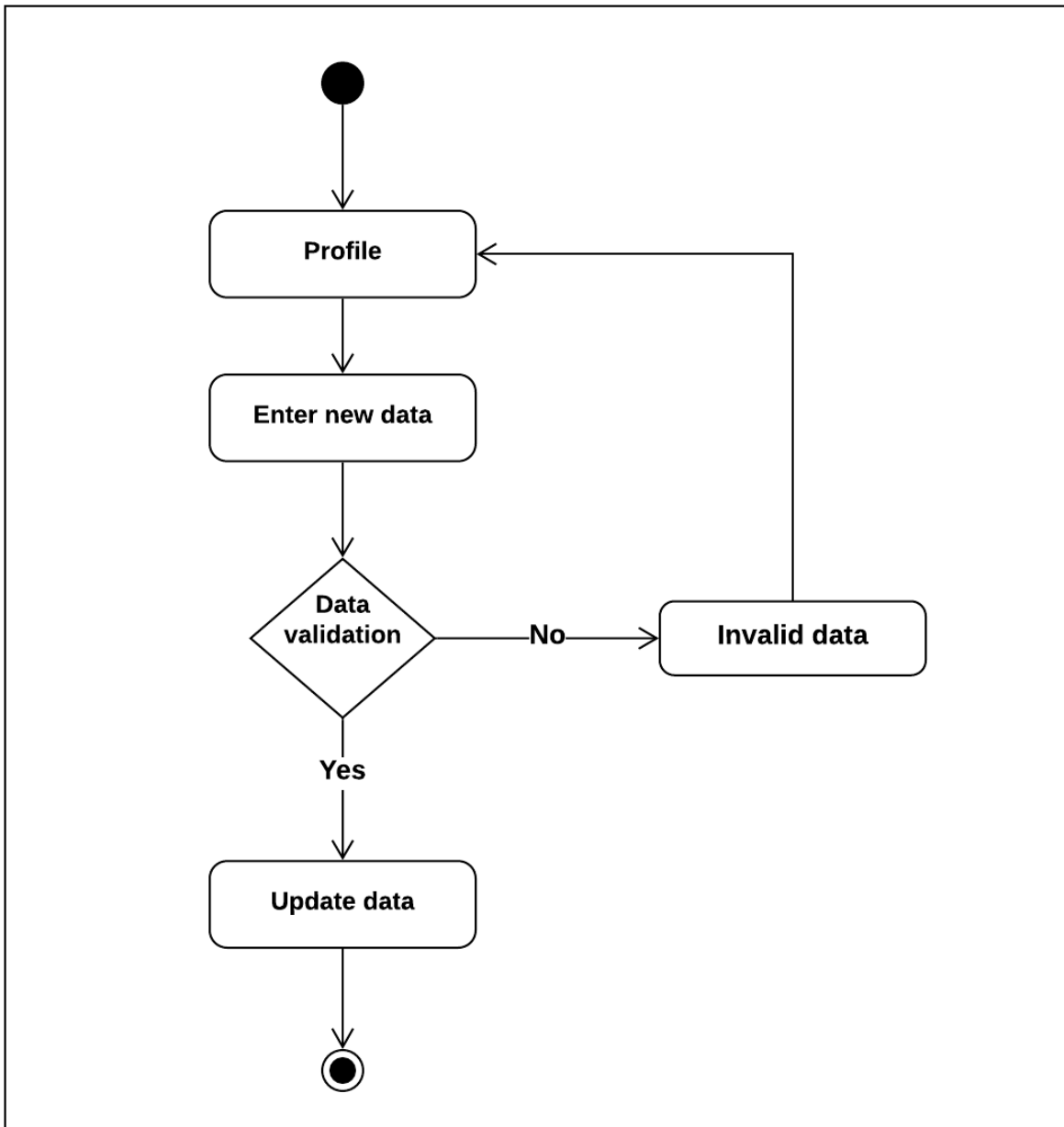
Figure 3.5.4: Update profile activity diagram
