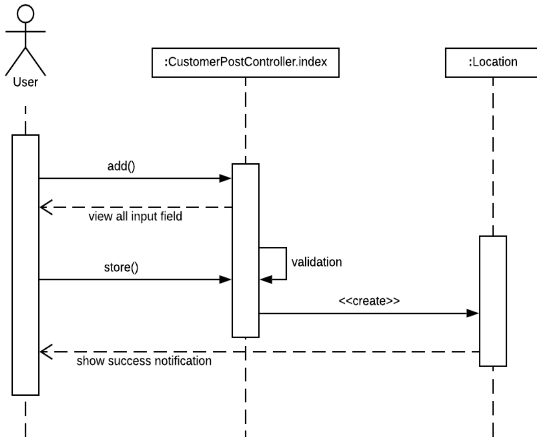
Figure 3.6.4: Sequence diagram for create post
