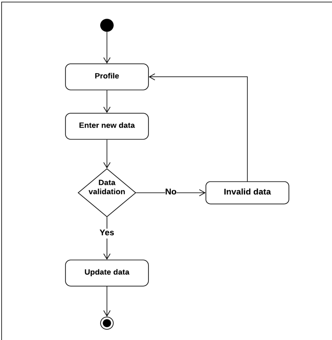
Figure 3.5.11: Update profile activity diagram
