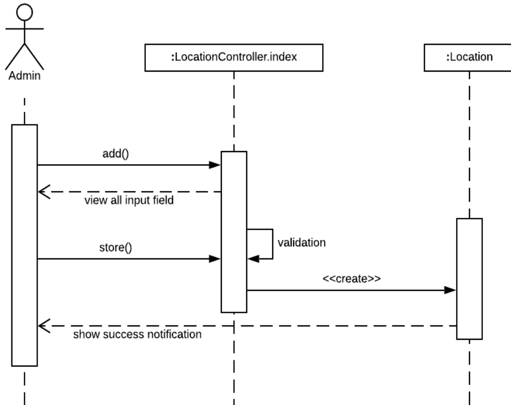
Figure 3.6.18: Sequence diagram for add location
