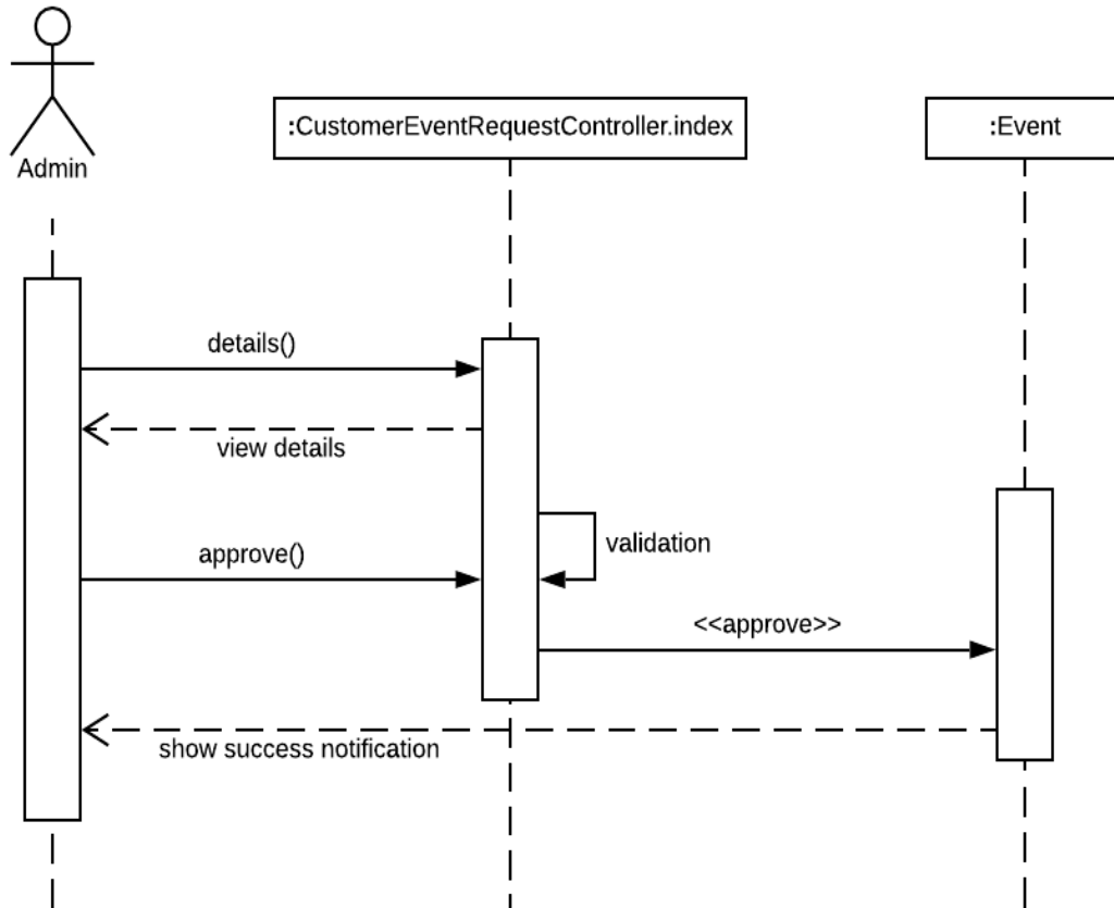
Figure 3.6.20: Sequence diagram for manage event request
