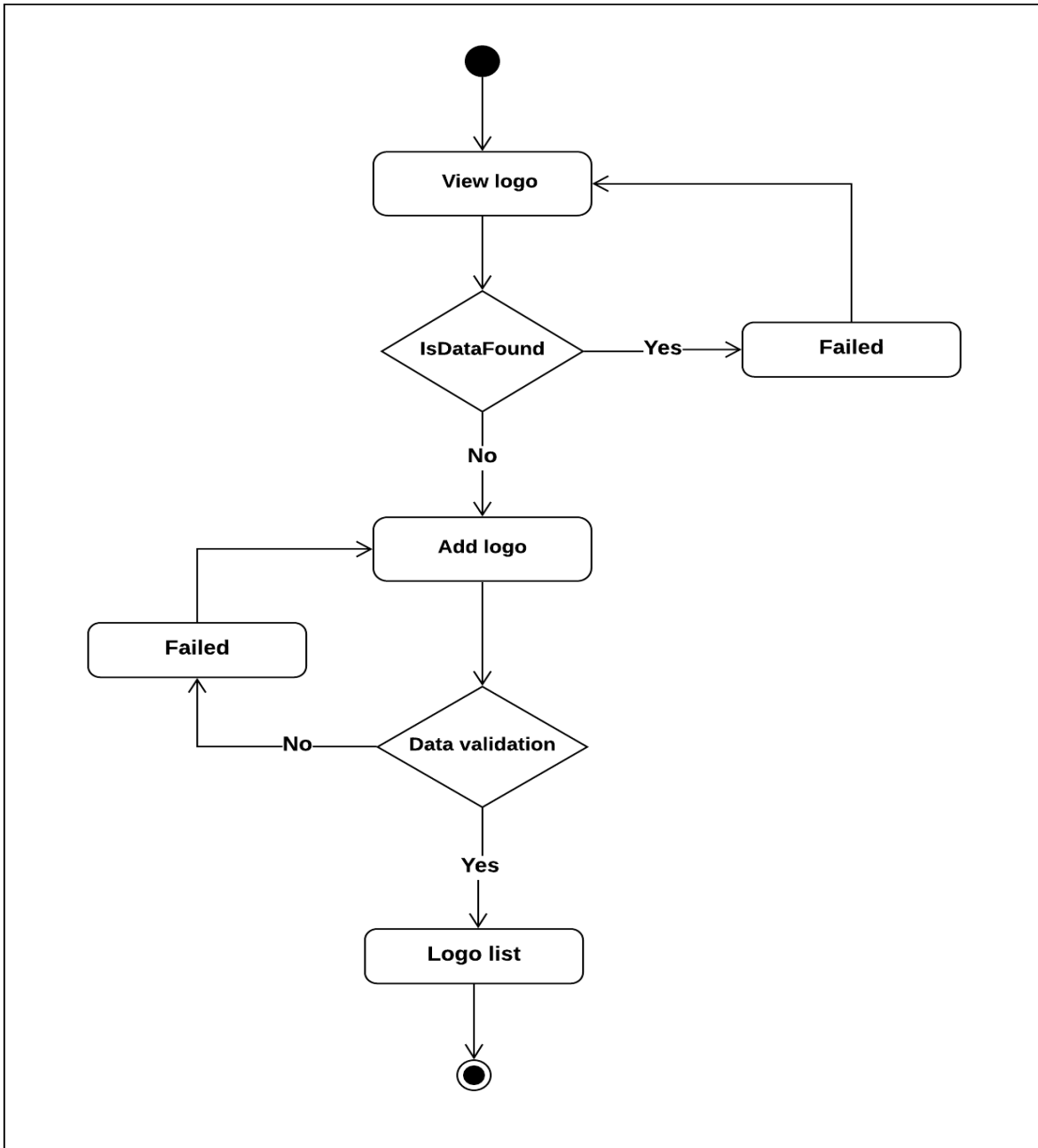
Figure 3.5.12: Add logo activity diagram
