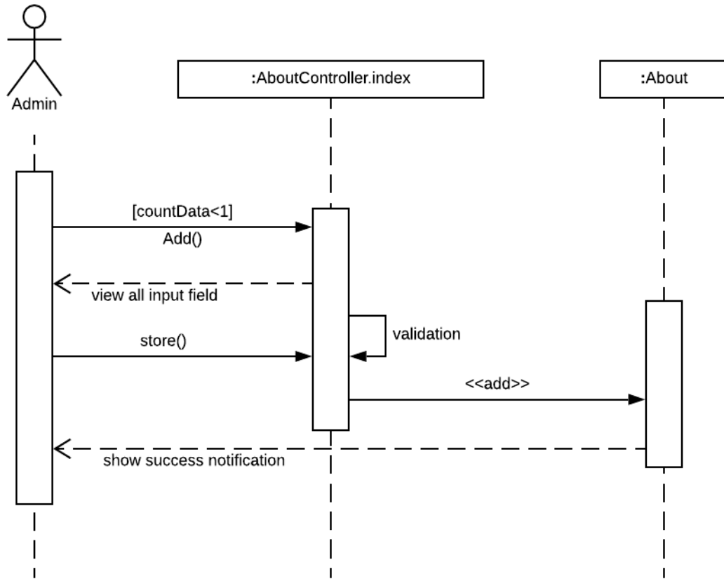
Figure 3.6.14: Sequence diagram for add about us
