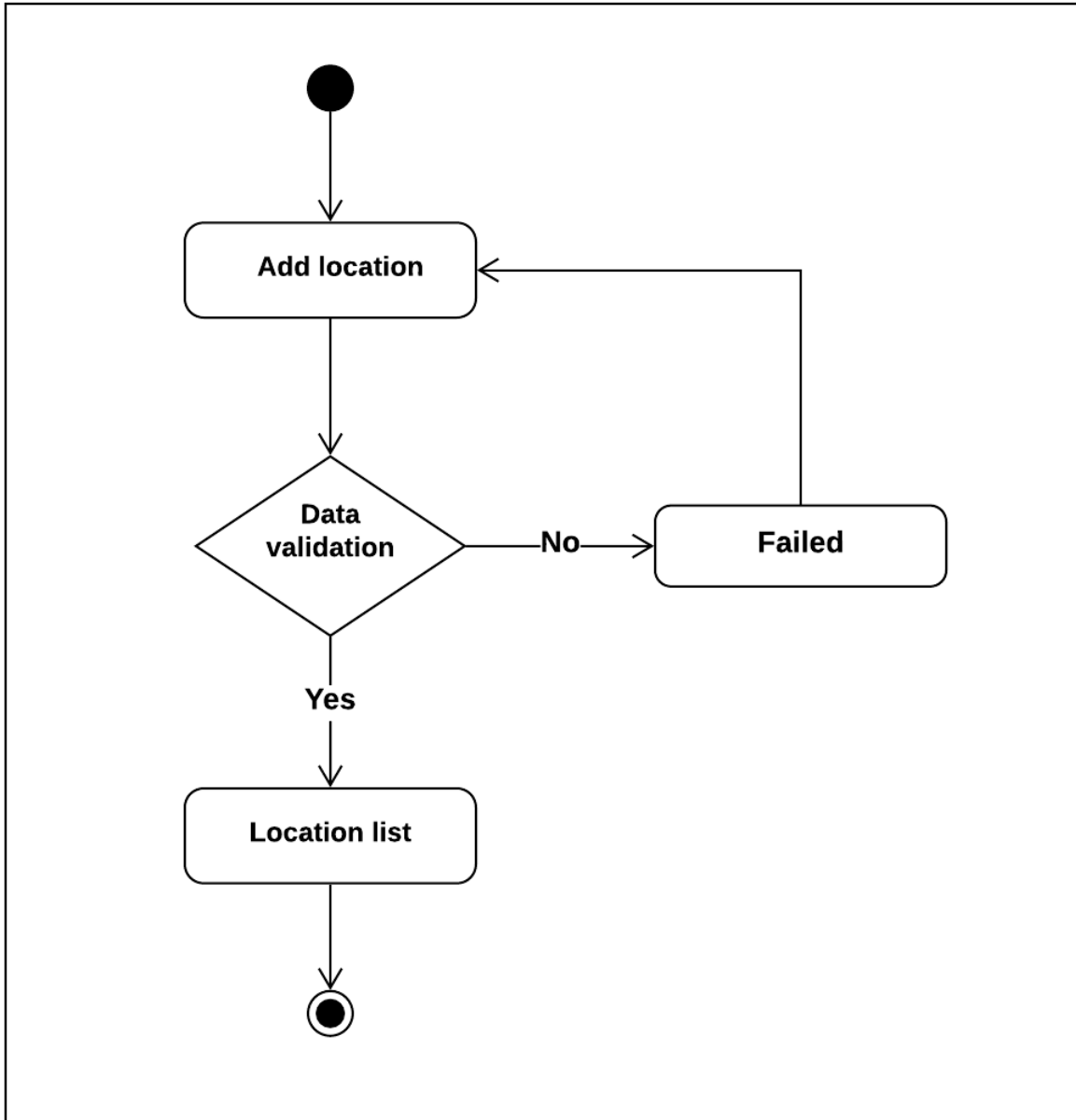
Figure 3.5.20: Add location activity diagram
