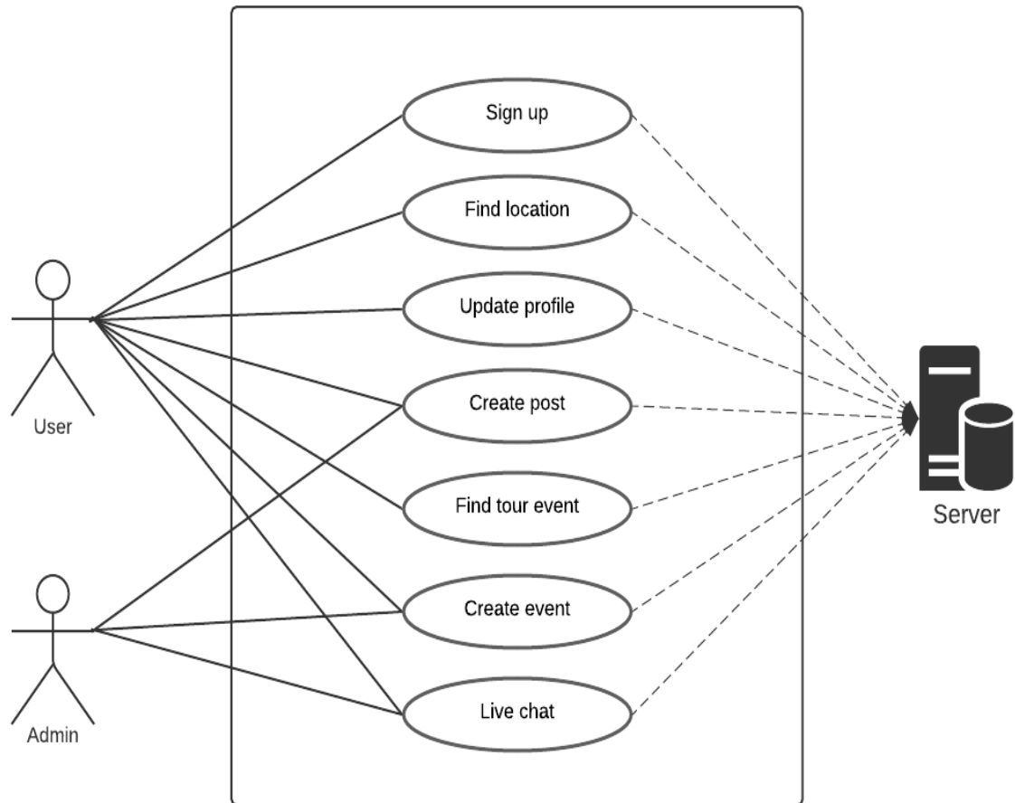
Figure 3.1: Use case diagram (User)
