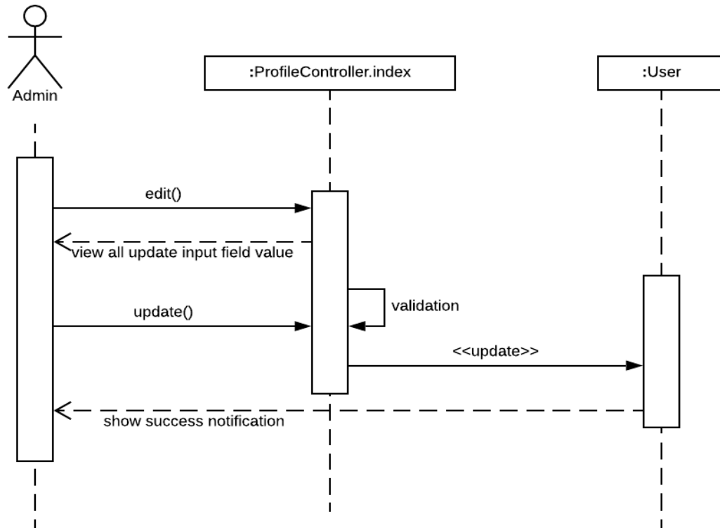
Figure 3.6.9: Sequence diagram for update profile
