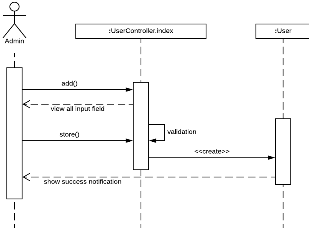
Figure 3.6.8: Sequence diagram for add user
