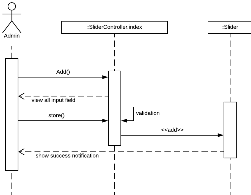
Figure 3.6.11: Sequence diagram for add slider
