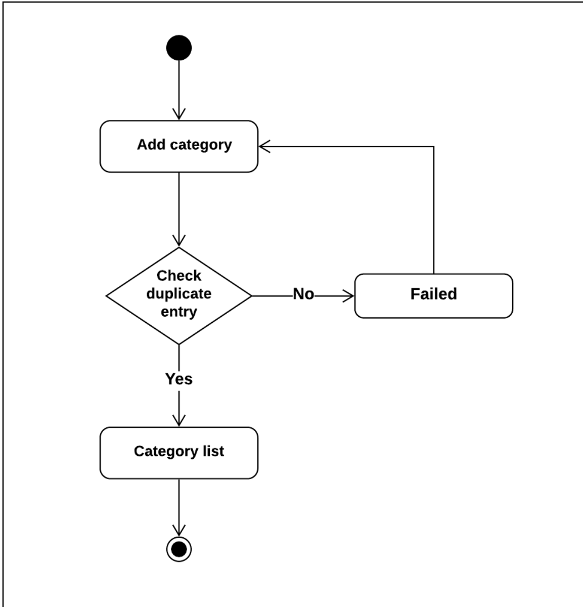
Figure 3.5.18: Add category activity diagram
