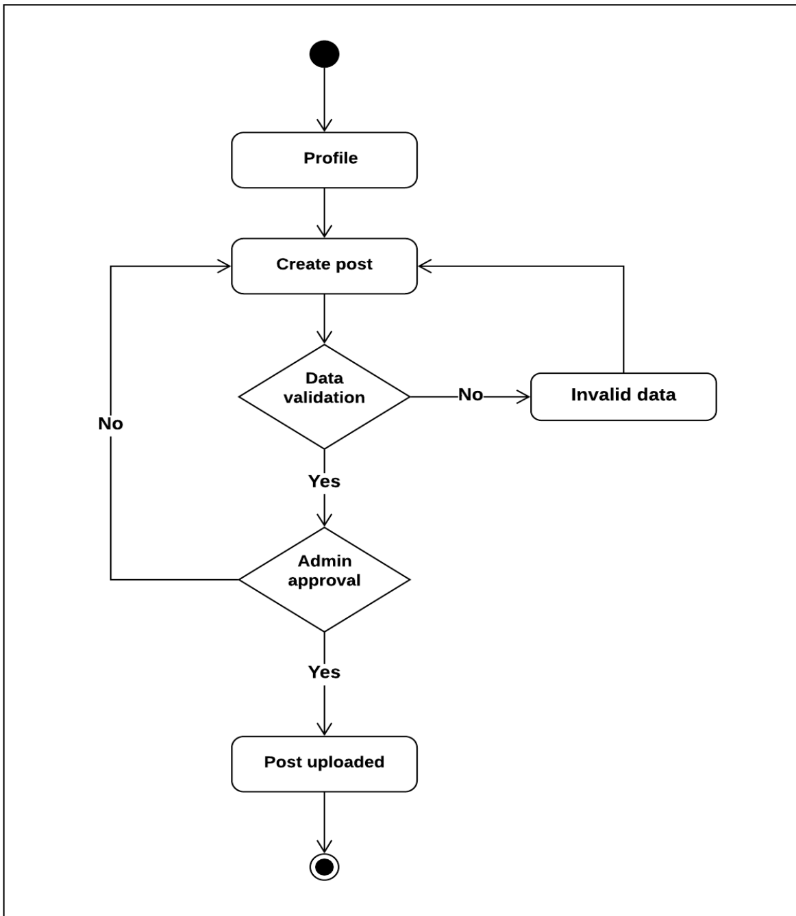
Figure 3.5.5: Create post activity diagram
