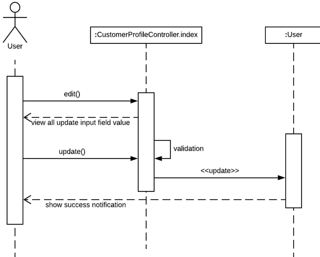
Figure 3.6.3: Sequence diagram for update profile
