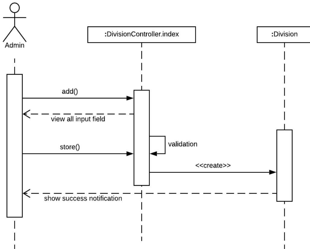
Figure 3.6.15: Sequence diagram for add division
