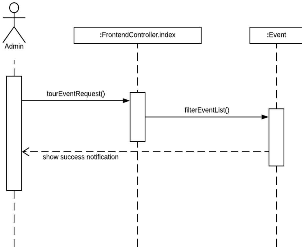
Figure 3.6.5: Sequence diagram for find tour event
