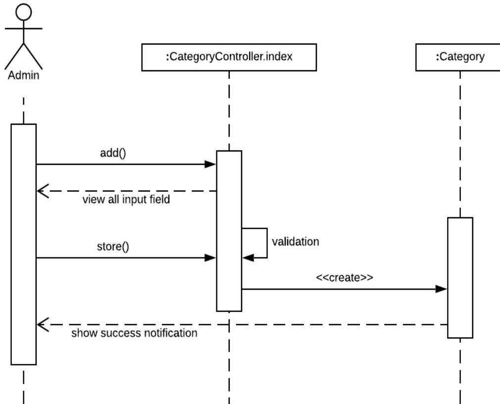
Figure 3.6.16: Sequence diagram for add category
