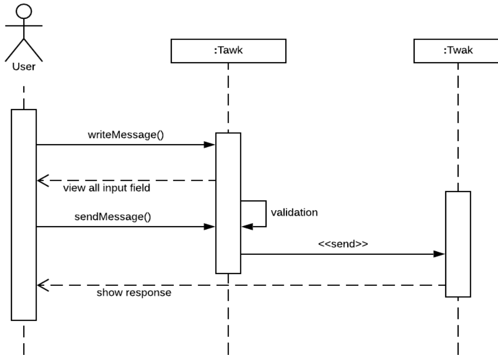
Figure 3.6.7: Sequence diagram for live chat
