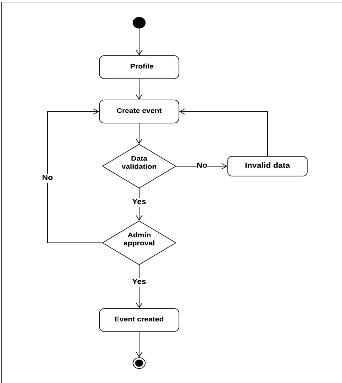
Figure 3.5.7: Create event activity diagram
