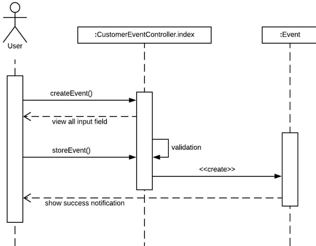
Figure 3.6.6: Sequence diagram for create event
