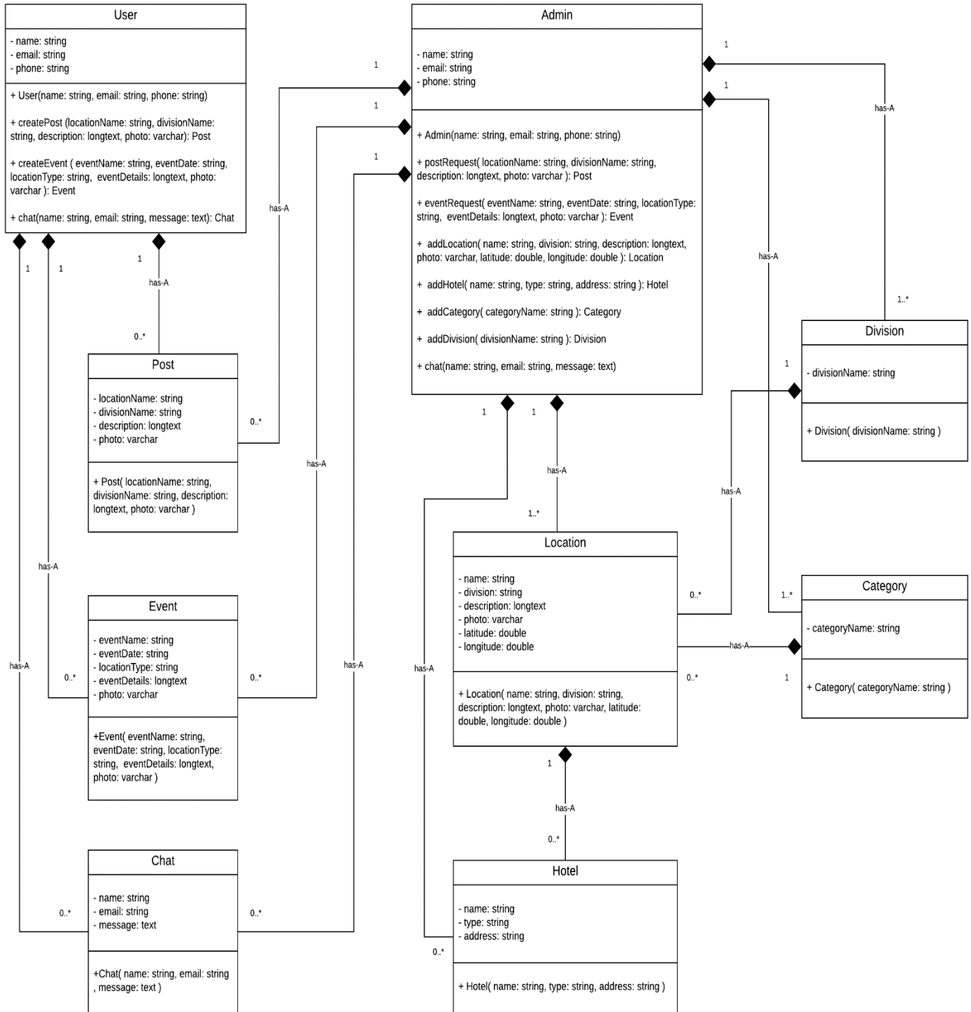
Figure 4.8: Class diagram
