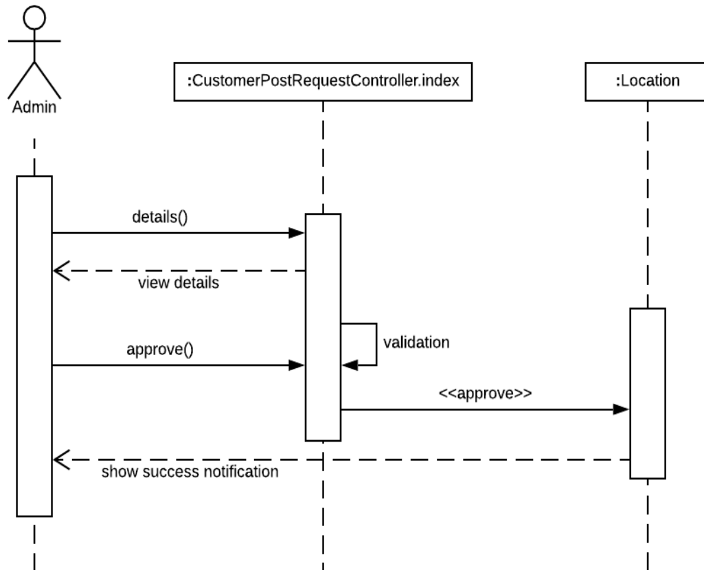
Figure 3.6.19: Sequence diagram for manage post request
