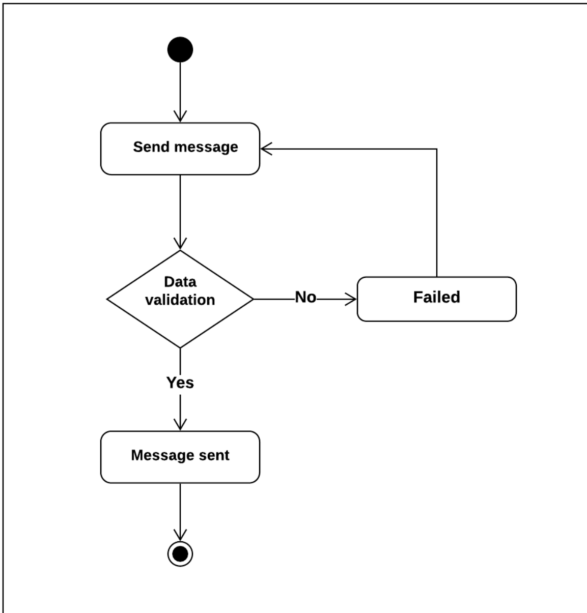
Figure 3.5.23: Live chat activity diagram
