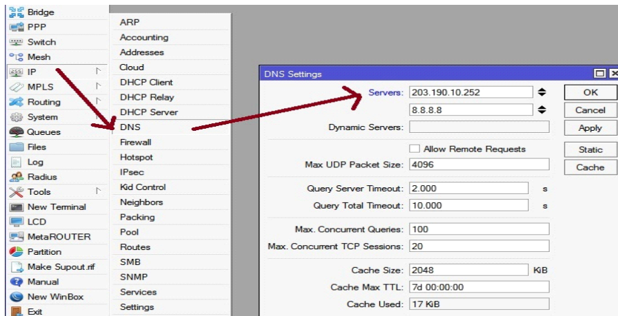
Fig. 3.8: Shows IP DNS setting Criteria
