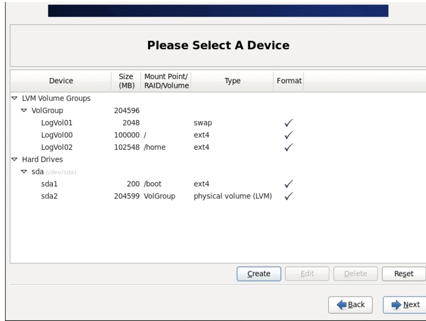
Fig 3.21: Screen Display Screen Print Partition diagram
