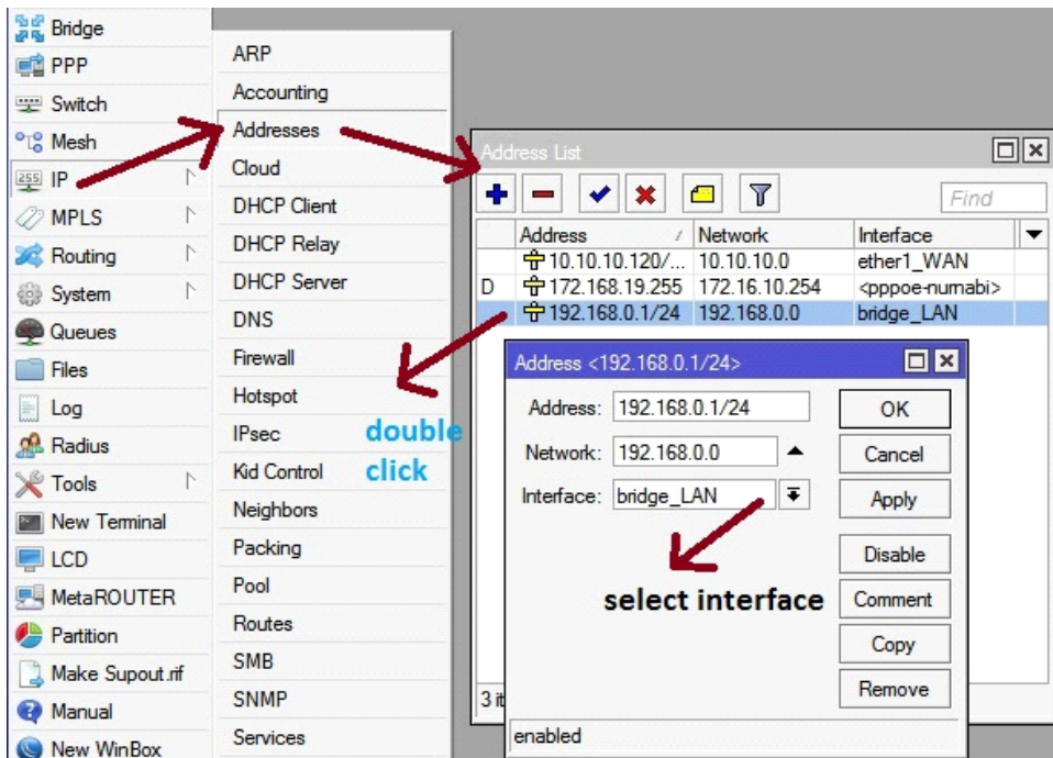
Fig. 3.17: Shows Screen Print create of BRIDGE process (3) diagram
