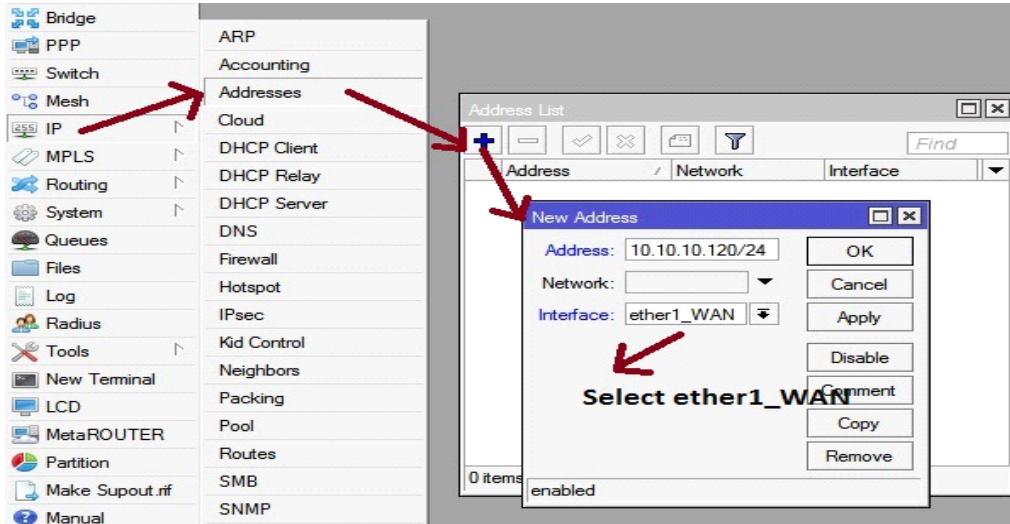
Fig. 3.5: Screen printed IP address shows WAN Port configure
