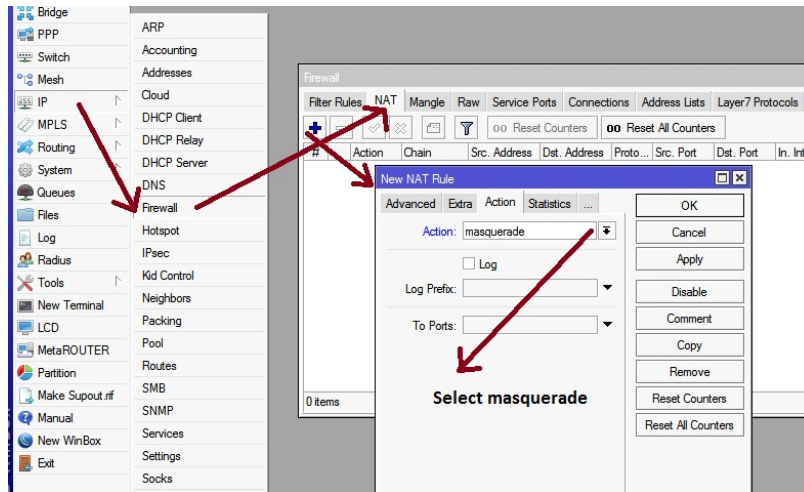
Fig. 3.9: Shows the NAT finishing display window
