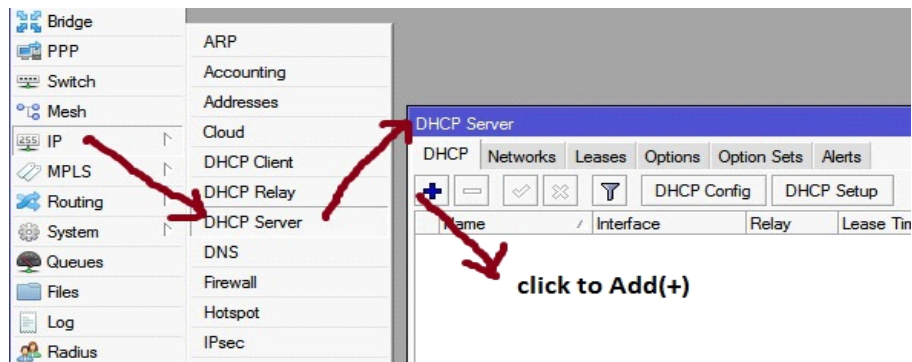
Fig. 3.12: Screen print setup display DHCP configure
