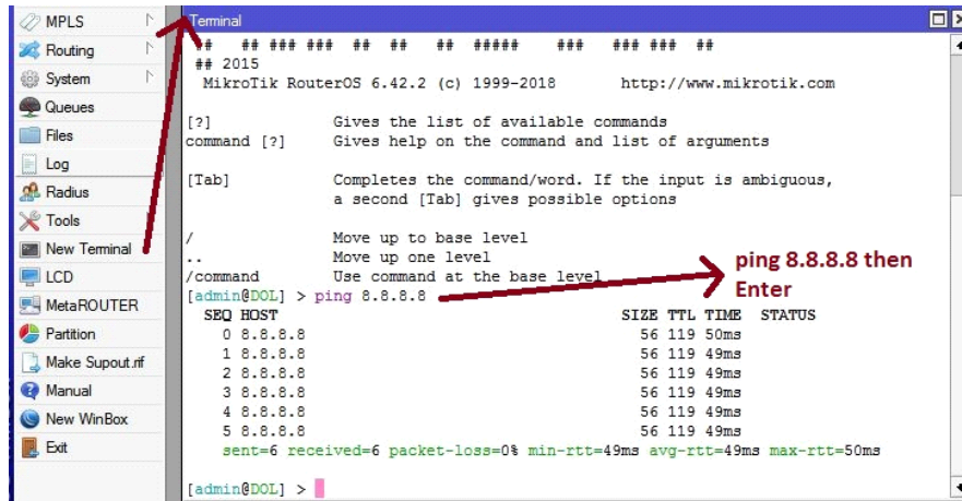
Fig. 3.10: Showing Ping end display
