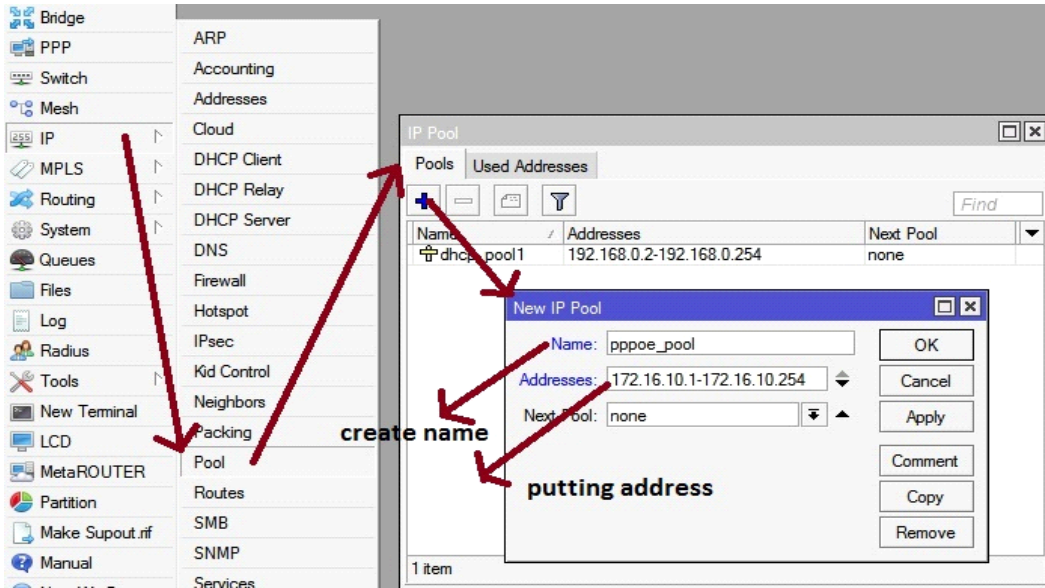
Fig. 3.14: Screen creation shows PPPOE diagram
