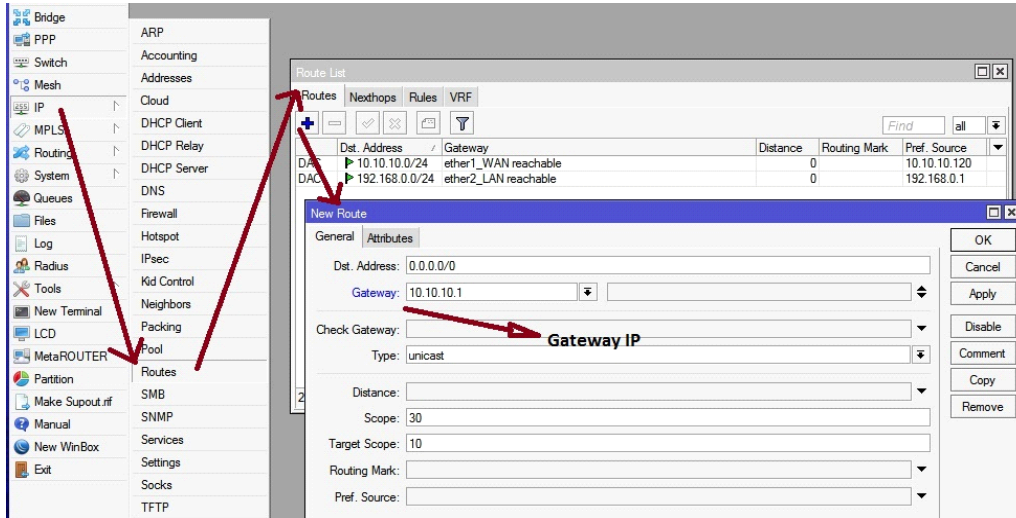
Fig. 3.7: showing up the design of screen Print Gateway connection
