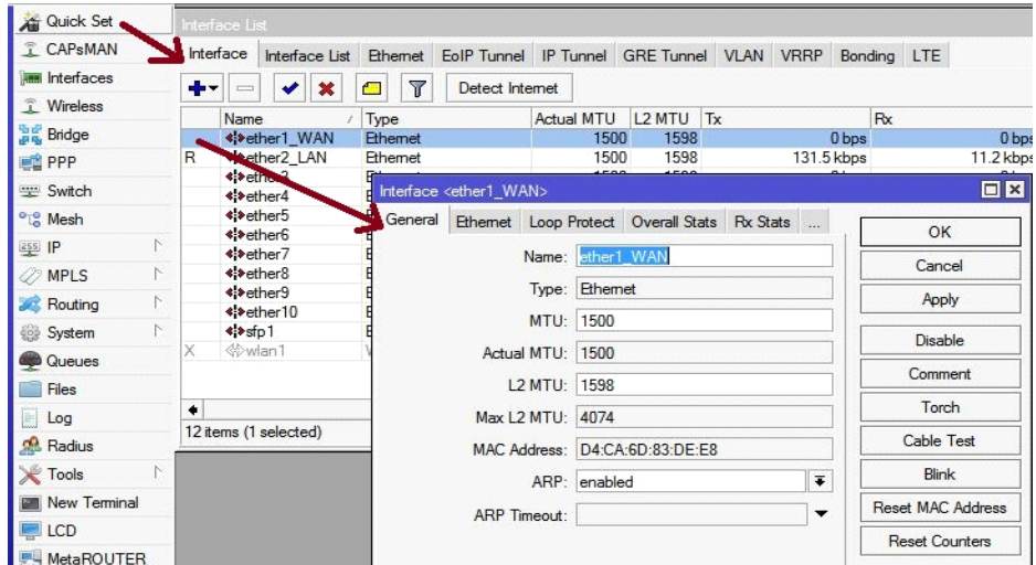
Fig. 3.3: Shows the WAN screen print port No
