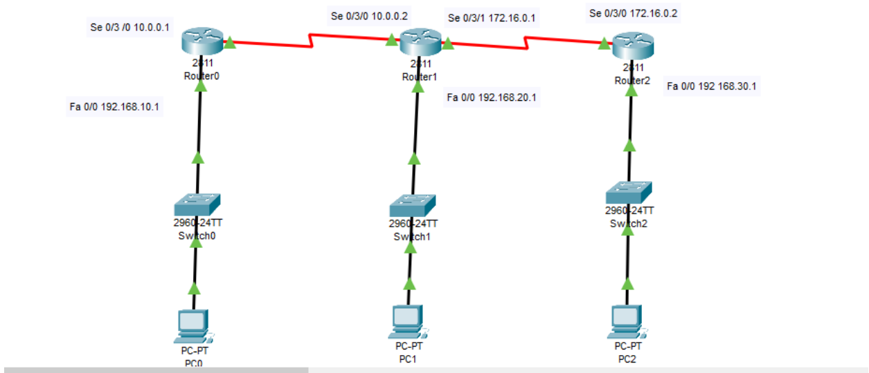
Figure 4.4 : EIGRP
