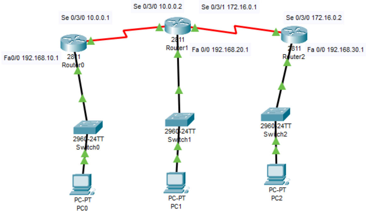
Figure 4.2: RIP V-1
