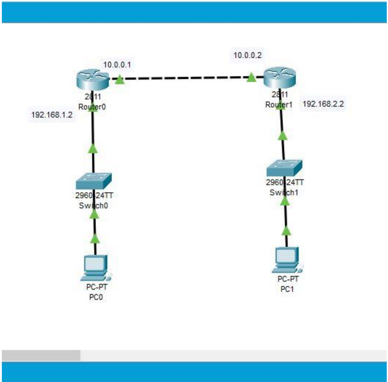
Figure 4.6:Default Routing
