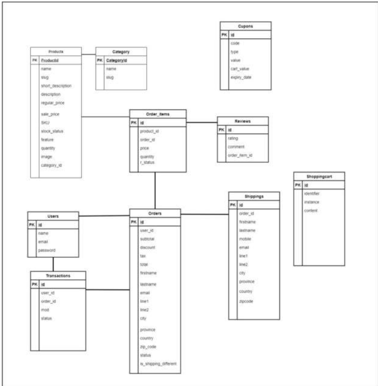
Figure 6.3.7: Database Diagram
