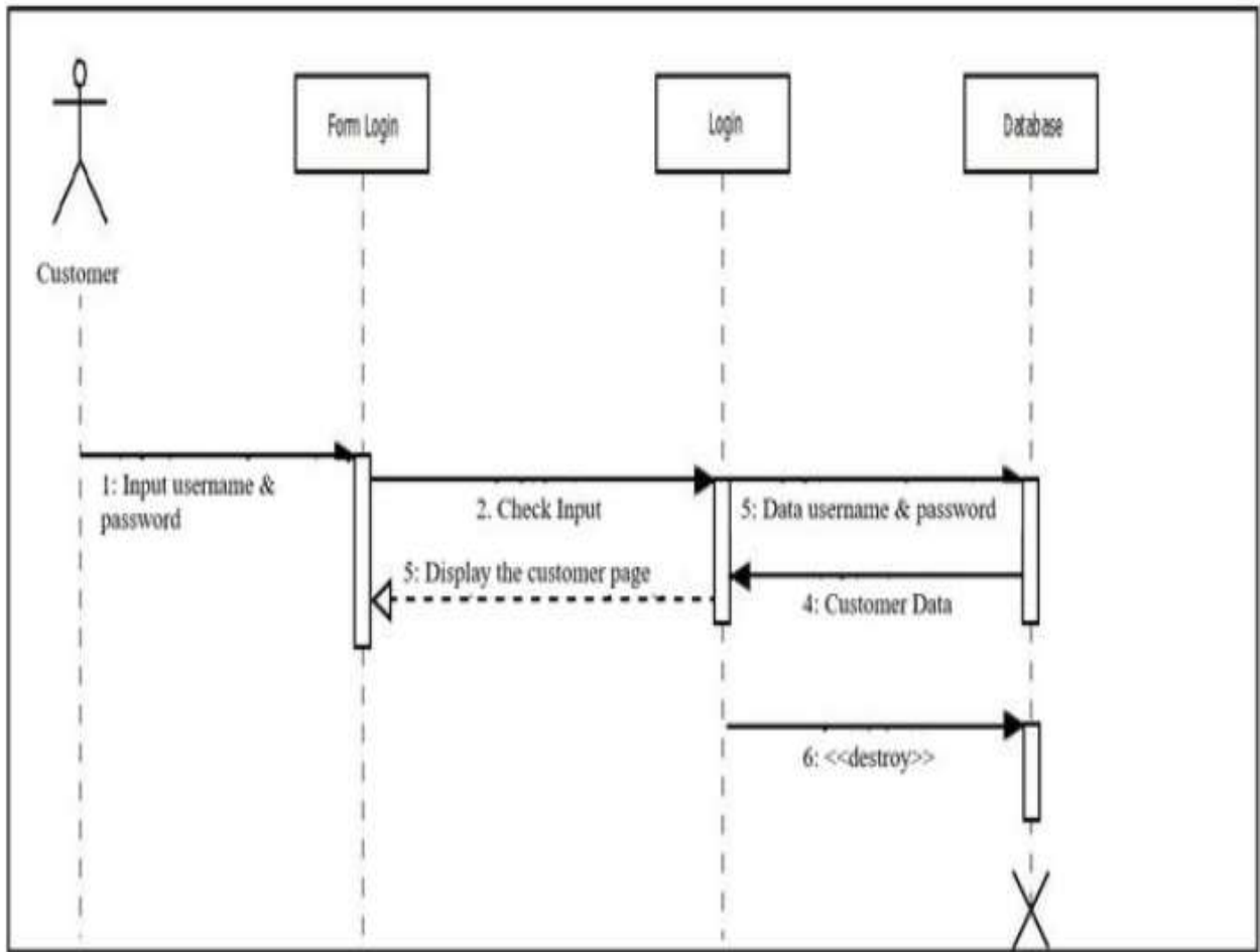
Figure 6.3.5: Sequence Diagram for Login
