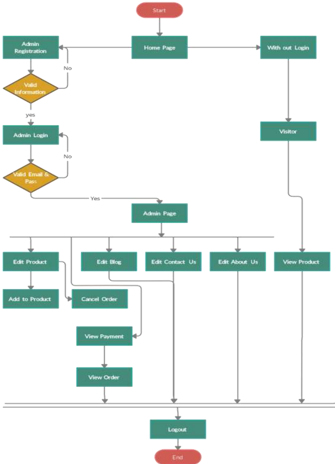
Figure 6.3.3: Activity Diagram for Admin
