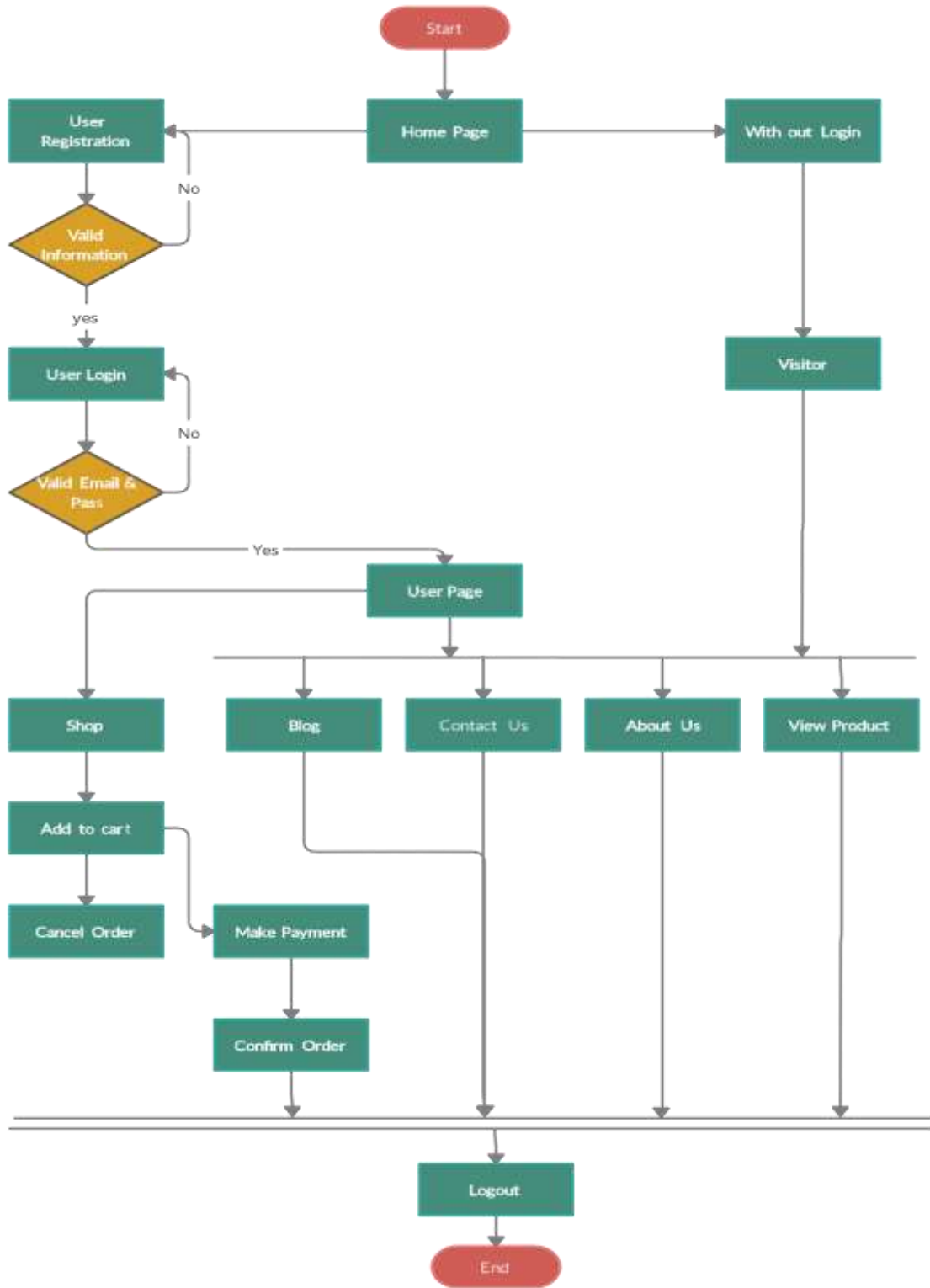
Figure 6.3.2: Activity Diagram for Customer
