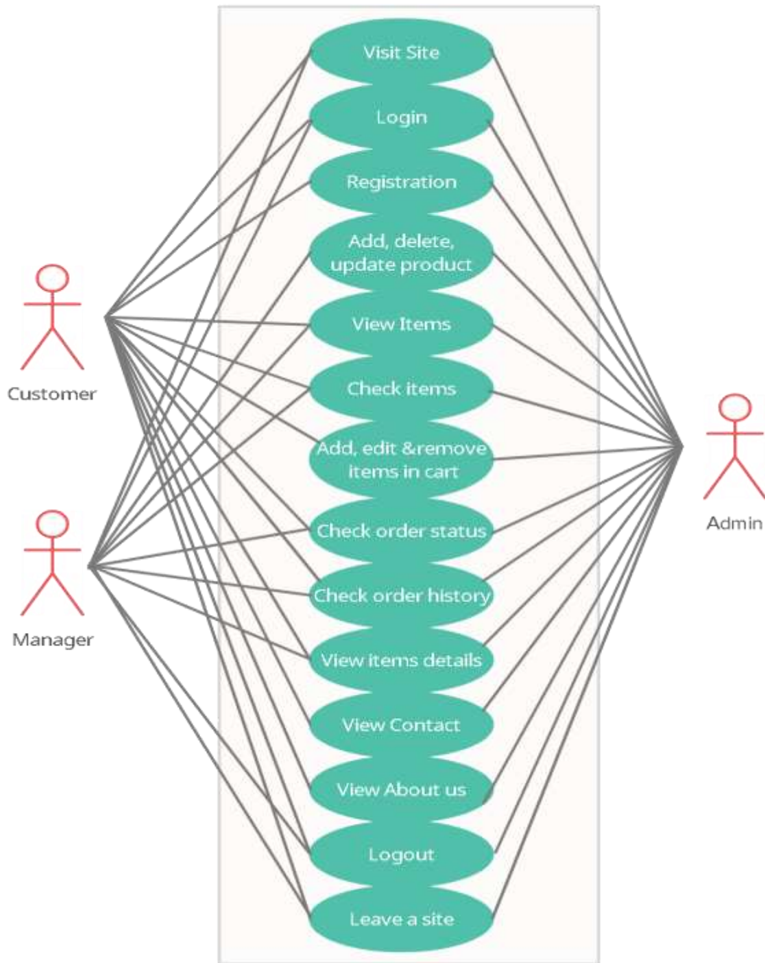
Figure 6.3.1: Use Case Diagram
