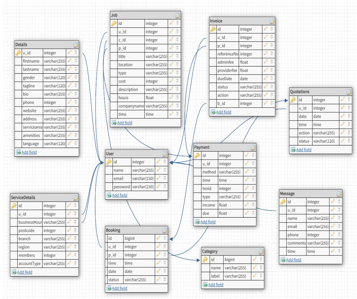
Figure 3.4.1: Logical Data Model
