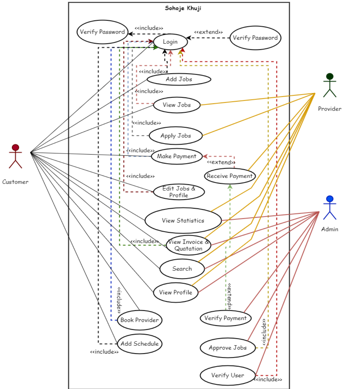
Figure 3.3.1: Use Case Modeling
