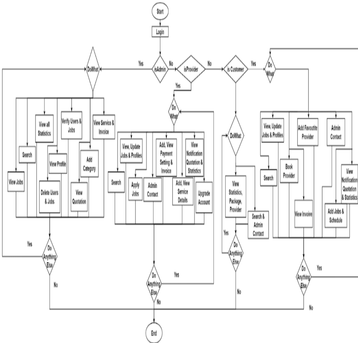
Figure 3.2.2: Flow Chart
