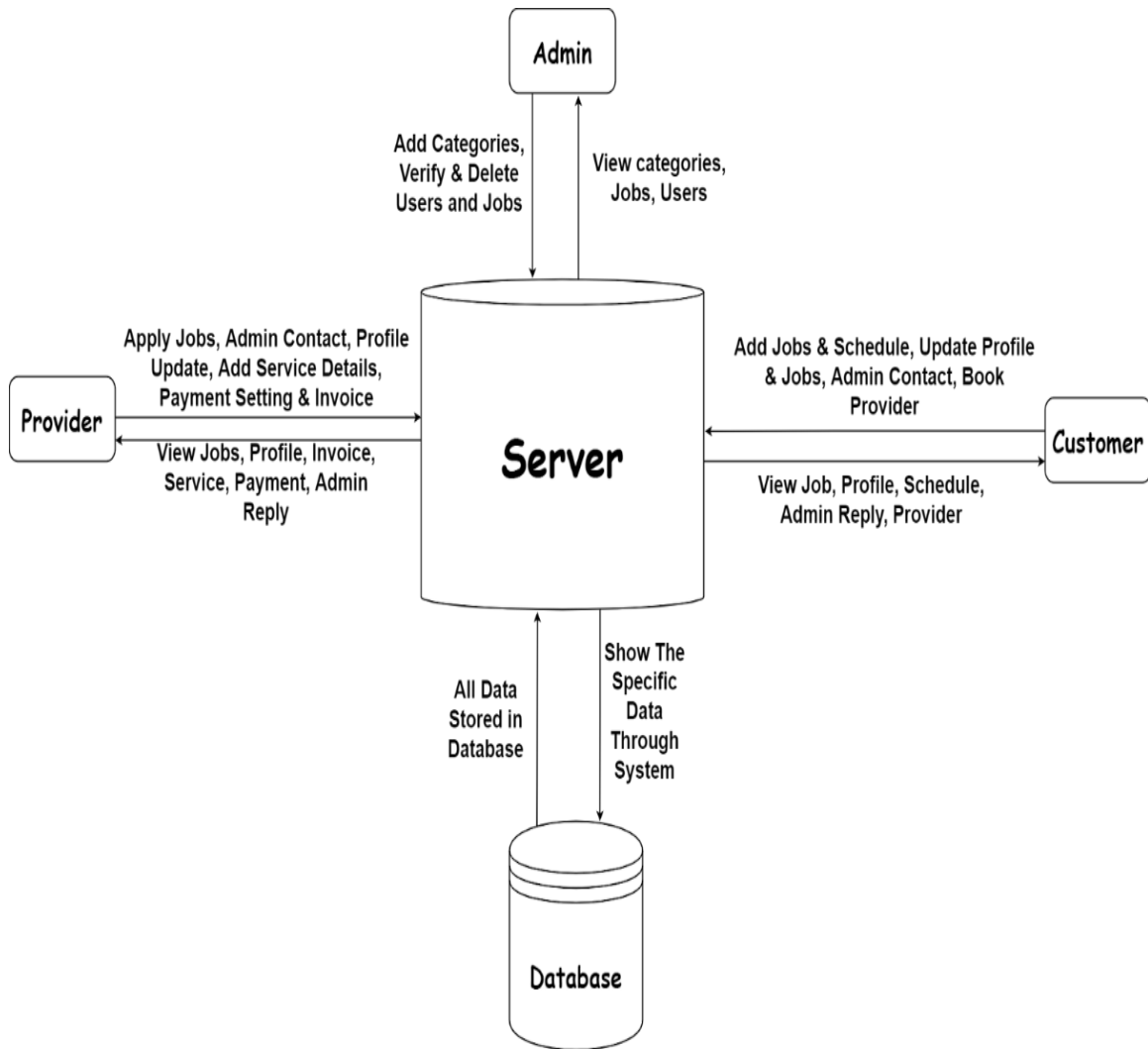
Figure 3.2.3: Data Flow Diagram
