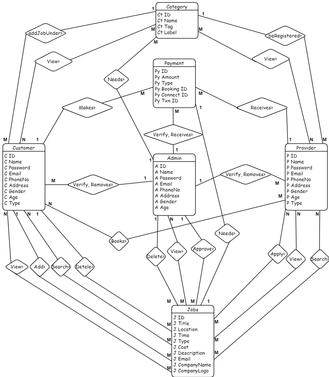
Figure 3.2.4: Entity Relationship Diagram
