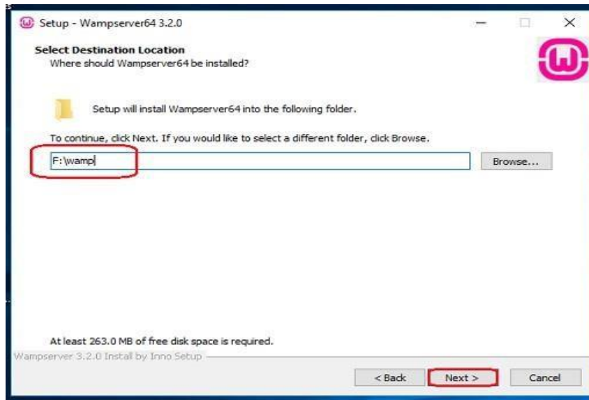
Figure 3.4.5: Select folder.
