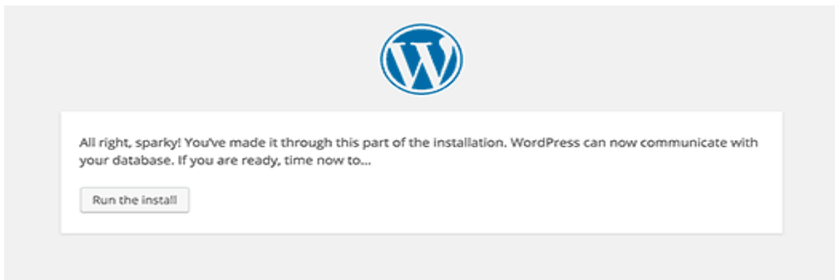
Figure 3.5.9: WordPress Ran
