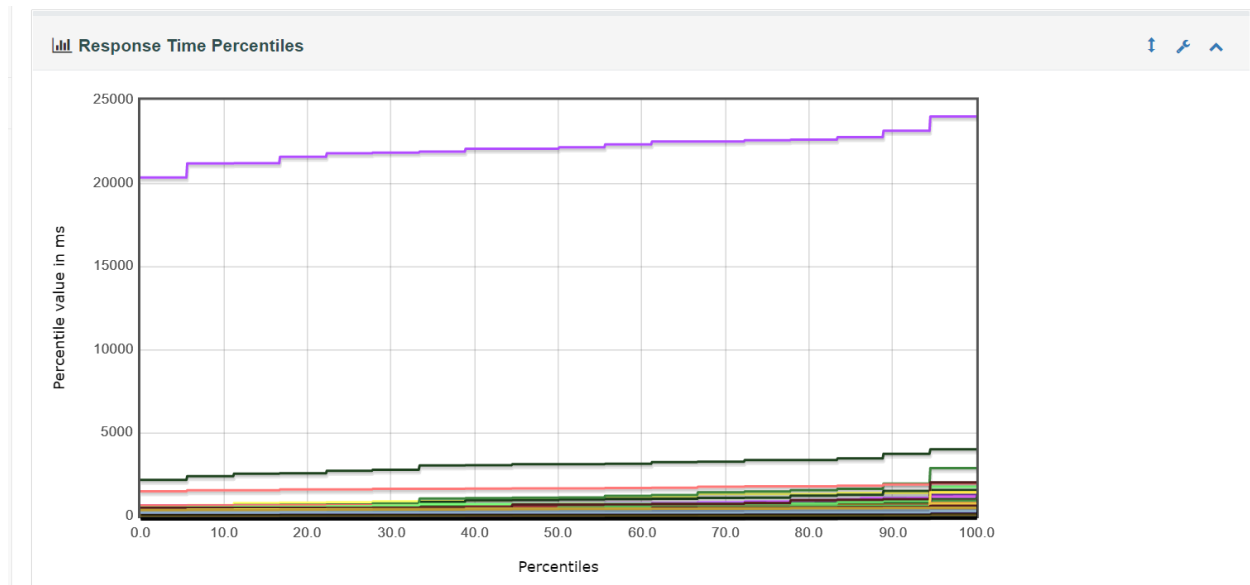
Fig 72: Response time
