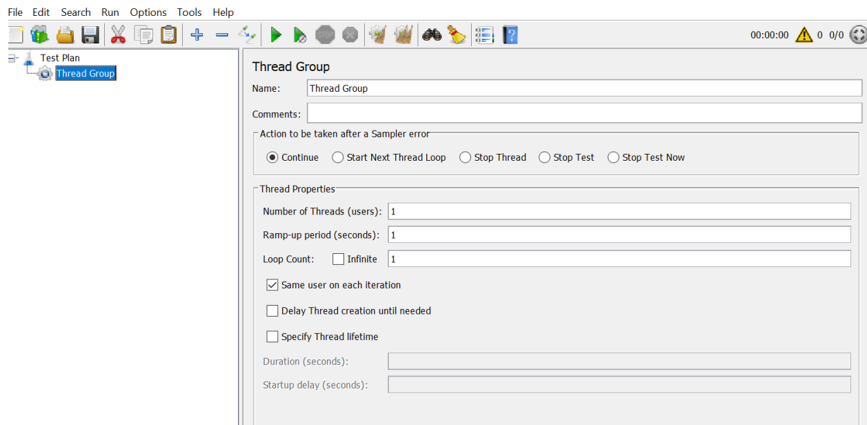
Fig 55: Thread Group
