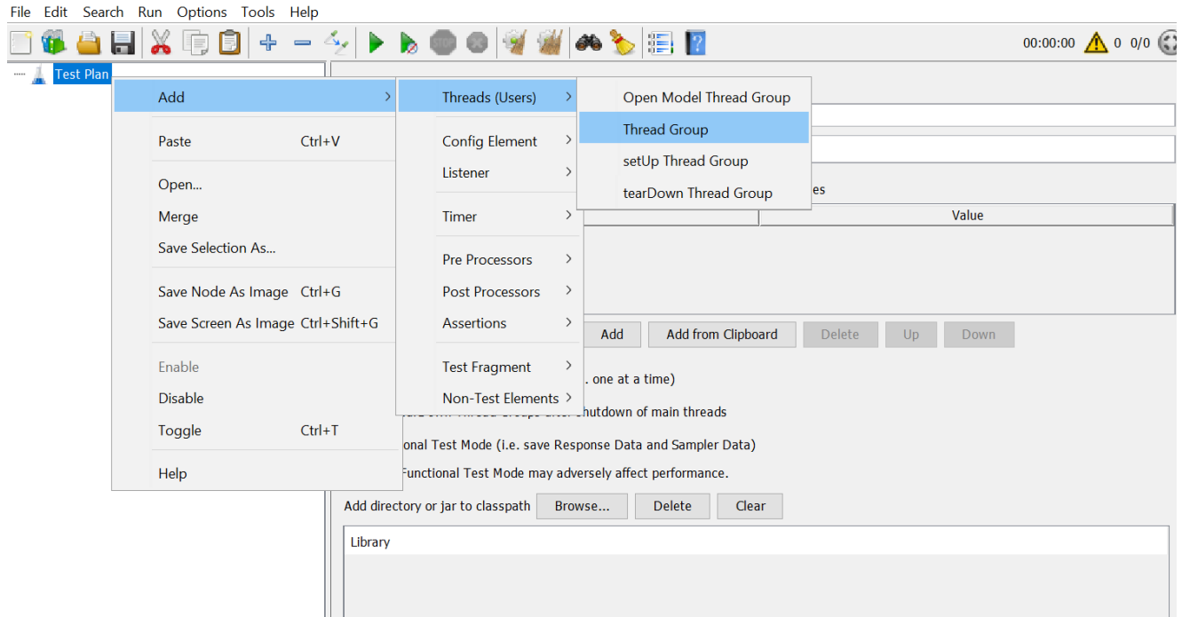
Fig 54: thread group
