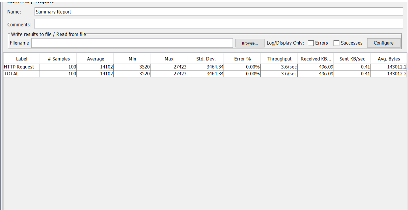
Fig 63: Summary
