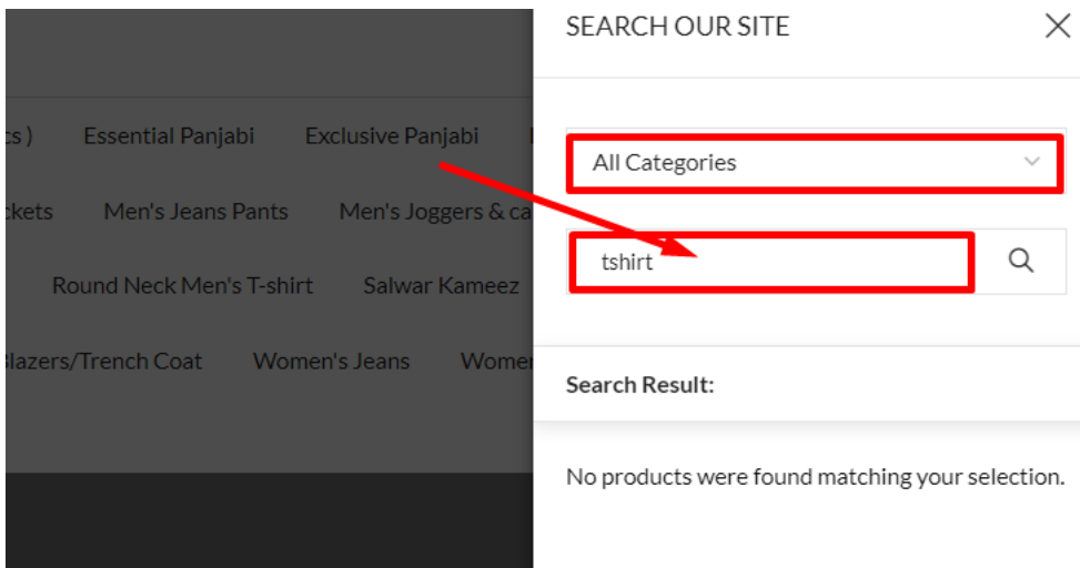
Fig 19: Search TC 003
