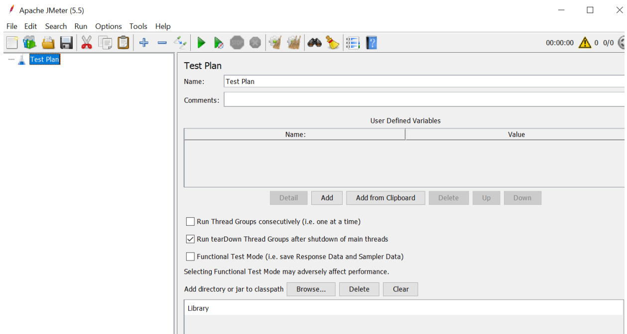
Fig 53: Apache
