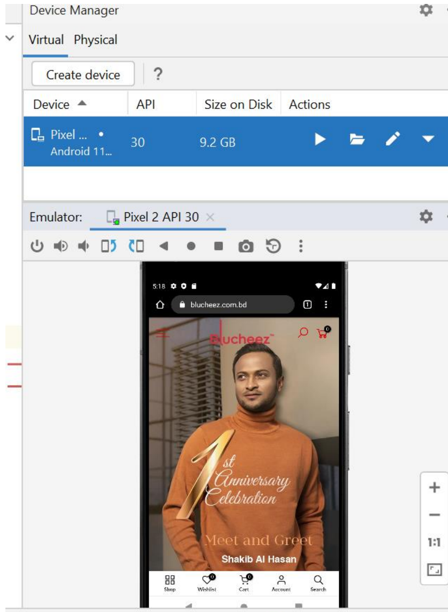
Fig 51: Mobiletest
