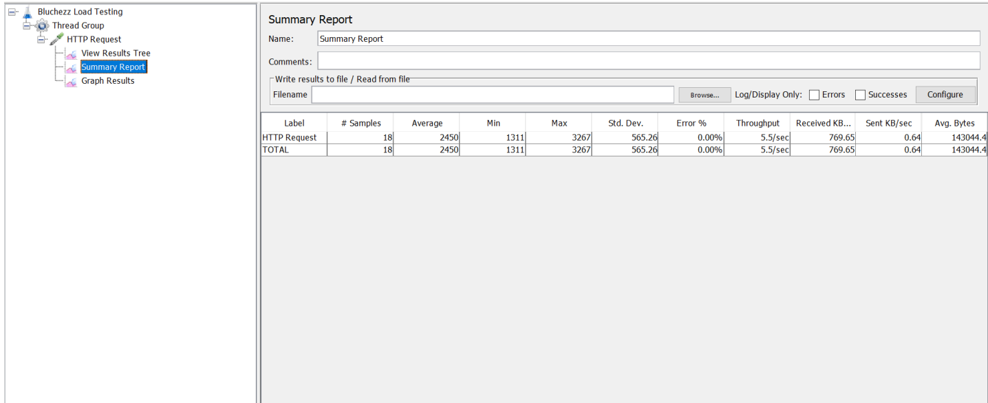
Fig 60: Summary result
