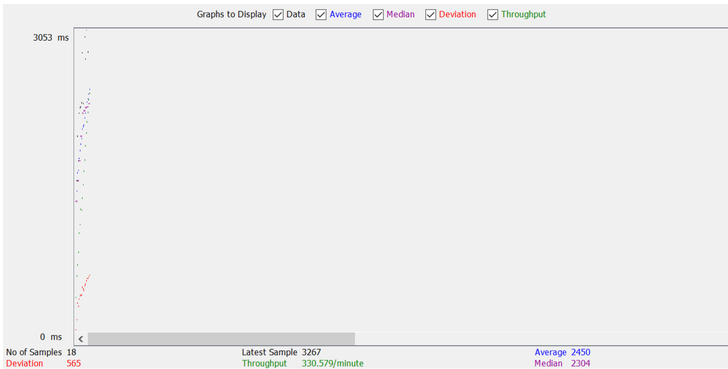
Fig 61: Graph Result
