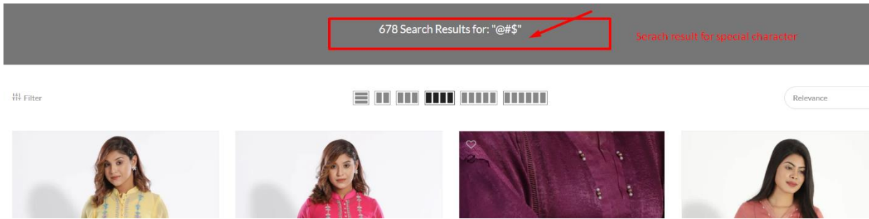
Fig 18: Search TC 001
