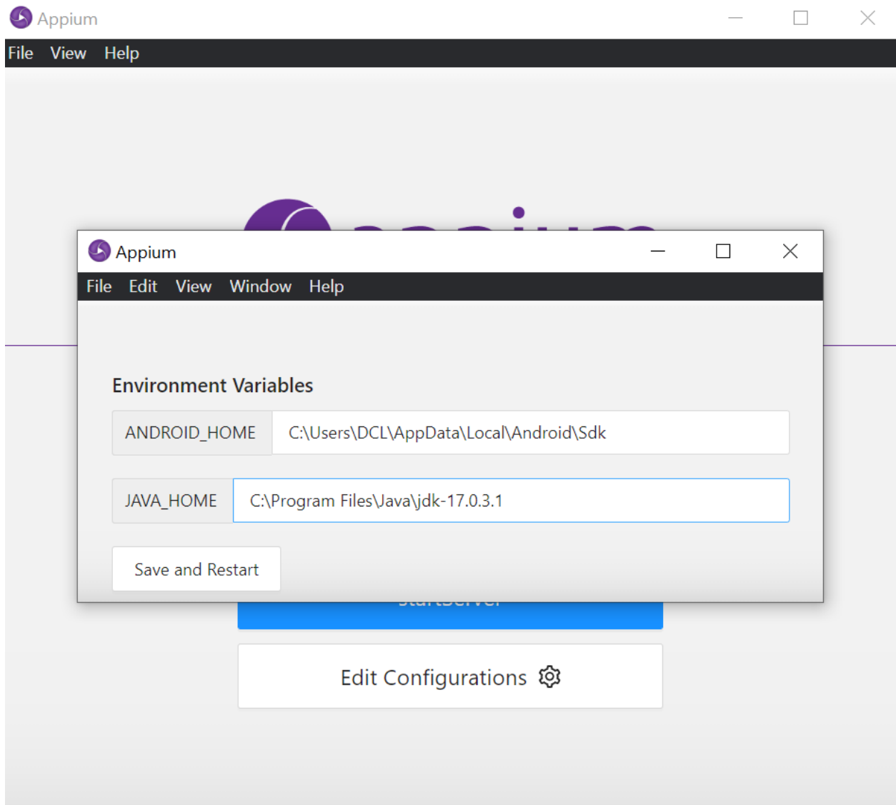
Fig 49: Setting Environment
