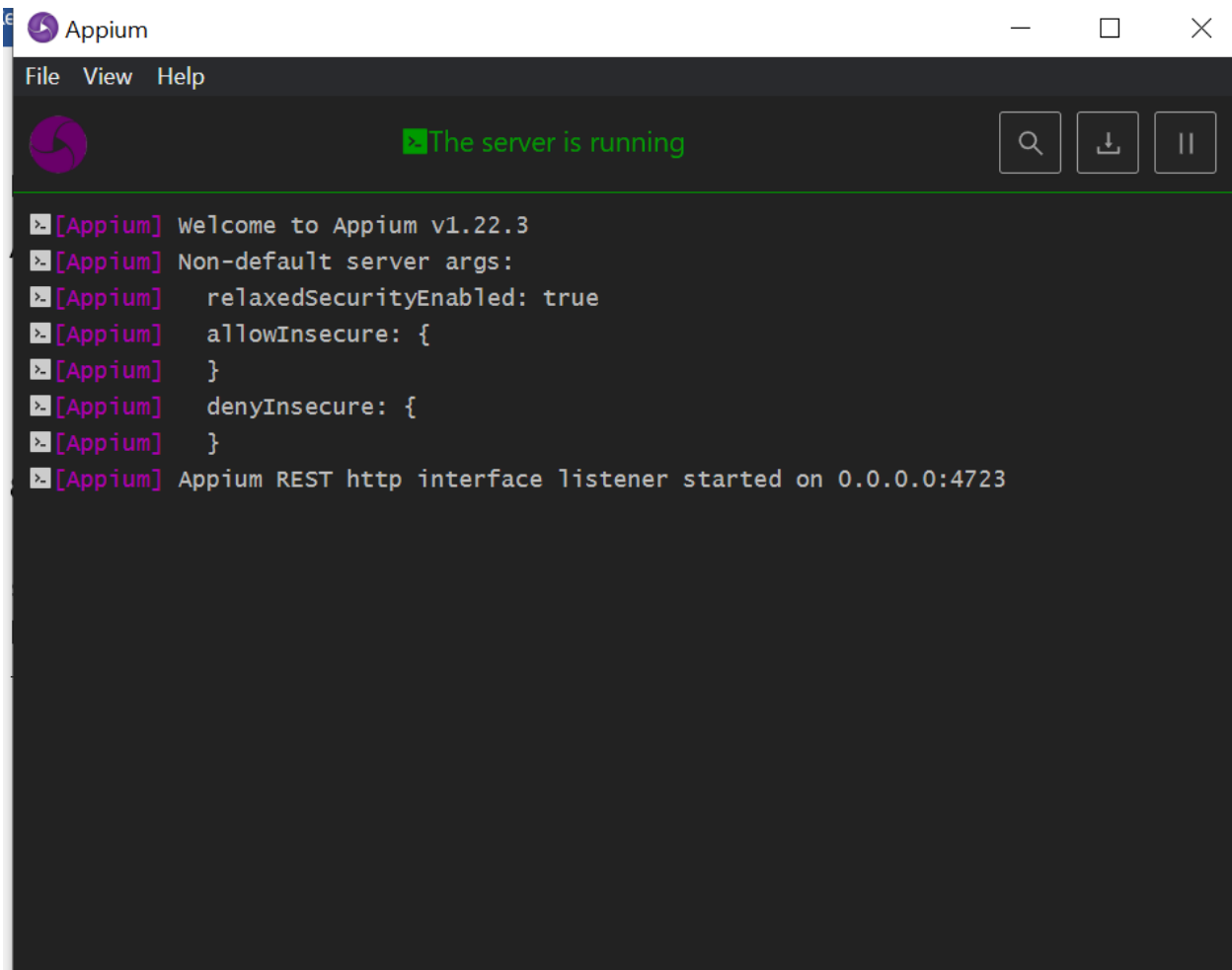
Fig 50: Appium running
