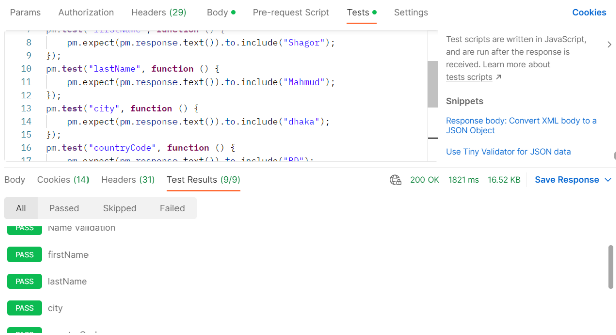
Fig 69: Checkout
