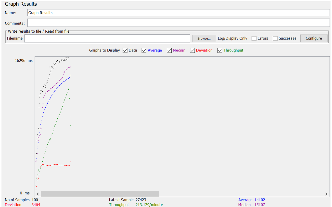
Fig 64: Graph Result
