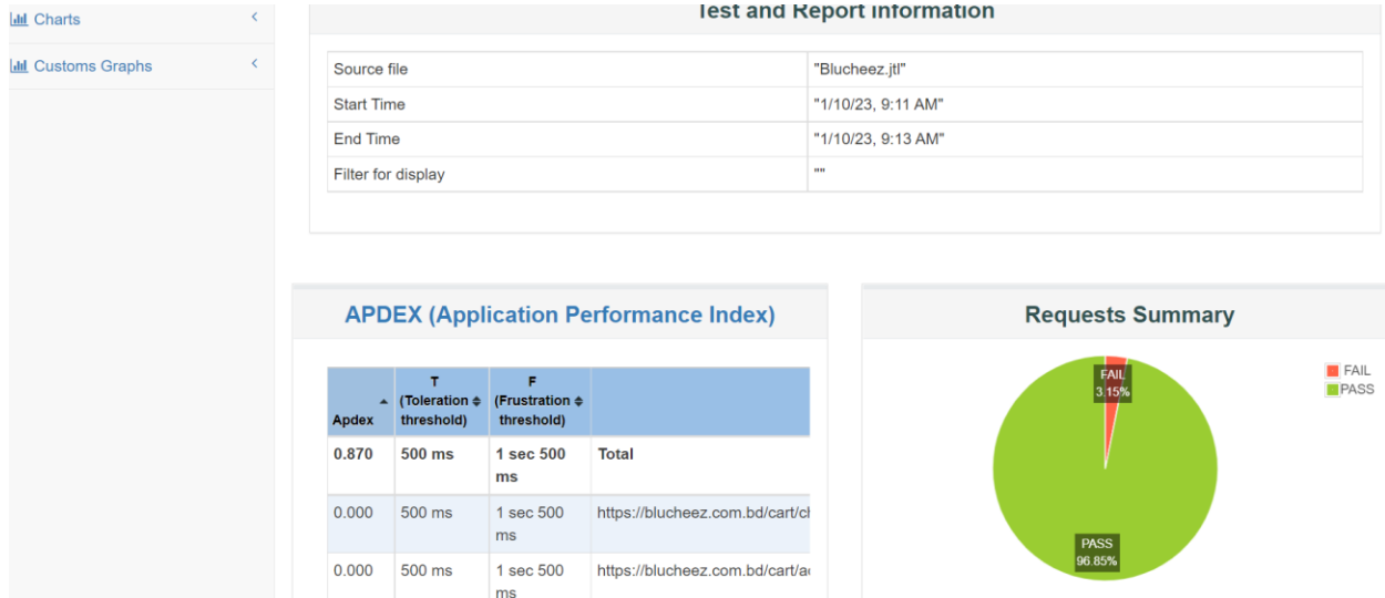
Fig 71: Summary
