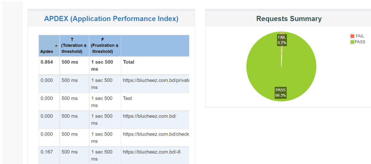
Fig 74: Summary
