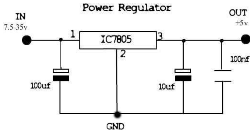
FIG 3.1 VOLTAGE REGULATOR CIRCUIT DIAGRAM
