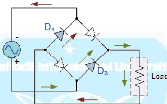
Fig 4.4 (Negative Half-cycle)
