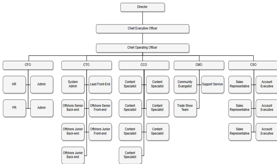
Fig 2.5.1: Organization Structure
