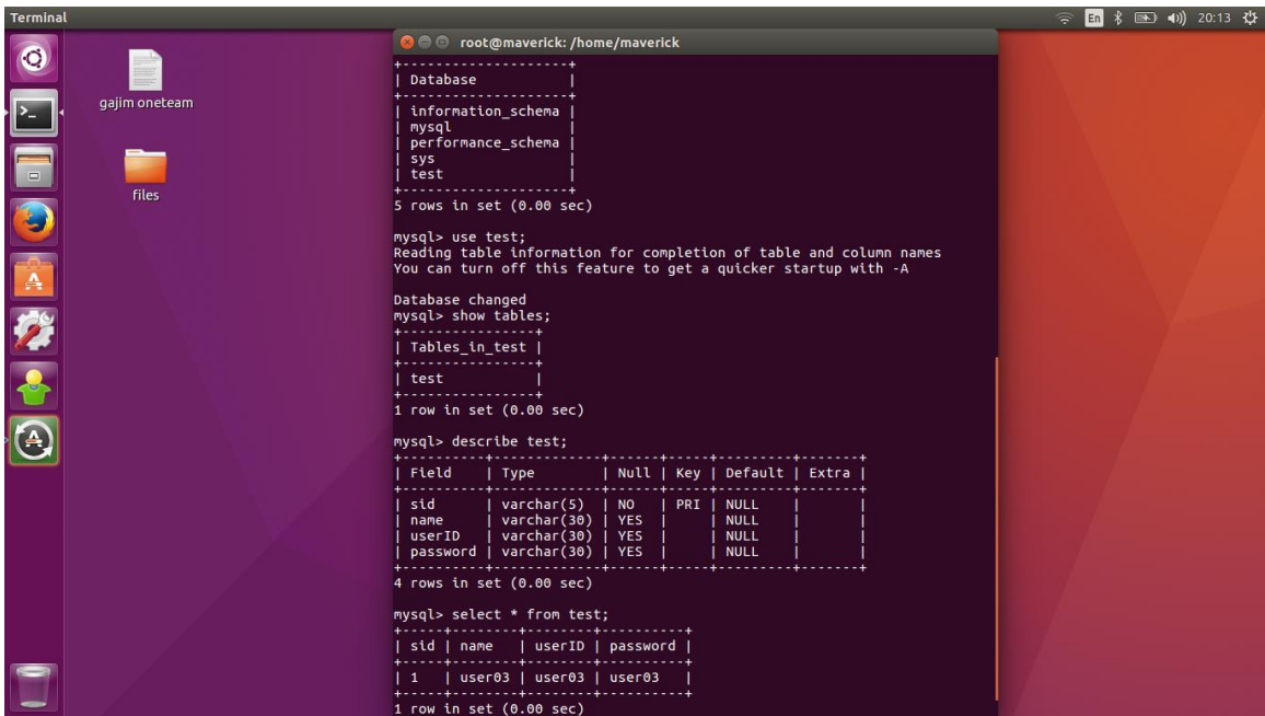
Fig 3.3: Database Management
