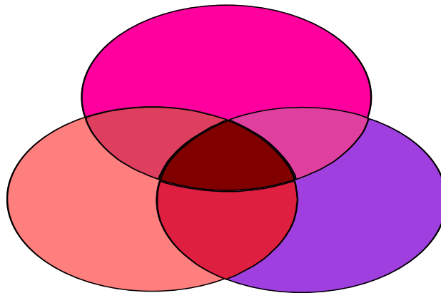
Figure 14: Handover Problem
