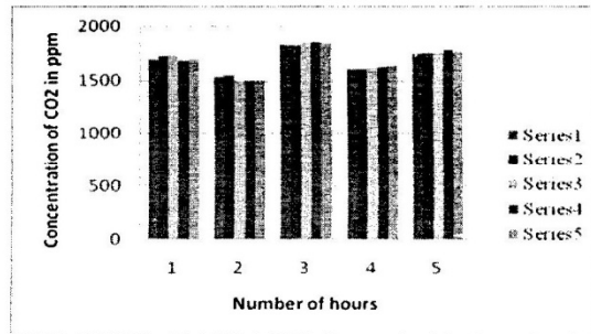
Fig. 2: Average Hourly Concentration of CO 2 in Sango Ota, Ogun State, Nigeria
