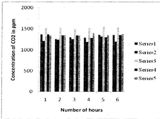
Fig. 1: Average Hourly Concentration of CO 2 in Abeokuta, Ogun State, Nigeria
